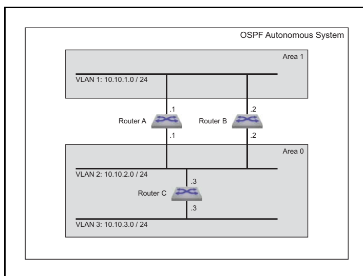
Figure 26-3 OSPFv2 Example 1
