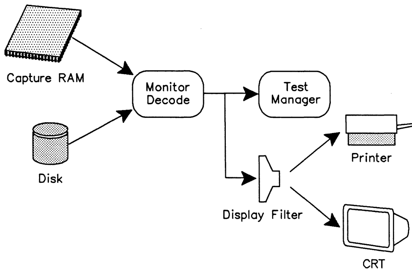
Figure 3-2 SNA Monitor Data Flow Diagram – Offline Processing
