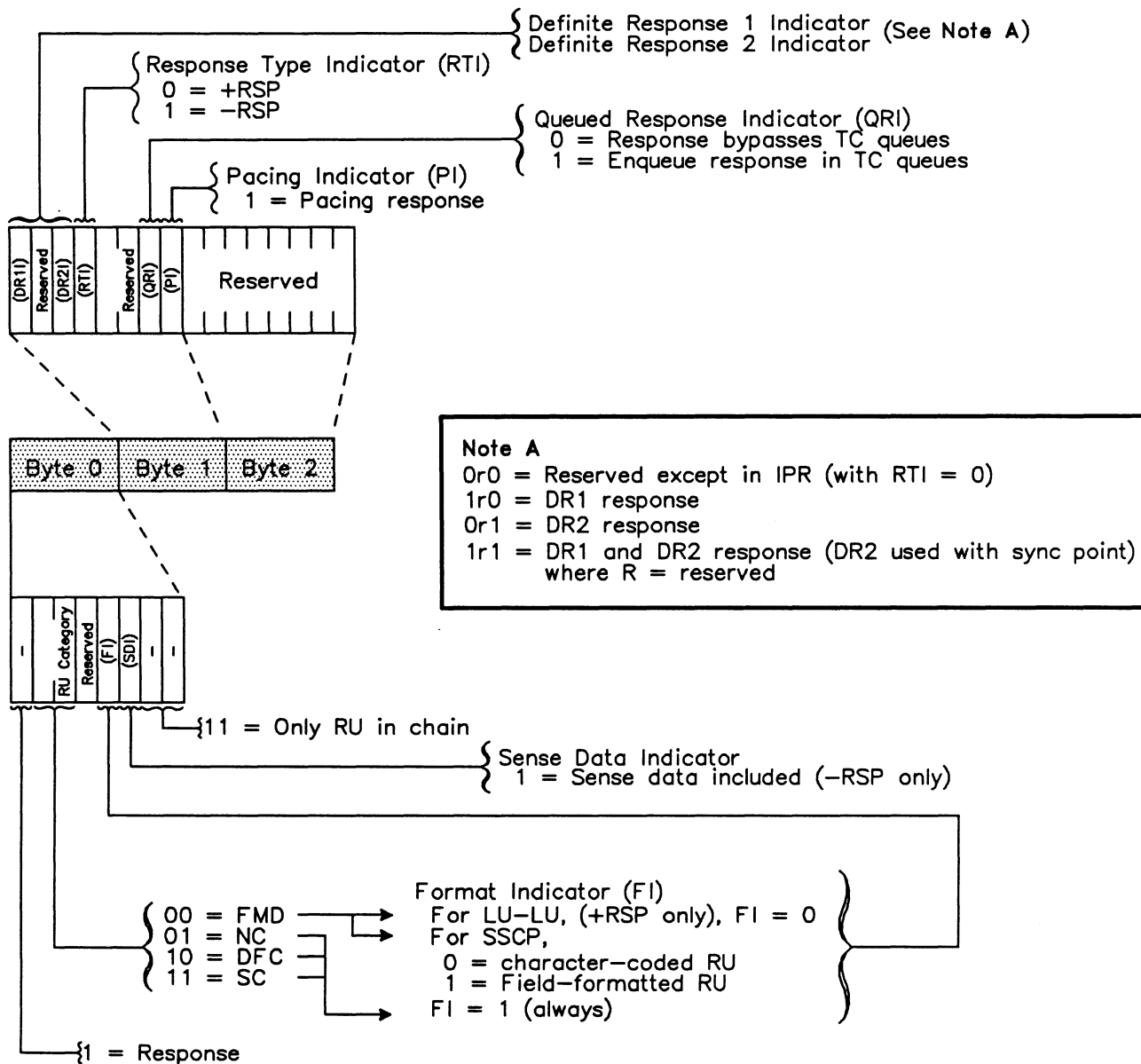
Figure A-15 Response Header
