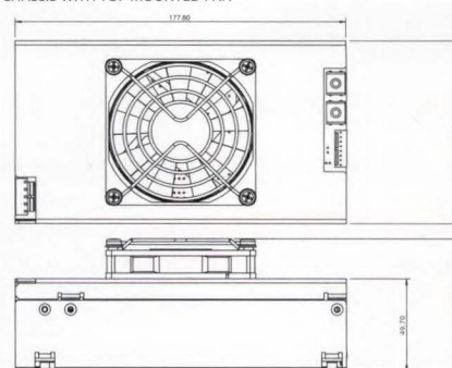
CHASSIS WITH TOP MOUNTED FAN
