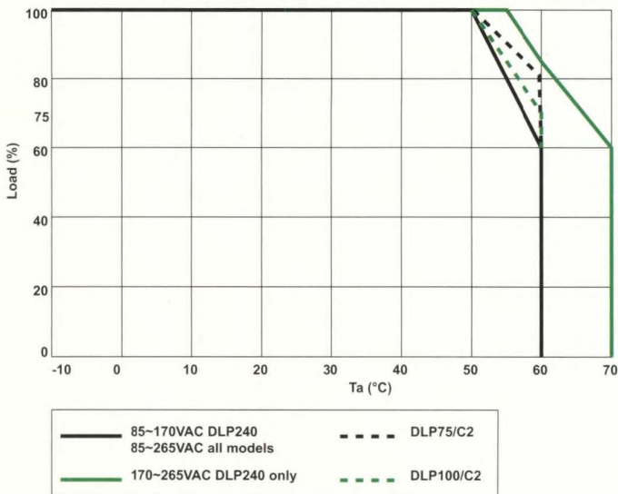
Derating Curve
