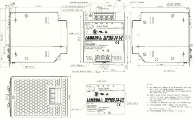
DLP180 Outline
