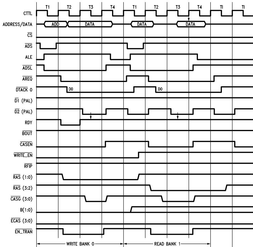
Design # 1: 32332 with No Wait States (No MMU, PAL Input 1W Tied High)
