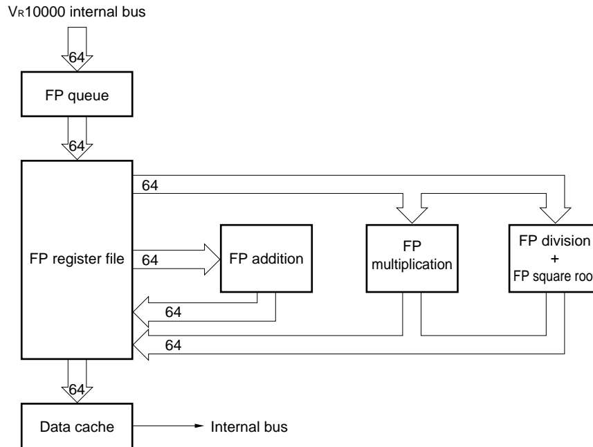
Figure 3-1. Internal Block of FPU
