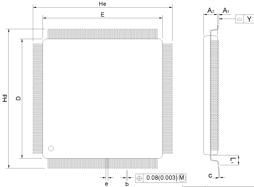
Figure 7-1 208-Pin Plastic Quad Flat Package (PQFP)
