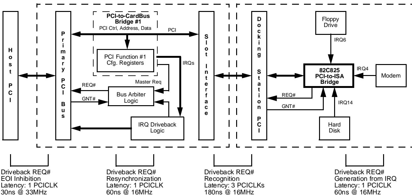
Figure 4-2 Worst IRQ Driveback Latency Example
