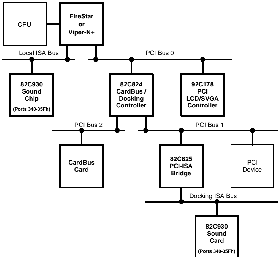
Figure 1-1 Multiple ISA Bus Support
