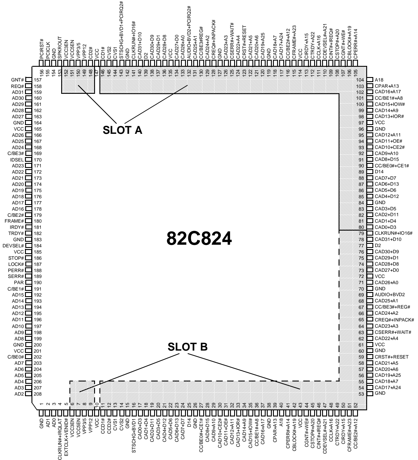
Figure 3-1 Pin Diagram
