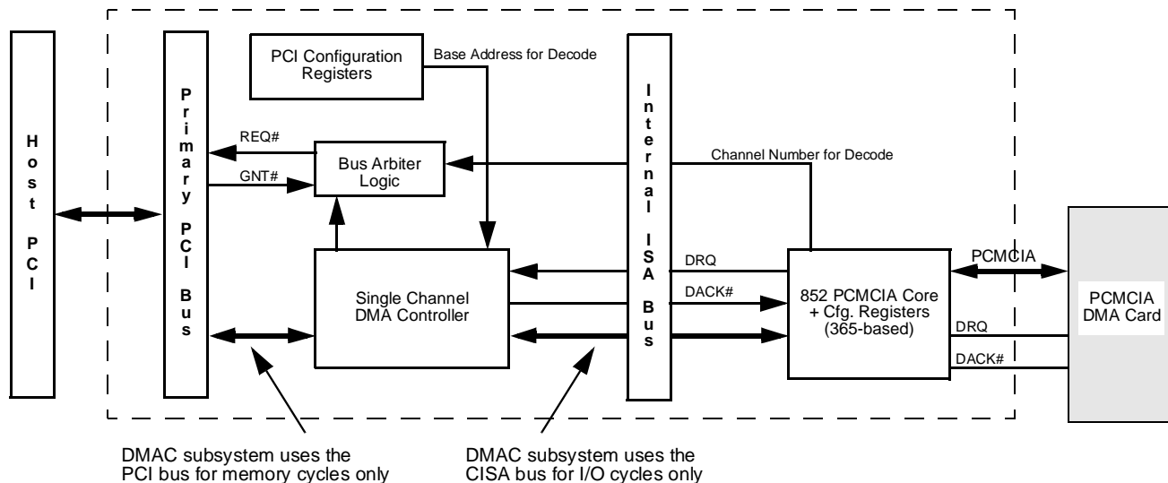
Figure 4-3 DMA Controller Subsystem Logic
