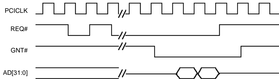
Figure B-1 IRQ Driveback Cycle High-Priority Request
