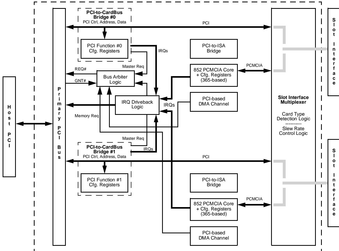
Figure 4-1 82C824 Organization
