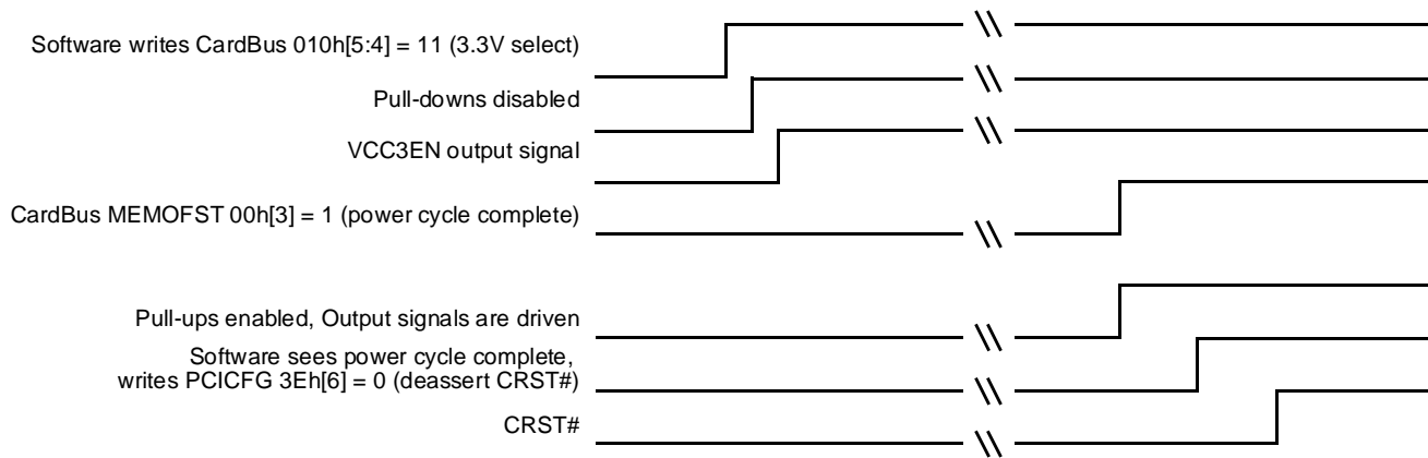
Figure 3-2 Power-Up Timing Example
