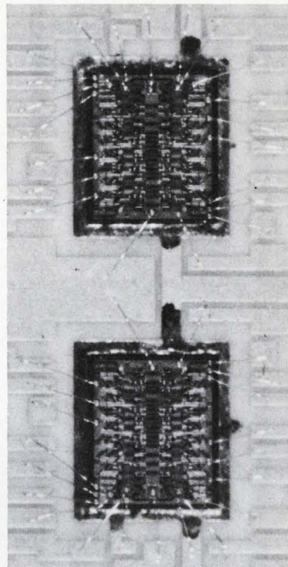
Complex digital circuits, such as this 104-gate, 32-bit ECL active element memory from Texas Instruments, will be discussed in Wescon paper 20/2.
