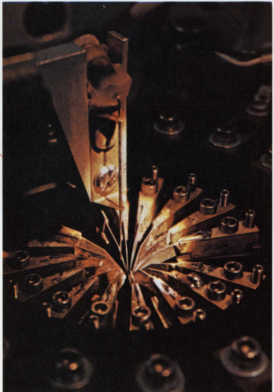
A complex array for dc and functional testing is probe-tested on the production line at Fairchild Camera and Instrument Corp.
