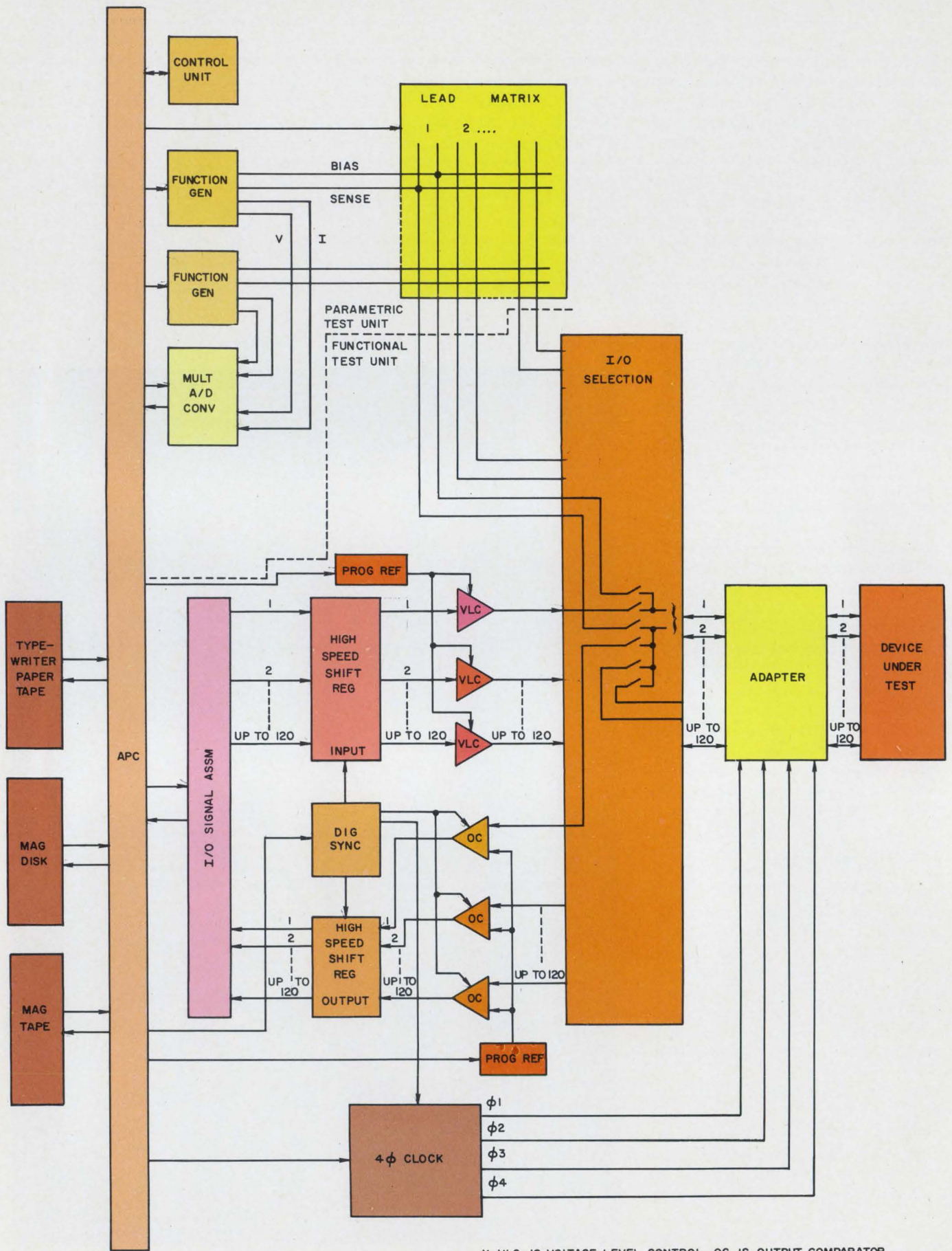
LSI tester can test up to 120 MOS leads at a 2-MHz rate. It's Texas Instruments' Model 561.
