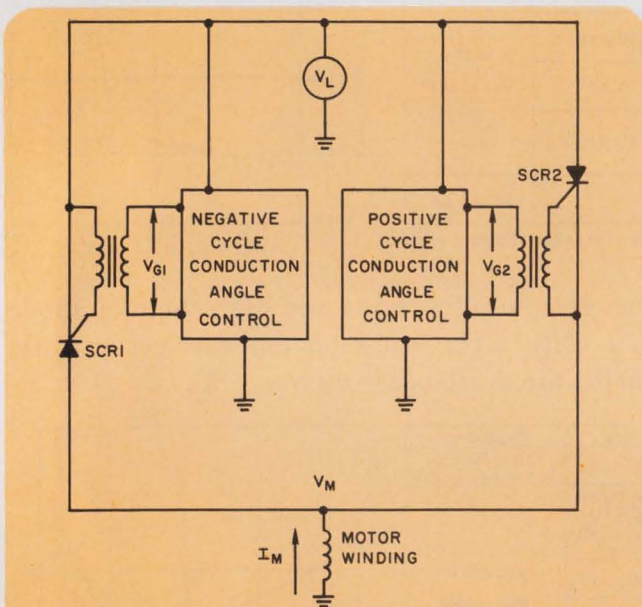
1. Because current I_M lags applied voltage V_L , SCR1 does not turn off and allow SCR2 to turn on when V_L goes through zero.
