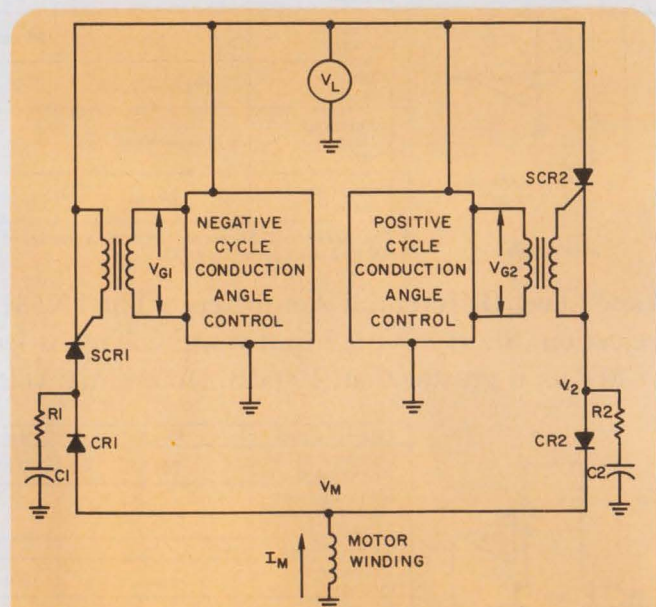
2. With the addition of CR2 , R_2 and C_2 , SCR2 can turn on when it receives its trigger pulse, even though SCR1 has not yet turned off.
