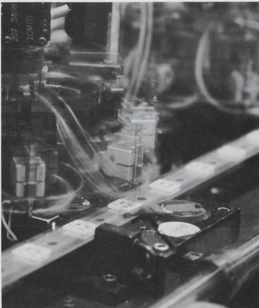
Chip transistors and diodes are placed on alumina substrate at IBM's solid logic manufacturing facility, Hopewell Junction, N.Y. (Paper 2/1).
