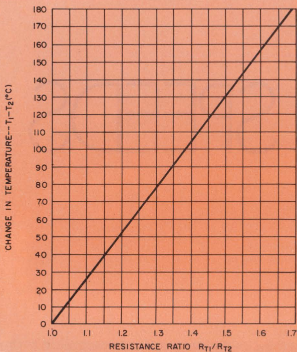
Ratio of primary winding resistances at no load, R_{T2} , and full load, R_{T1} , allows computation of the transformer's internal temperature rise.
