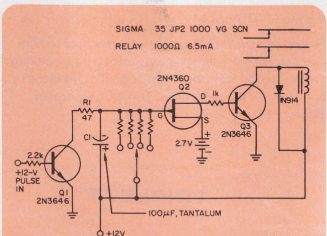
C_1 becomes fully charged each time an input pulse is received, so that Q_3 is forward-biased by FET Q_2 .
