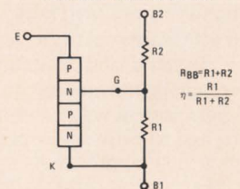
EQUIVALENT CIRCUIT WITH EXTERNAL "PROGRAM" RESISTORS R1 AND R2
