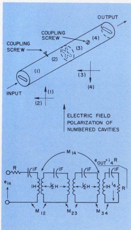
1. Waveguide elliptic-function filter structure has two pairs of screw-coupled cavities that are iris-coupled to each other. The equivalent circuit shows mutual coupling of the input and output cavities.
