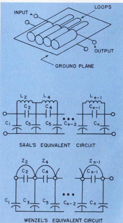
2. Coupled bars and wire loops between a pair of ground planes are the main elements of this compact elliptic-function filter design by R. Wenzel. The equivalent circuit is similar to the classic version by R. Saal.
