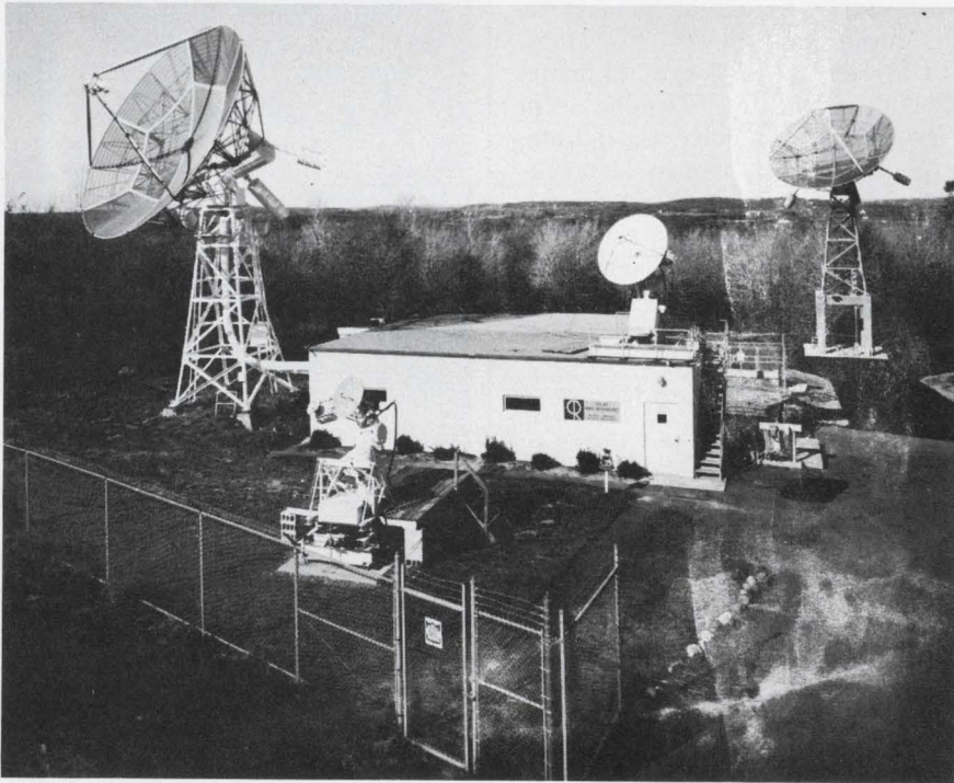
Solar activity is monitored in different frequencies by these five antennas at the Air Force Cambridge Laboratories' solar radio observatory near Ipswich, Mass. From left to right: the 28-foot antenna receives solar emissions at 606 MHz and 1415 MHz; the 1-foot antenna in the foreground attached to its 3-foot companion on the right receives at 35,000 MHz; the 3-foot dish is tuned in at 15,400 MHz; the 8-foot antenna on the observatory roof receives at 2695 MHz, 8800 MHz and 4995 MHz; the 28-foot dish at the right of the building receives at 245 MHz.
