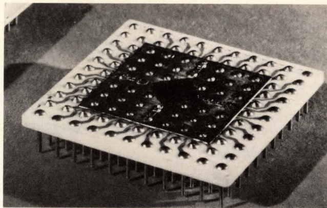
3. Bondage. There are 132 solder dots on the finished logic chip (left). The chip is inverted onto the 116-pin ceramic carrier (above) and the two are heated till the solder reflows and bonds them together, several chip solder connections being linked to the same pin.
