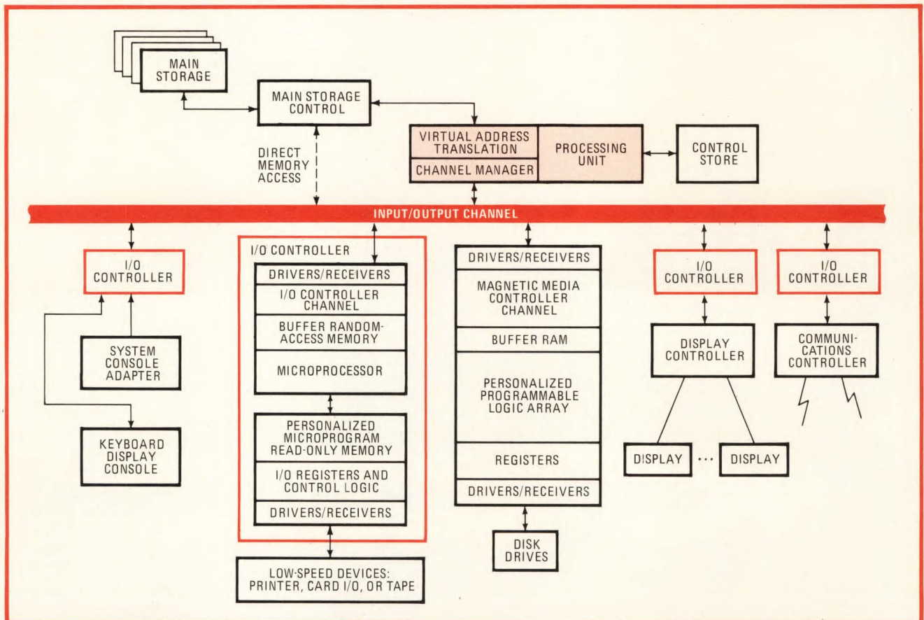
2. Central channel. System/38 hardware centers on an input/output channel that operates at speeds up to 5 megabytes per second. Attached to it are not only the central processing unit but also I/O controllers based on microprocessors or programmable logic arrays.
