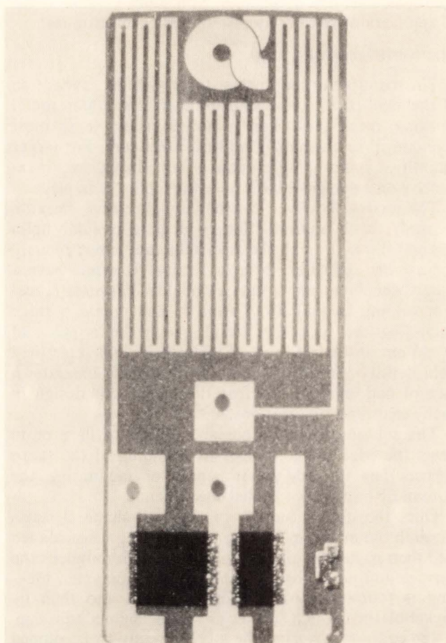
1. Porcelain on steel. The thermal and surface properties of porcelain-coated steel allow modified thick-film inks to be screened and fired onto its surface at a relatively low temperature. A sample, shown above, has screened-on resistors and conductors.
