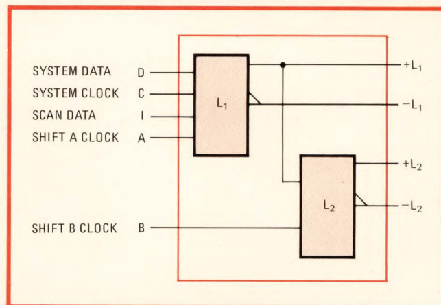
1. Limited memory. Level-Sensitive Scan Design technique restricts the types of memory elements in a design to random-access memories and shift register elements made of paired latches. Latch 1 is both a test and a storage element, latch 2 primarily a testing element.
