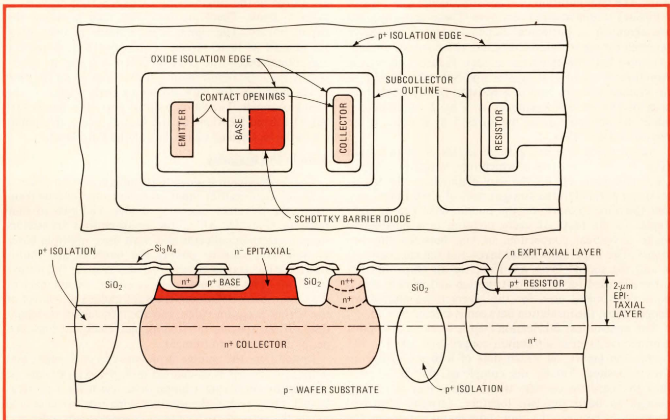
1. Master slice. The master slice used in the System/38 contains an array of 704 gates made from transistors, Schottky clamping diodes, and resistors. To give an idea of scale, the devices are formed in an epitaxial layer typically 2 micrometers thick.
