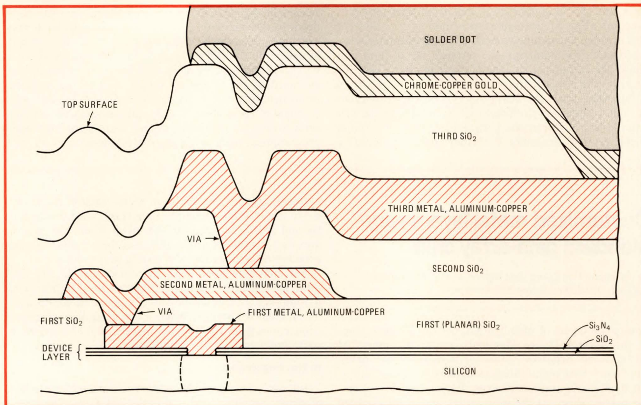
2. Differentiation. To individualize the gate arrays, the first two layers of metal and their interconnections, or vias, are customized. The third layer, used for power distribution and signal input/output, is fixed. Solder dots connect the chips to their ceramic carriers.
