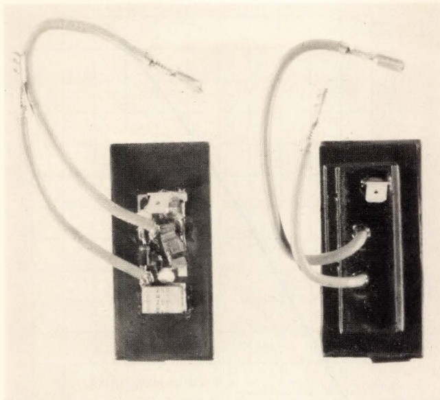
4. Potted power. Porcelain-coated steel replaces alumina in substrate for power-supply circuitry. The same material also replaces the aluminum heat sink. Hybrid thick-film techniques were used in both cases. An unpotted module is pictured to the left.
