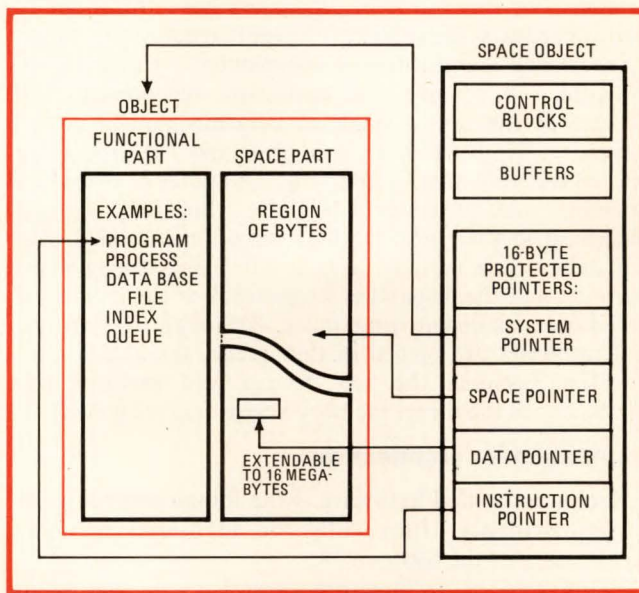
4. Objective memory. All information in memory is stored as an object whose functional part contains the information and whose associated space part provides a set of memory locations. A space object holds the pointers that indicate the location of the object.
