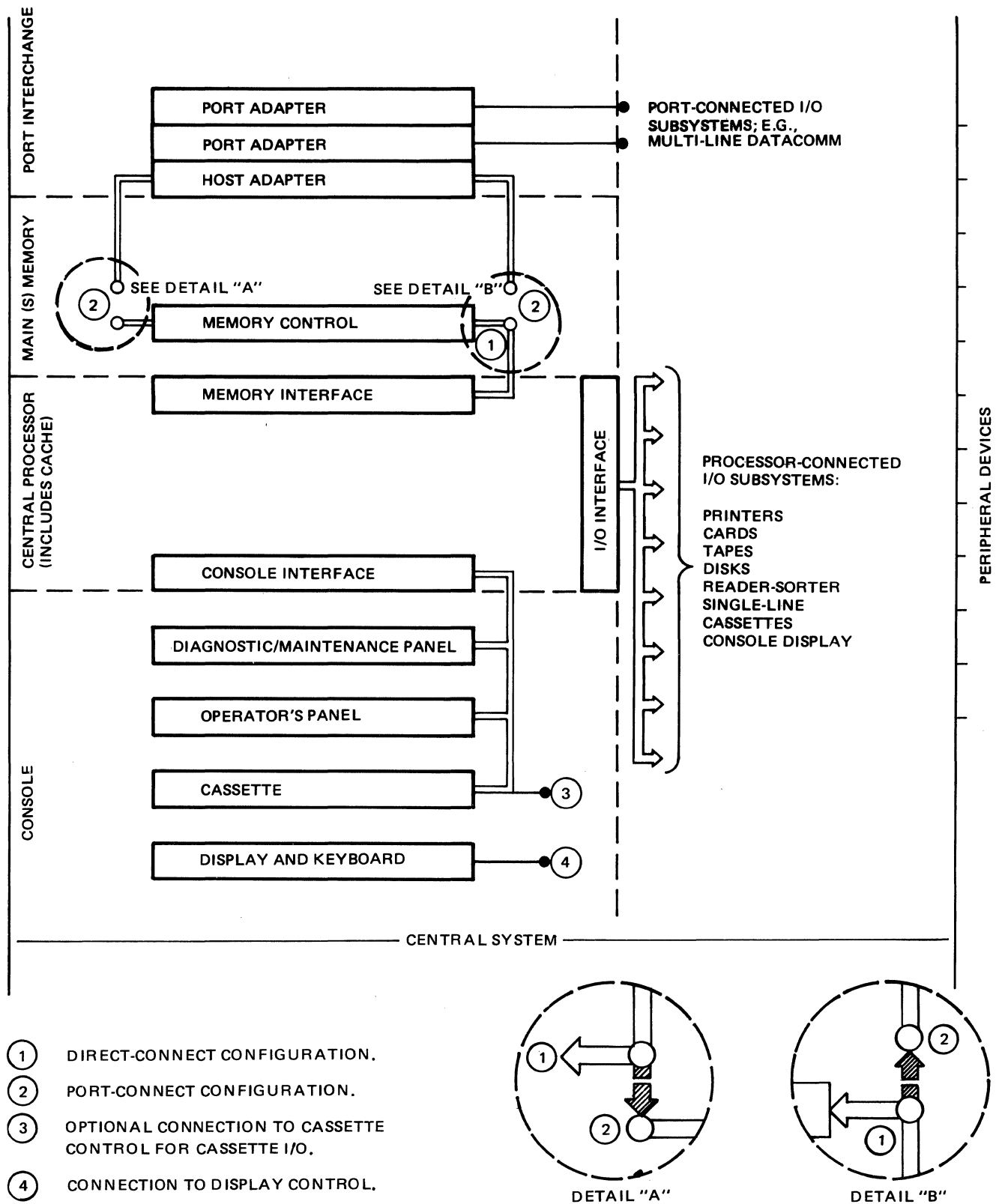
Figure 2-2. Functional Configuration, B 1800 Central Systems
