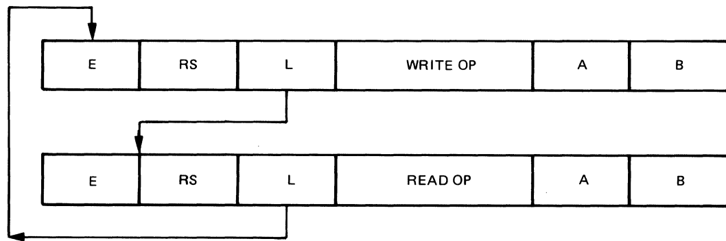
Figure 6-18. Use of Linking for Write Operation
