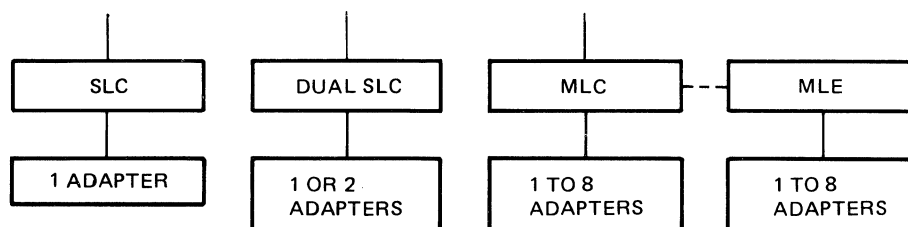
Figure 6-15. Data Communications Subsystem Configurations
