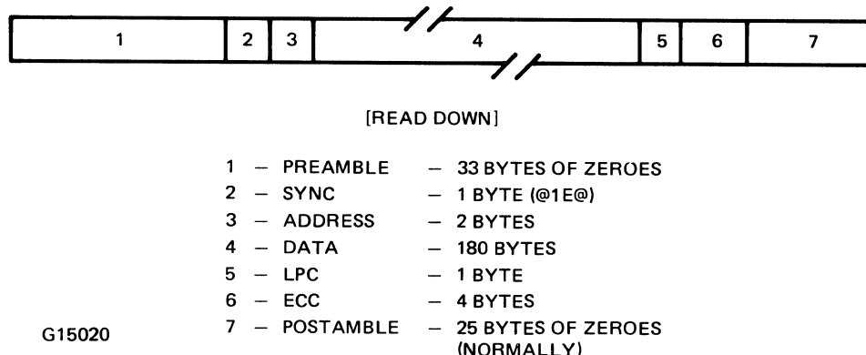
Figure 6-9. Burroughs Cartridge Disk Format
