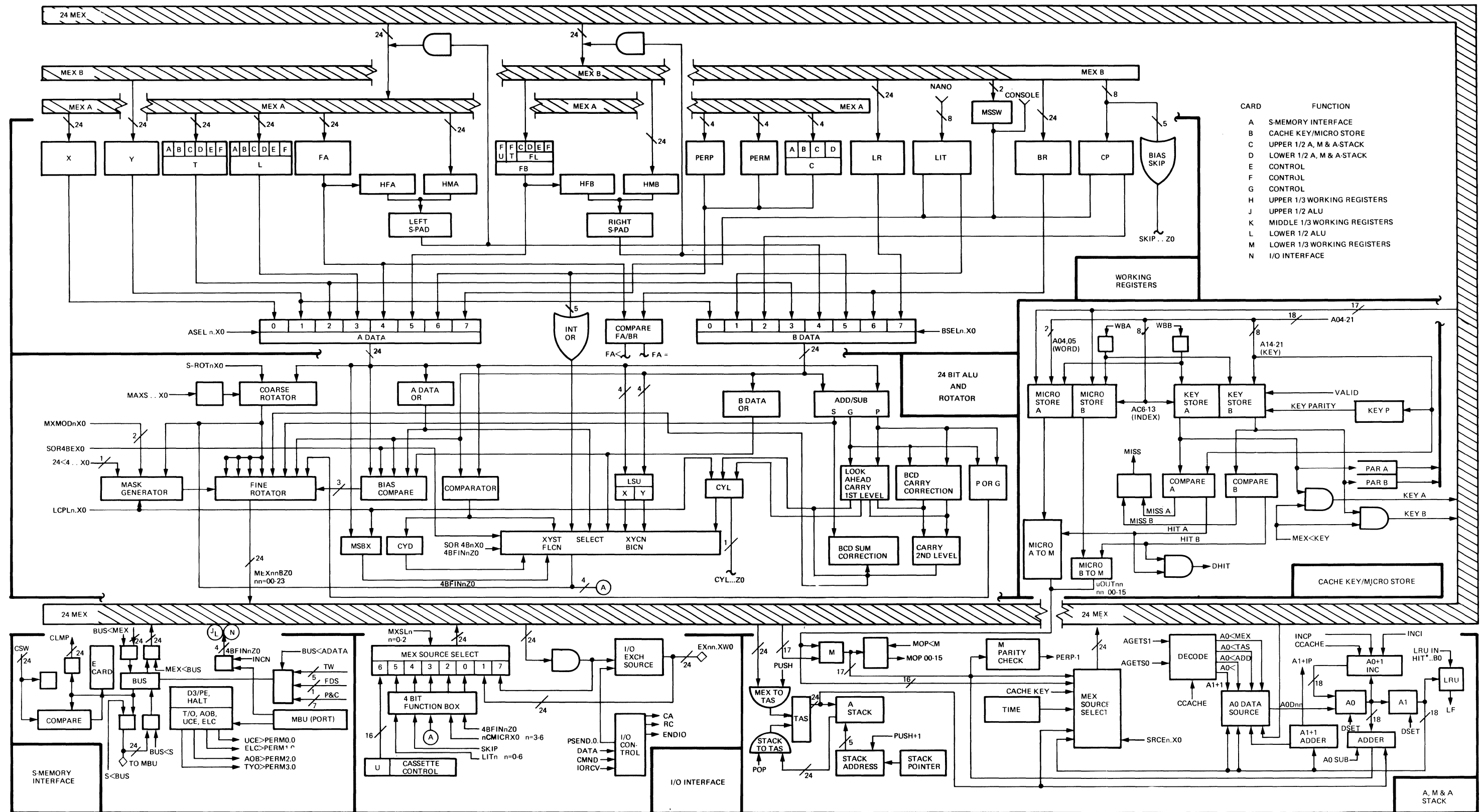
Figure 2-3. Block Diagram, B 1800 Central Processor
