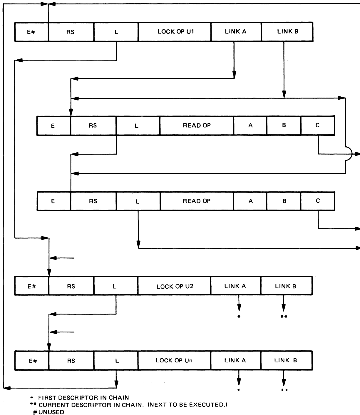
Figure 6-5. I/O Descriptors Showing Linkages
