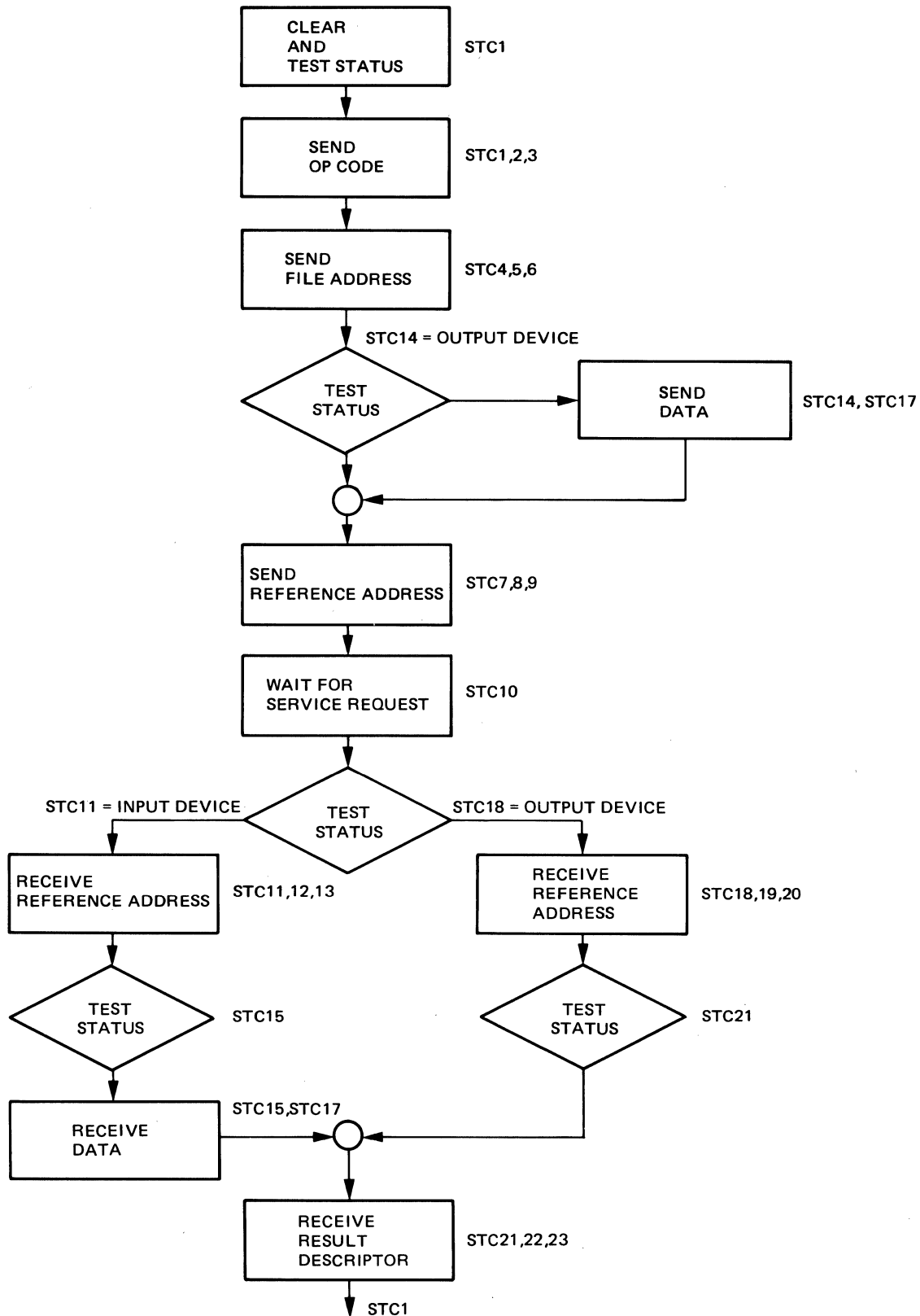
Figure 2-8. Status Count Sequence for an I/O Control
