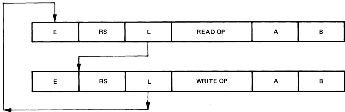
Figure 6-17. Use of Linking for Read Operation
