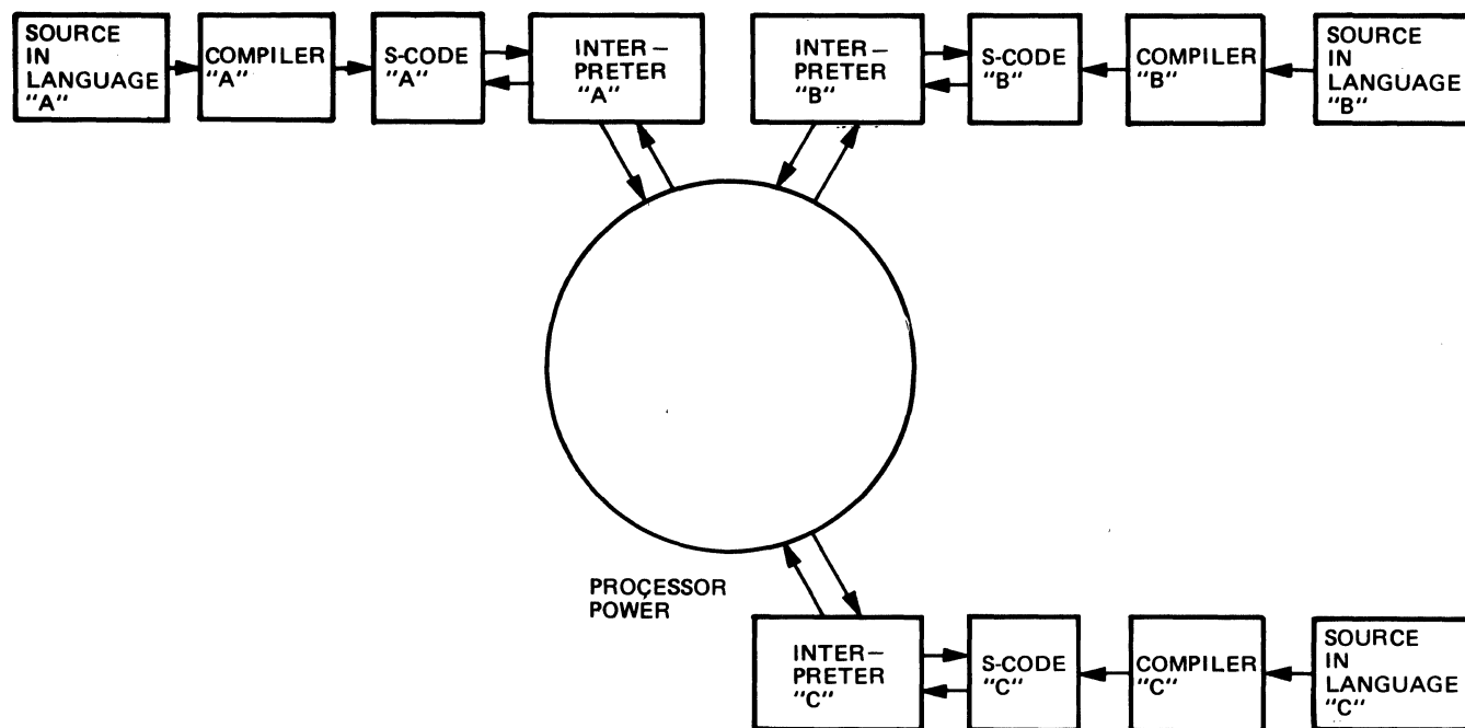
Figure 1-2. B 1800 Approach to Interpretation
