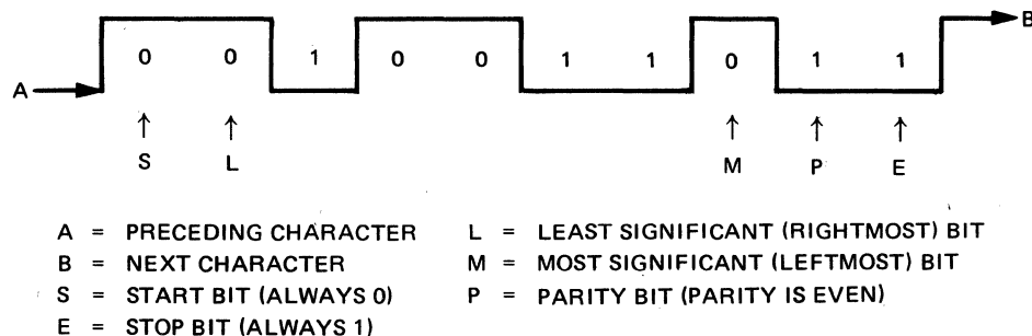
Figure 6-1. Character Transmission, Display Console Control
