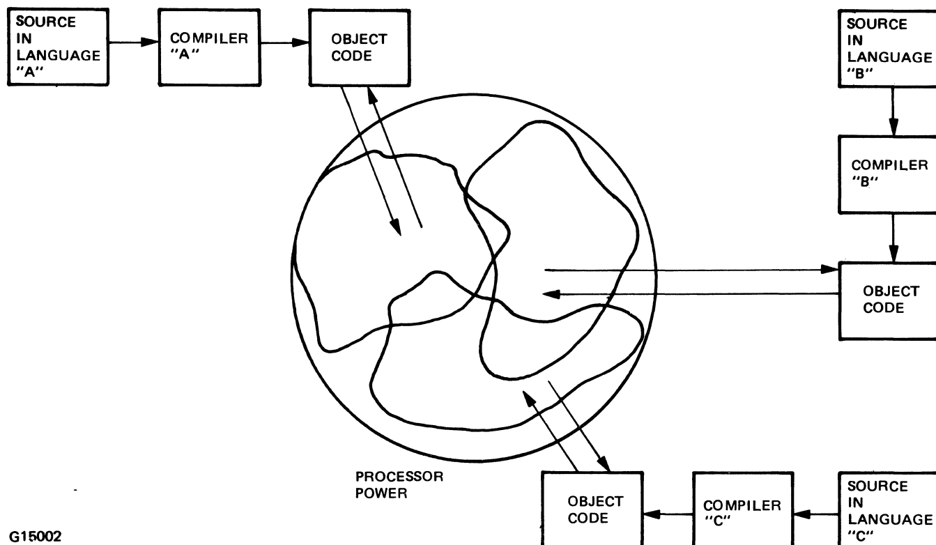
Figure 1-1. Traditional Approach to Interpretation
