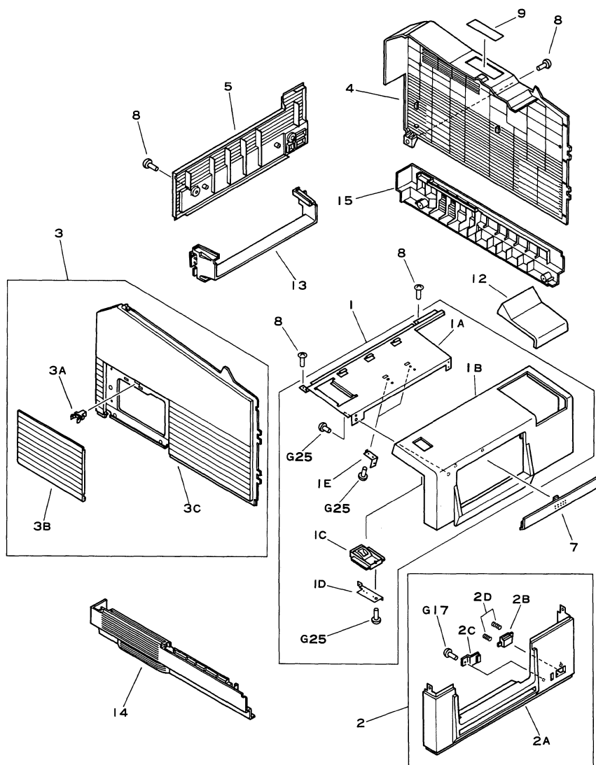
FIGURE 100 EXTERNAL COVER, PANELS, ETC.
