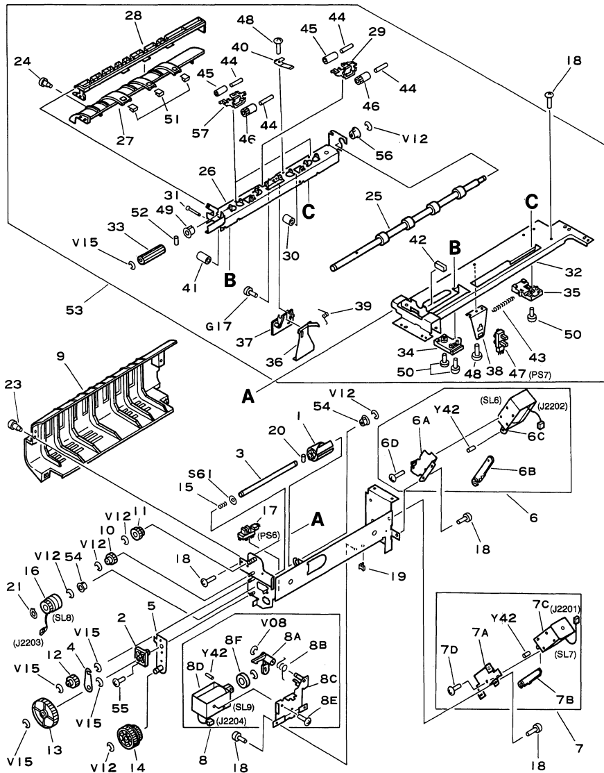
FIGURE 380 DELIVERY ASSEMBLY 排紙部
