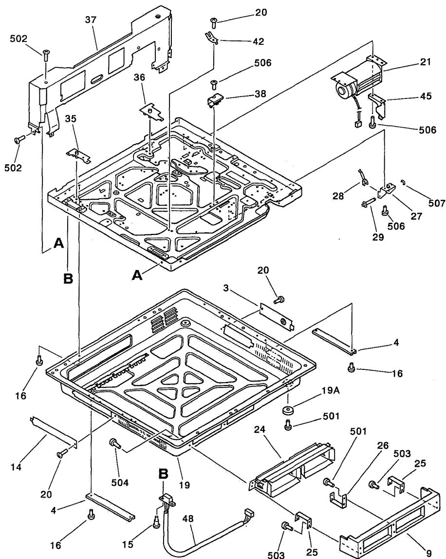
FIGURE 103 BOTTOM CASE ASS'Y ( \frac{2}{2} ) 底箱部 ( \frac{2}{2} )
