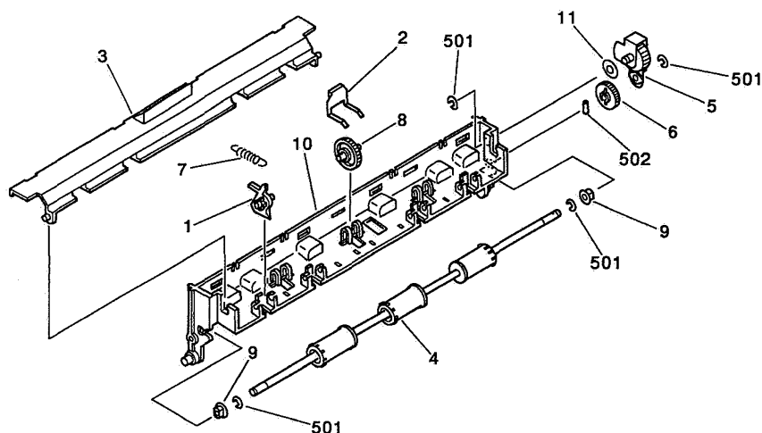
FIGURE 370 FIXING DELIVERY ASS'Y 定着排紙部
