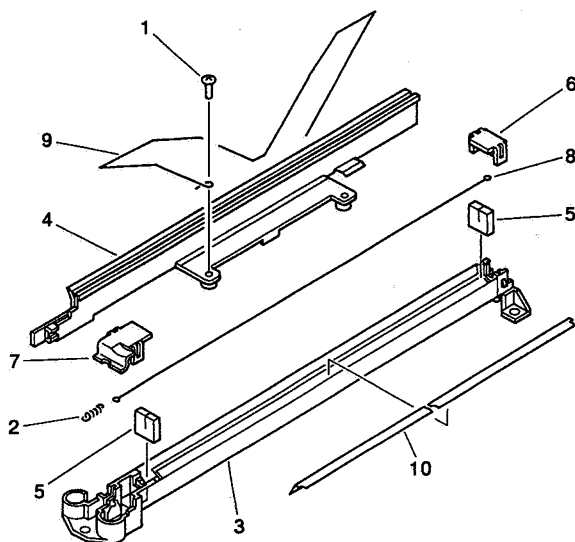
FIGURE 580 TRANSFER CORONA ASS'Y 転写帯電器
