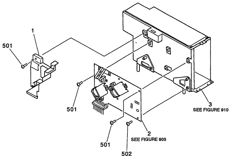
FIGURE 900 ELECTRICAL COMPONENTS ASS'Y
