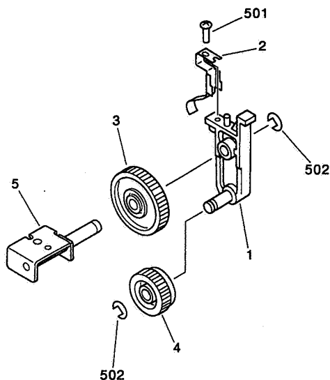
FIGURE 375 DELIVERY COUPLER ASS'Y 排紙カプラ部
