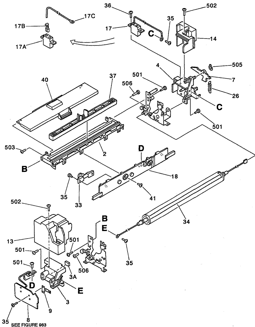
FIGURE 810 FIXING ASS'Y ( \frac{2}{2} ) 定着器 ( \frac{2}{2} )
