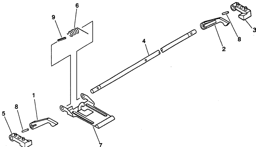
FIGURE 120 PRESSURE ASS'Y 紙加圧部
