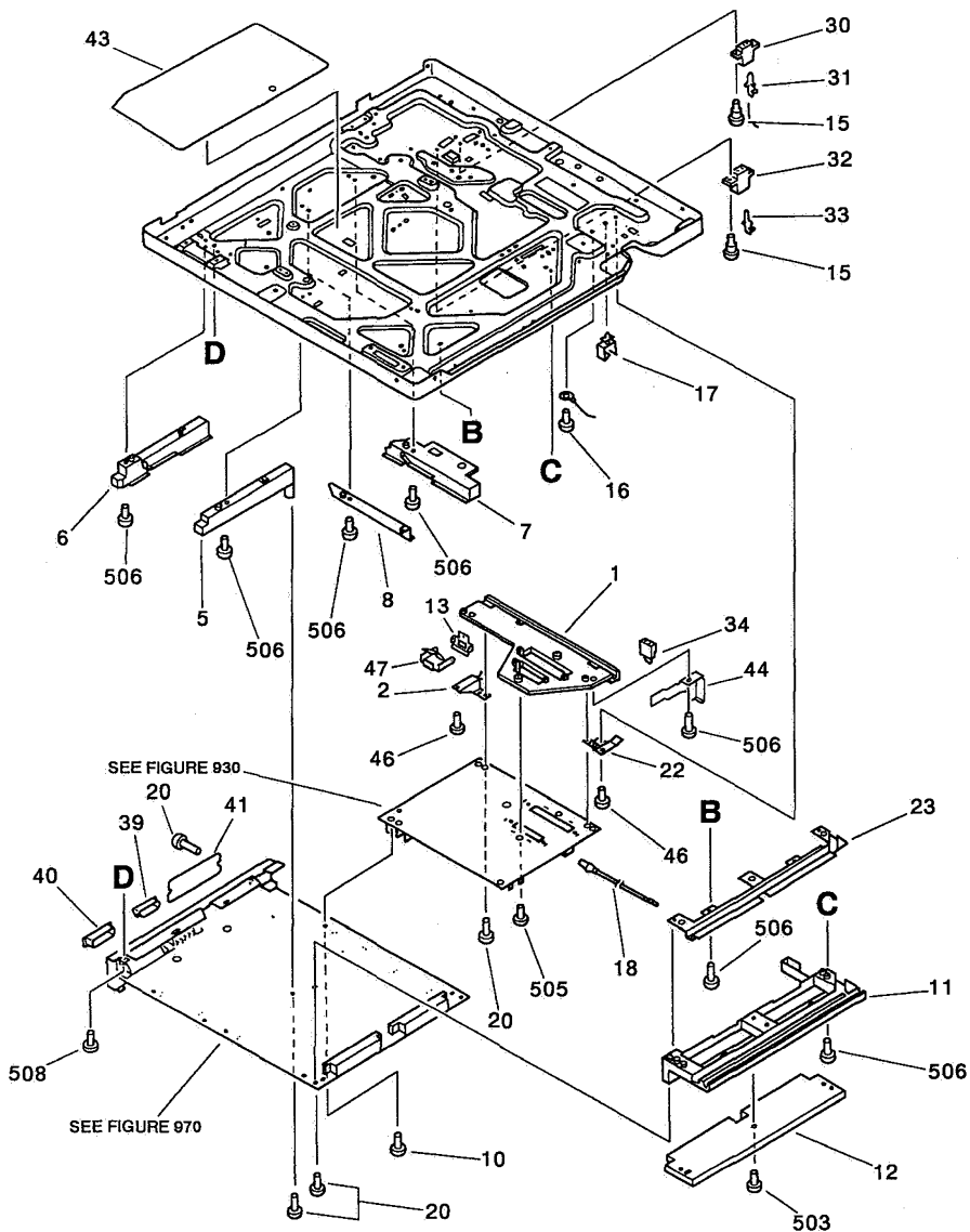
BOTTOM CASE ASS'Y (1/2) 底箱部 (1/2)
