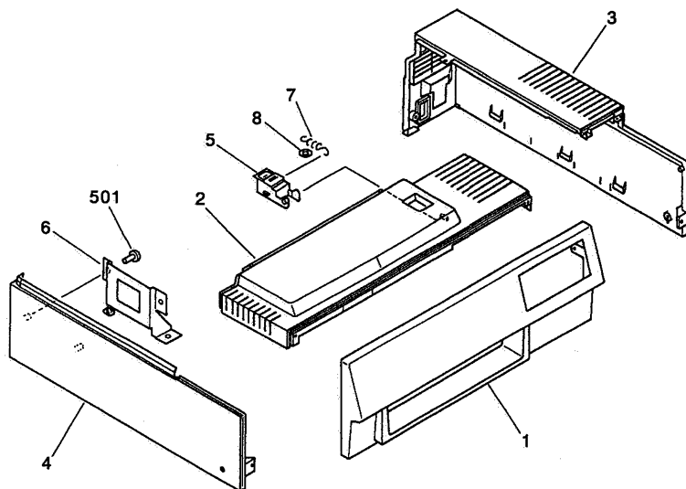
FIGURE 100 EXTERNAL COVERS, PANELS, ETC. 外装カバー
