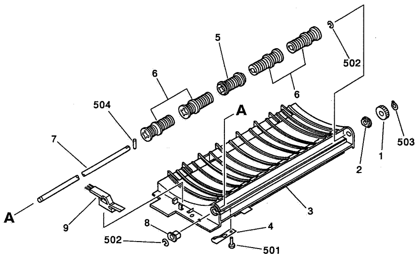
FIGURE 350 FEEDER ASS'Y
