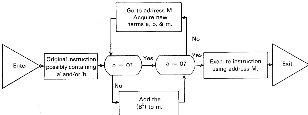
Figure 7-3. Indexing and Indirect Addressing Routine Flow Chart
