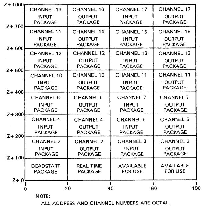
Figure 2-11. Model 176 CM I/O Exchange Package Areas
