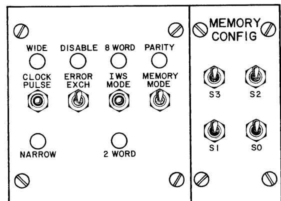
Figure 3-21. Controls on Modules at 5A1 through 5A3 - Model 175
