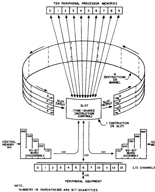
Figure 2-14. Barrel and Slot Operation
