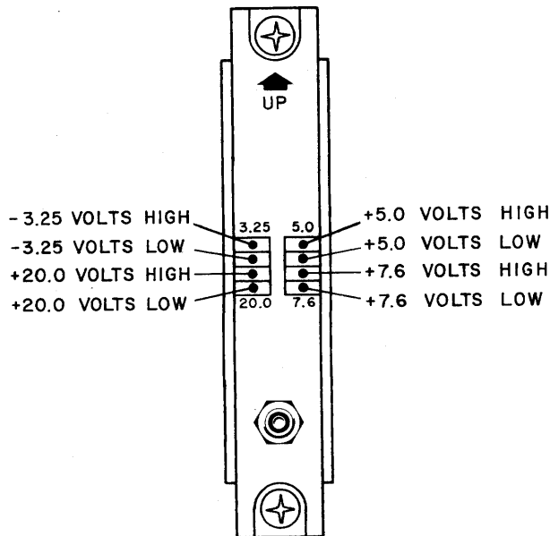
Figure 3-10. PM Module
