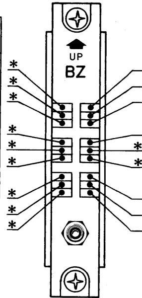
Figure 3-13. Module at PPS F25 - Models 171 through 175
