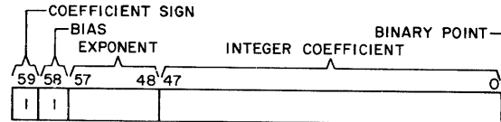
Figure 5-4. Floating-Point Format
