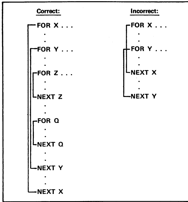
Figure 4-14. FOR...NEXT Loops
