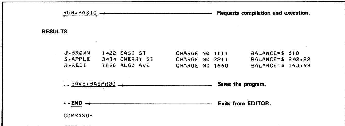
Figure 11-3. Using Data Files Under NOS/BE (Sheet 2 of 2)
