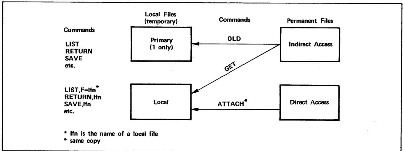
Figure D-1. NOS Files
