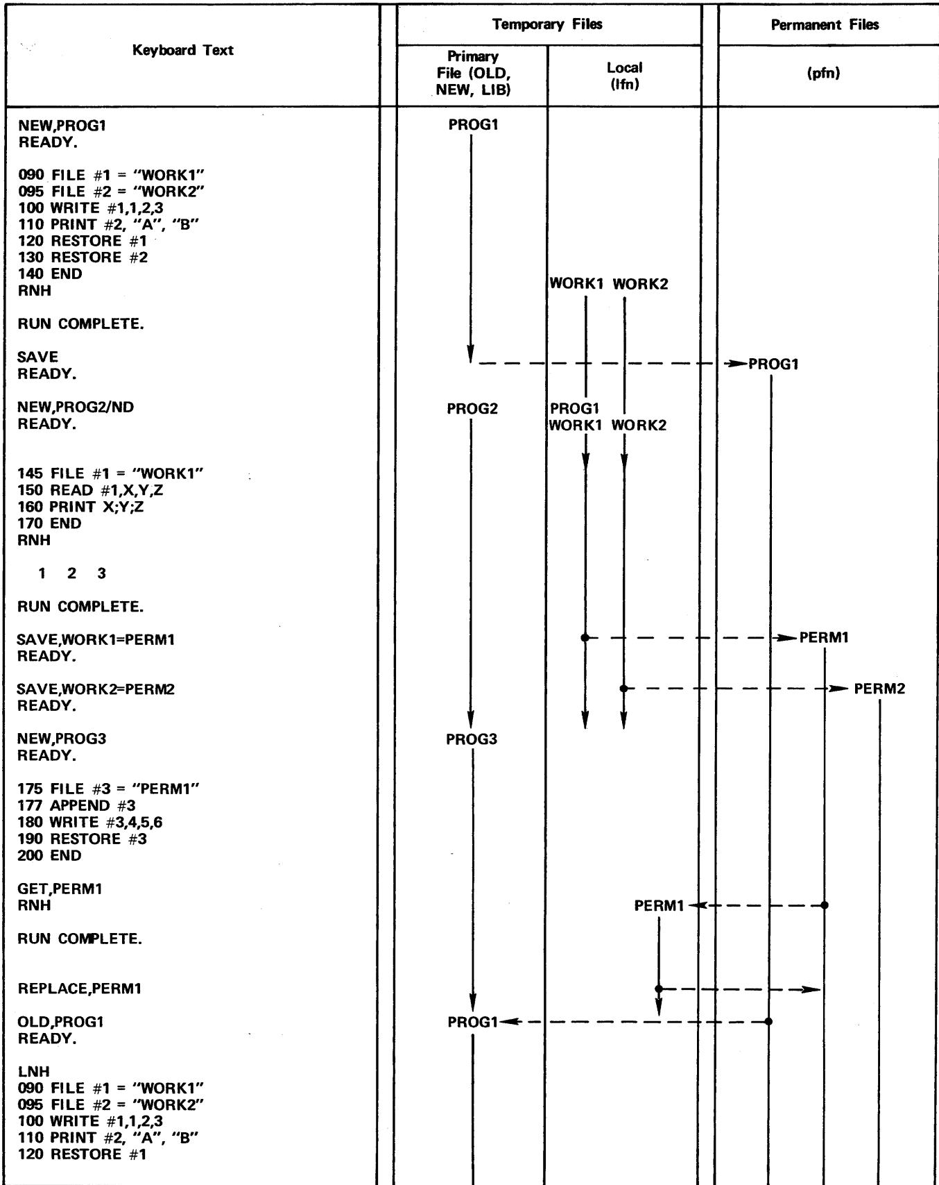
Figure D-4. File Control Commands (Sheet 1 of 2)
