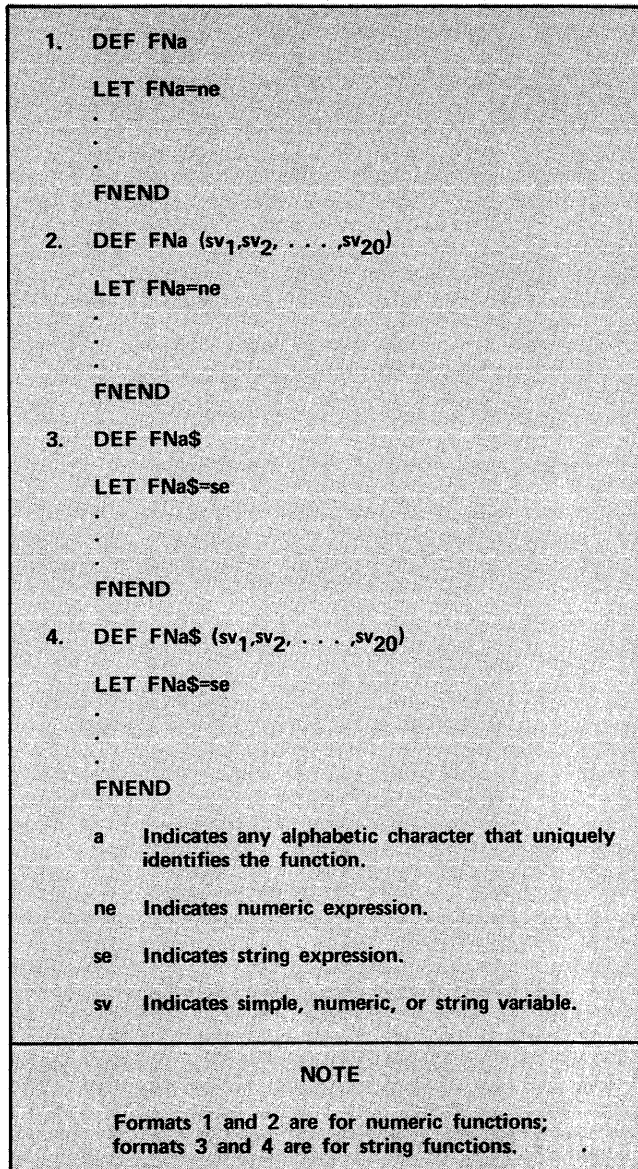
Figure 5-36. Multiple-Line Function Format with DEF . . . FNEND
