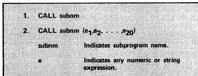
Figure 6-7. CALL Statement Format
