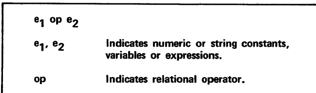
Figure 2-4. Format for Simple Relational Expressions
