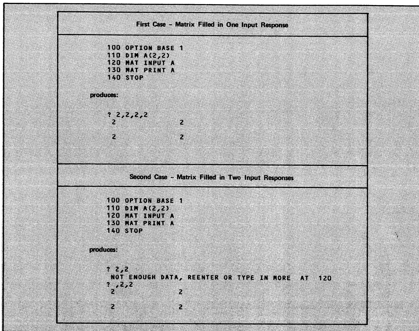
Figure 8-32. MAT INPUT Example
