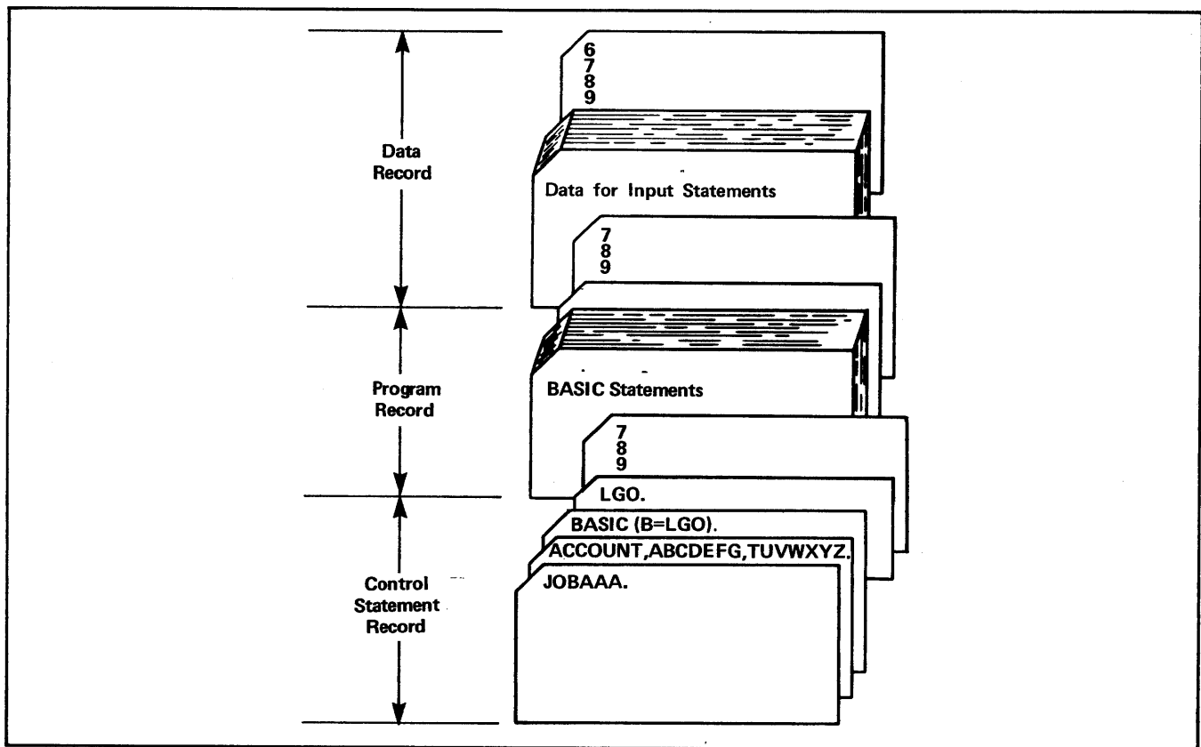
Figure 12-4. BASIC Compile, Load, and Execute Job Under NOS/BE
