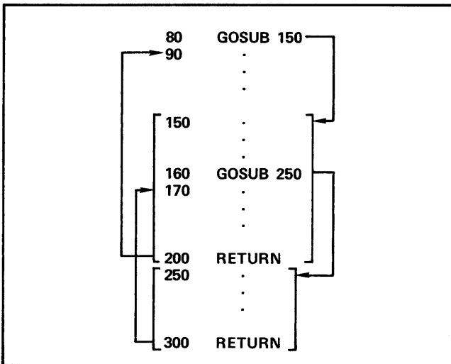
Figure 6-3. Nested Subroutines
