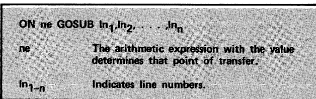
Figure 6-4. ON GOSUB Statement Format
