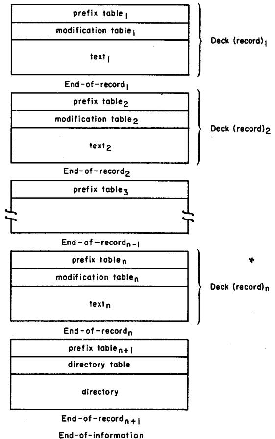
Figure 9-1. Library File Format
