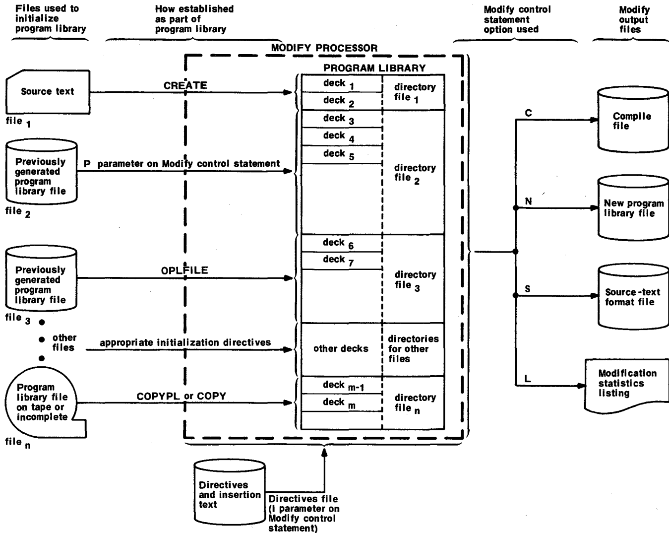
Figure 1-1. Simplified Modify Organization
