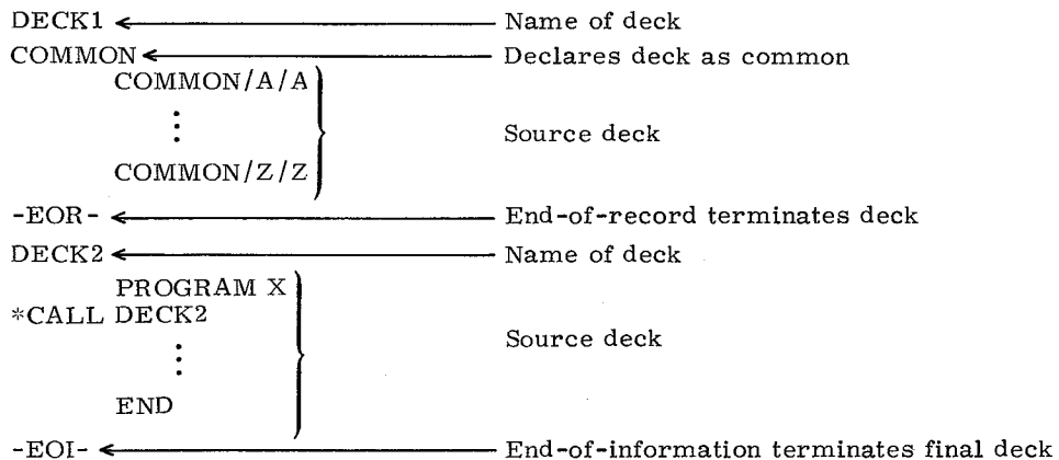
Figure 3-1. Modify Source Deck
