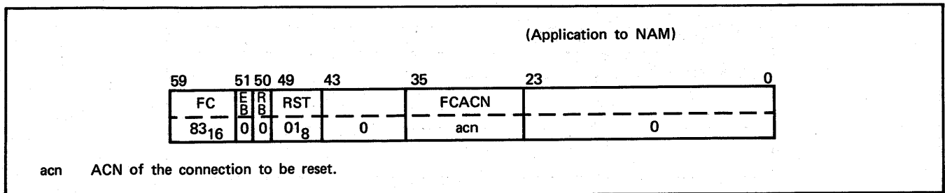
Figure 4-13. Format for Reset (FC/RST)
