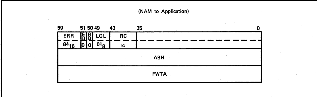
Figure 4-16. Format for Logical Error (ERR/LGL) (Sheet 1 of 2)
