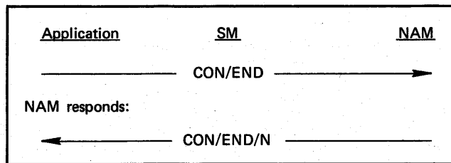
Figure 4-1. CONnection/END Supervisory Message
