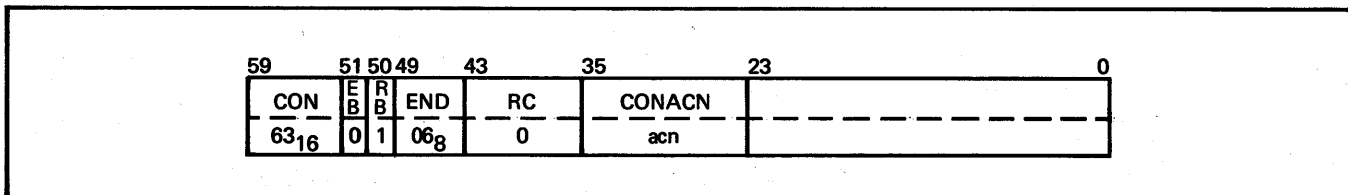
Figure 4-5. Format for Connection Ended (CON/END/N) NAM to Application
