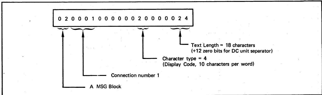
Figure 2-7. ABH Configuration of 'ENTERΔINPUTΔPLEASE'
