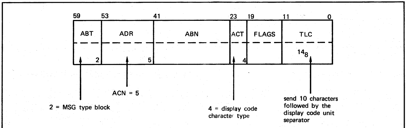
Figure 3-3. ABH Configuration of 'INPUT PLS'
