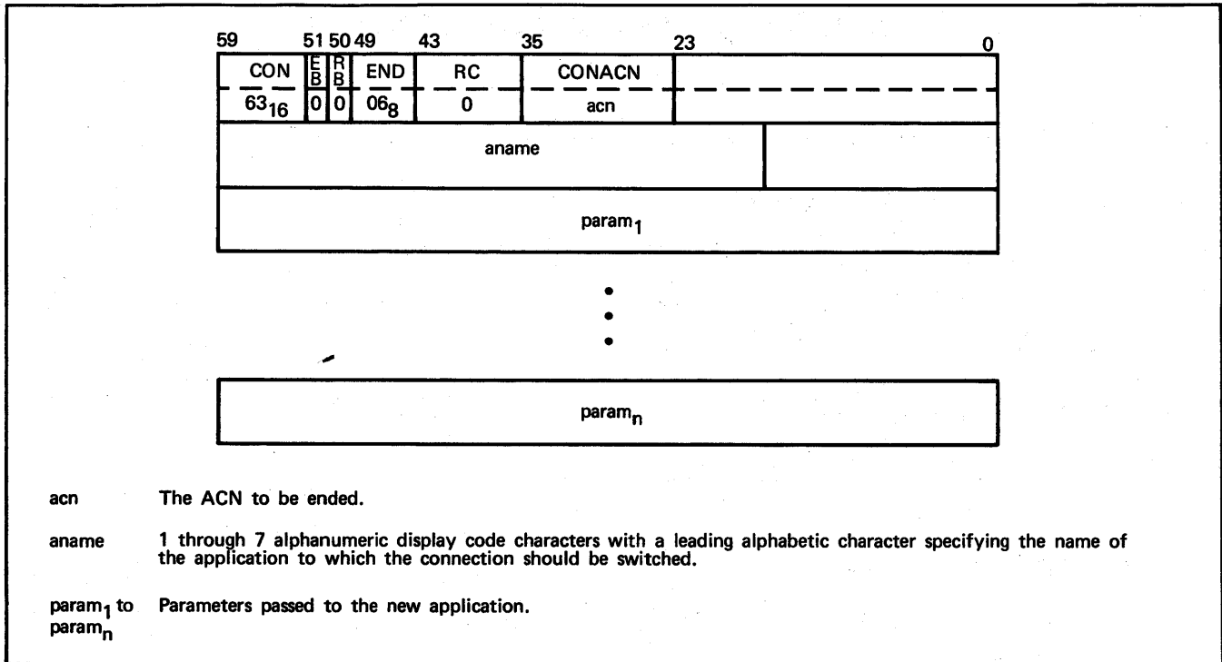
Figure 4-4. Format for Connection Ended (CON/END) Application to NAM
