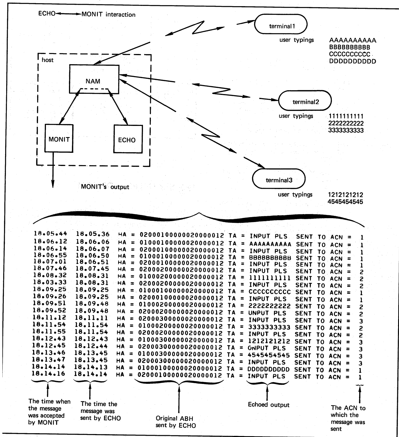
Figure 6-10. ECHO-MONIT Interaction
