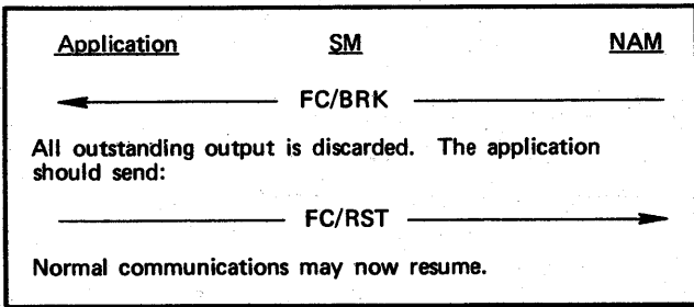
Figure 4-9. FC/BRK Protocol
