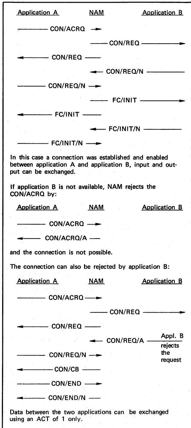
Figure 6-5. Application-to-Application Communication
