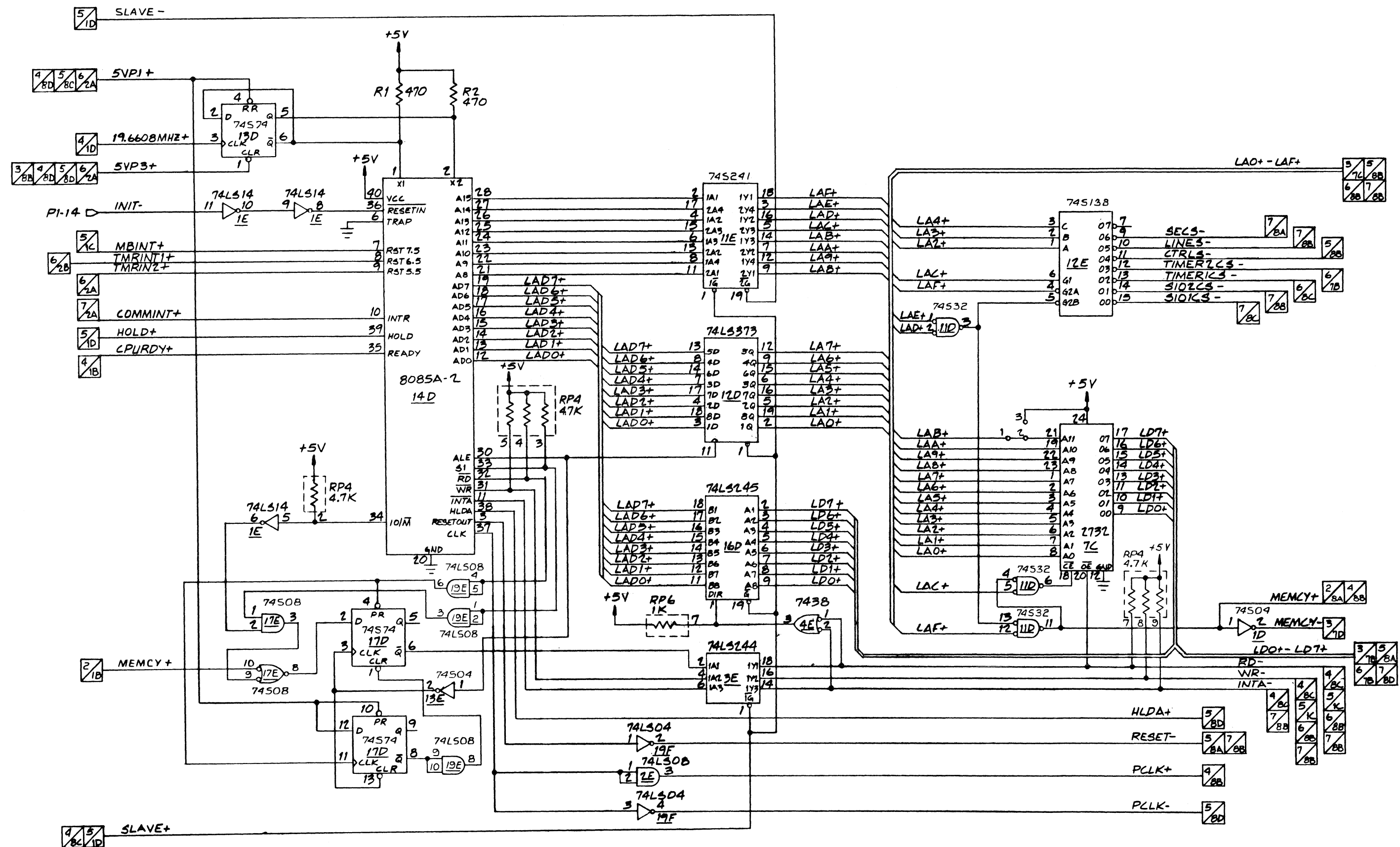
Figure 14-7. MLCP Board Schematic. (Page 2 of 8)
