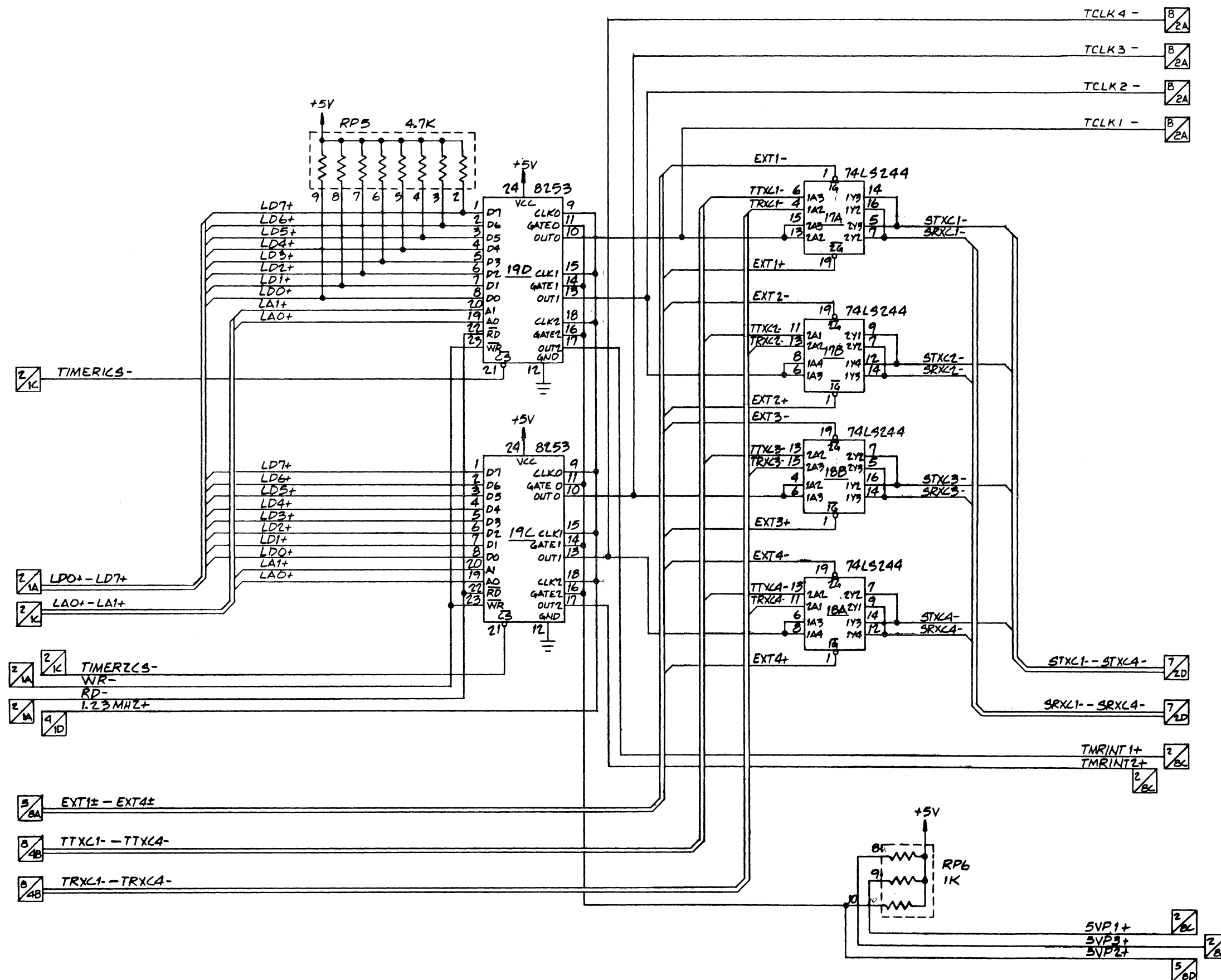
Figure 14-7. MLCP Board Schematic. (Page 6 of 8)
