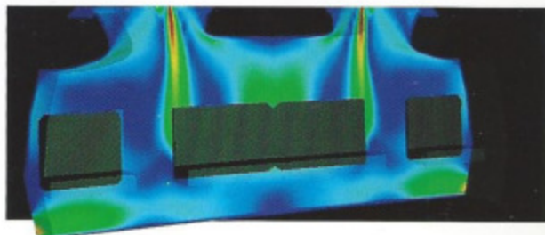
Left, natural convection heat transfer in a three-dimensional electronics enclosure, computed using FIDAP.
