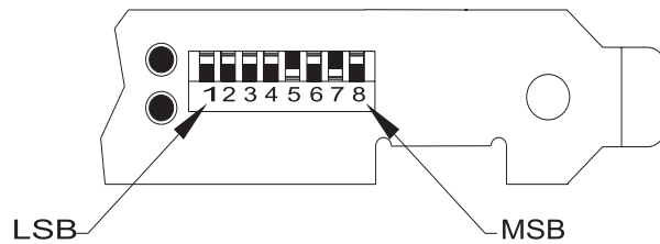
Figure 1-Node ID Switch
