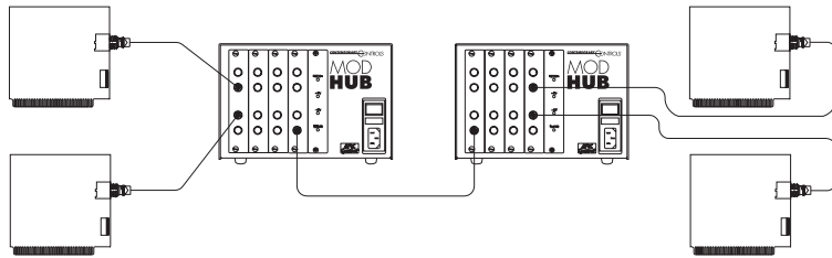
Figure 2-Active hubs can be cascaded for greater distances.
