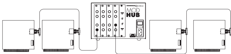
Figure 3-Bus segments can be extended through active hubs.
