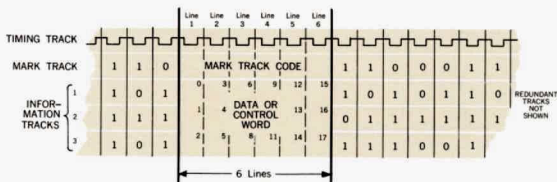
Figure 2 Basic Six Line Tape Unit
