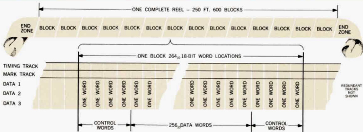
Figure 3 Control And Data Word Assignments
