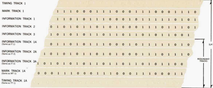
Figure 1 Track Allocation Showing Redundantly Paired Tracks
