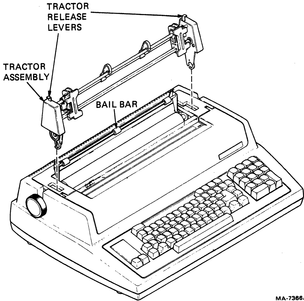
Figure 4-4 Tractor Removal
