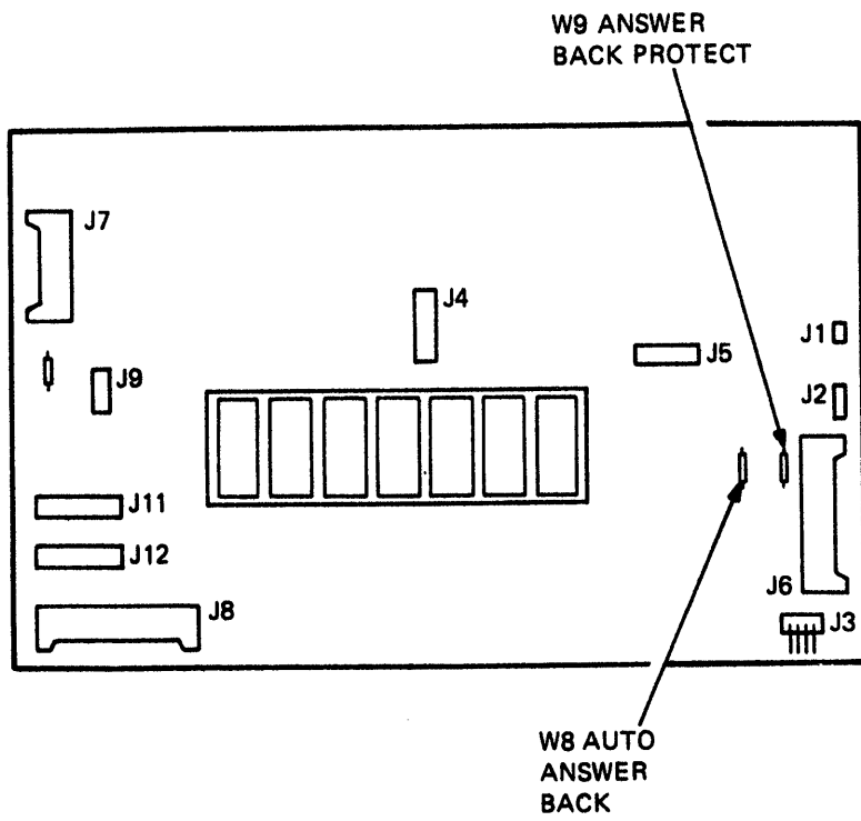
Figure 3-1 Jumper Selectable Features
