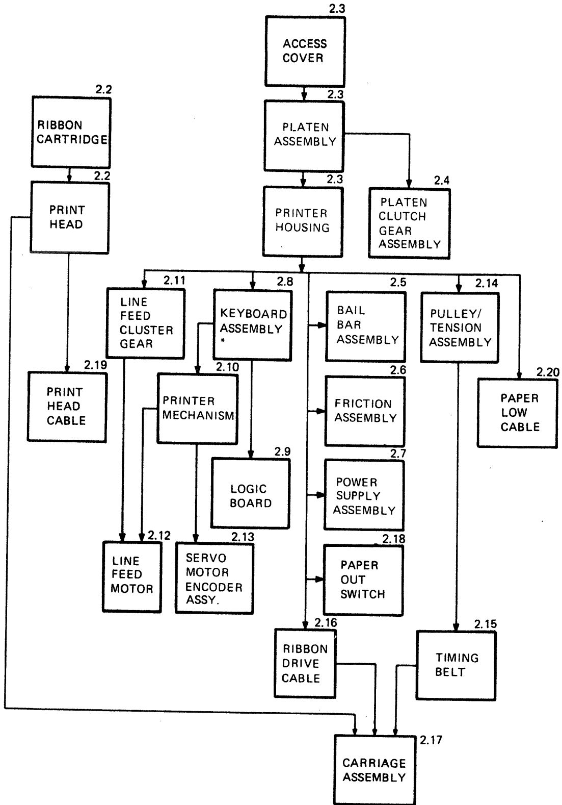
Figure 2-1 Assembly Removal Sequence
