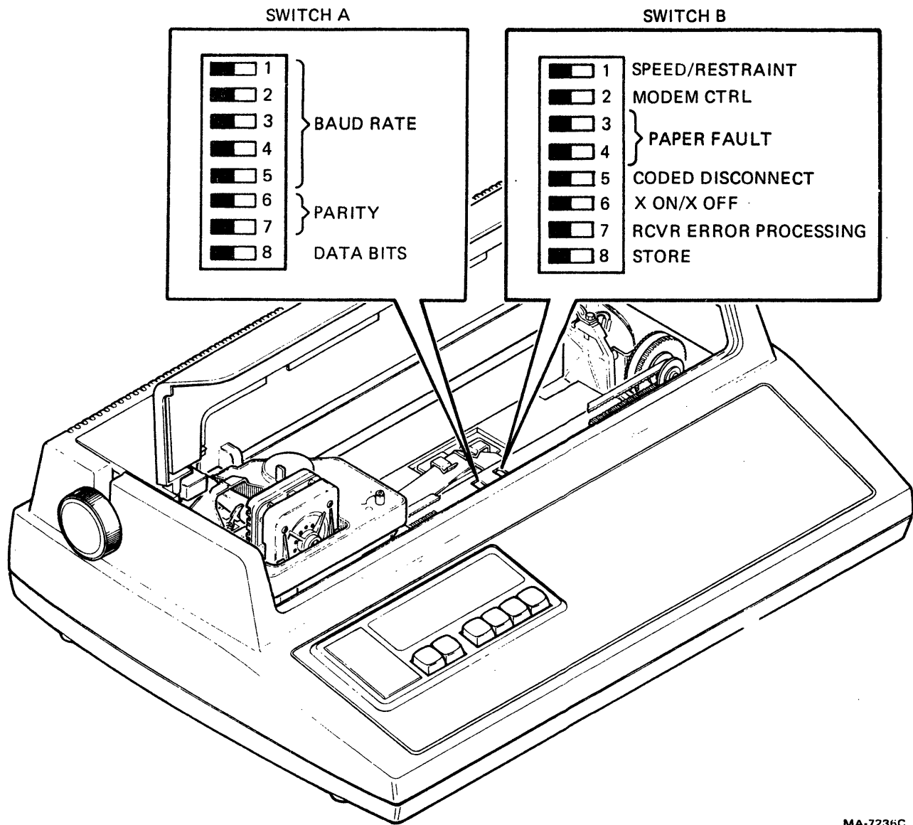
Figure 5-1 Communication Switches
