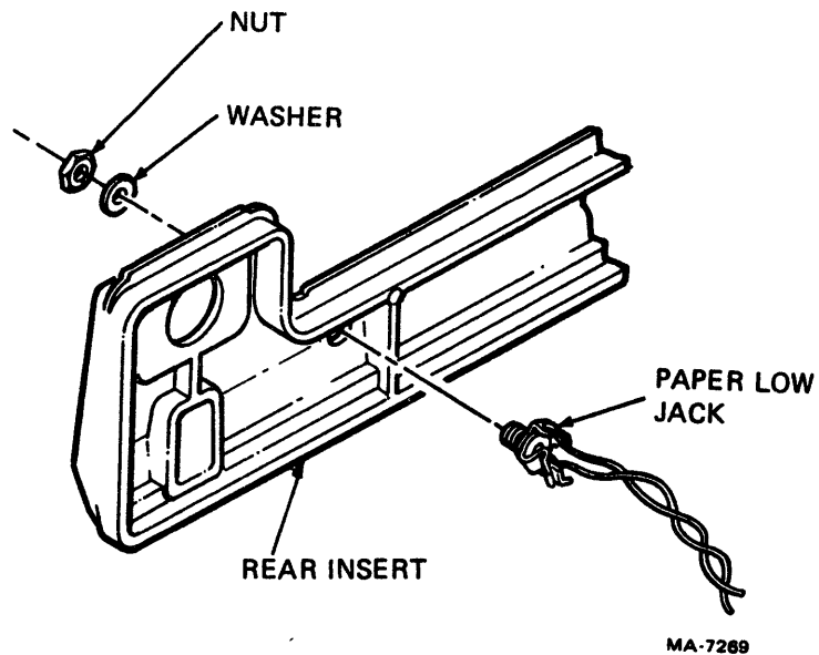
Figure 2-31 Paper Low Jack Removal
