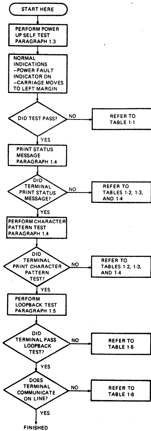
Figure 1-1 Troubleshooting Procedure
