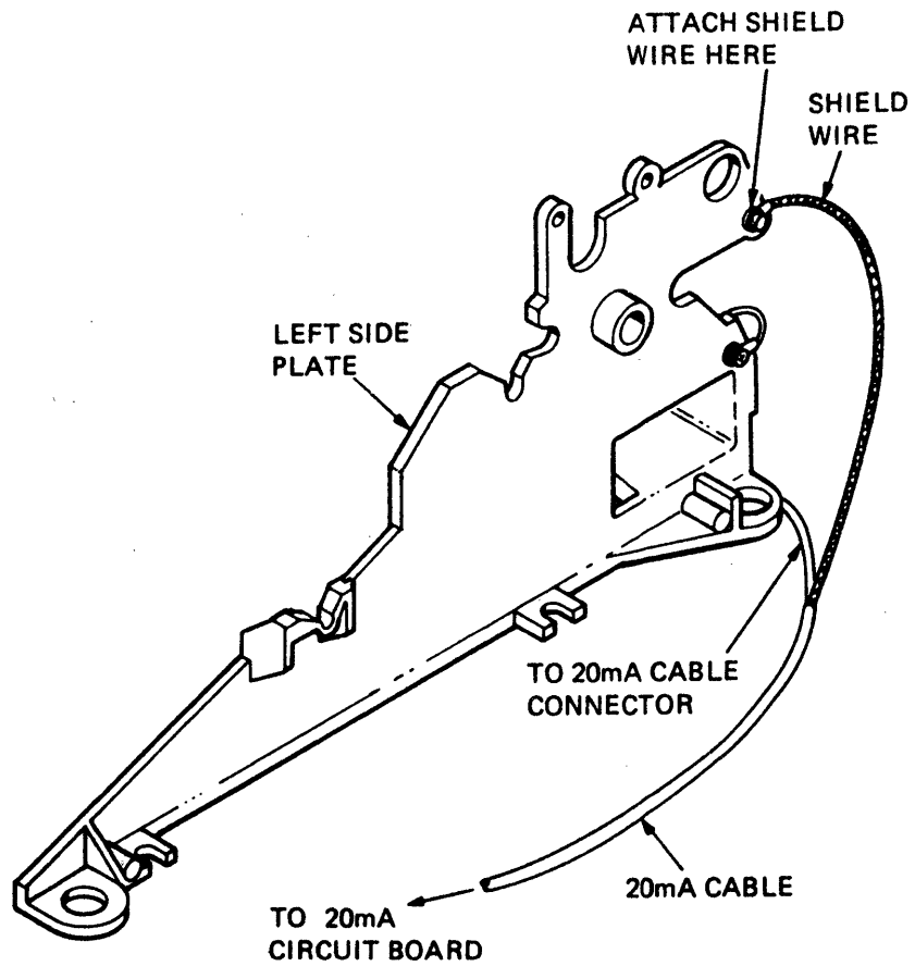
Figure 4-8 Detaching Shield Wire
