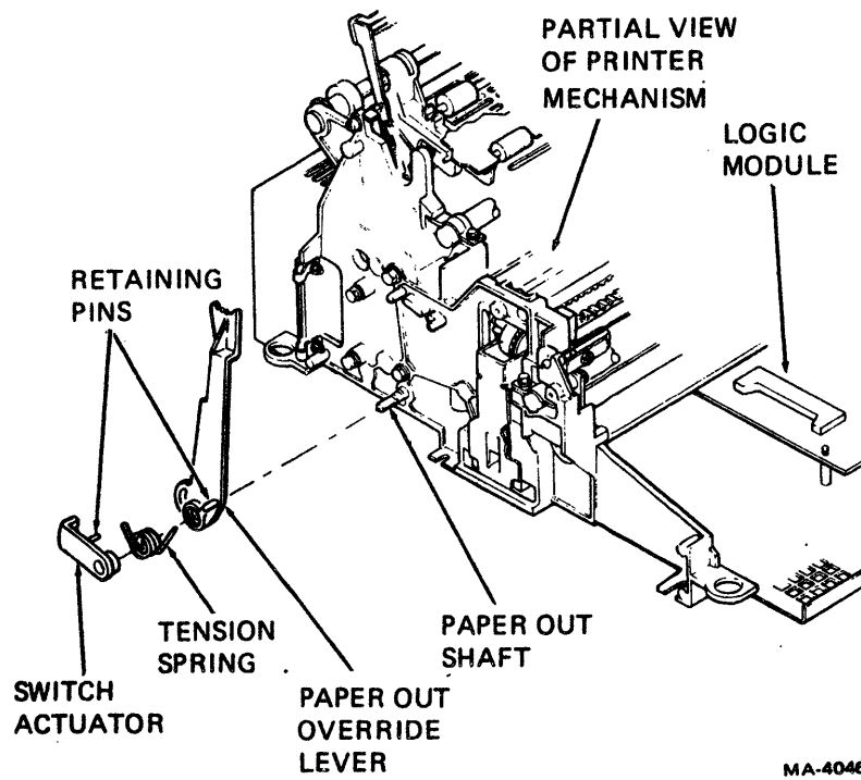
Figure 2-28 Paper Out Override Lever Removal
