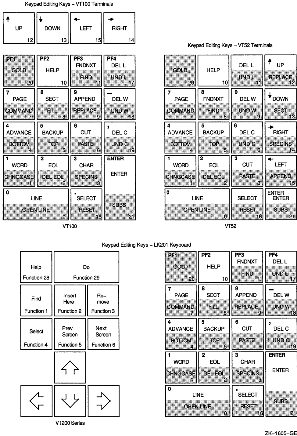
Figure 2-1 VT100, VT52, and LK201 Keypads
