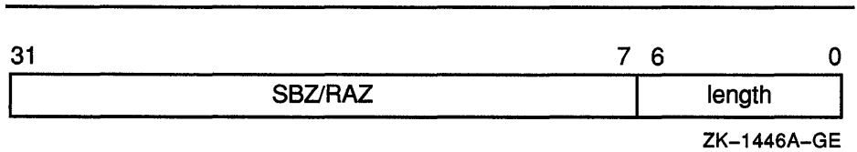
Figure 10–2 Vector Length Register (VLR)
