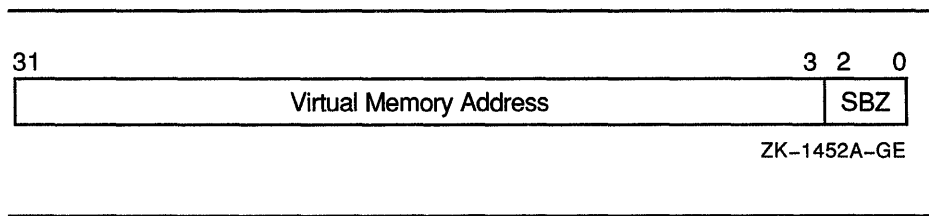
Figure 10–9 Vector State Address Register (VSAR)
