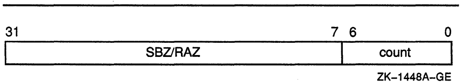
Figure 10–4 Vector Count Register (VCR)
