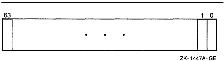
Figure 10–3 Vector Mask Register (VMR)
