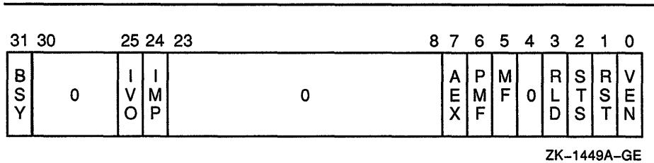
Figure 10–5 Vector Processor Status Register (VPSR)
