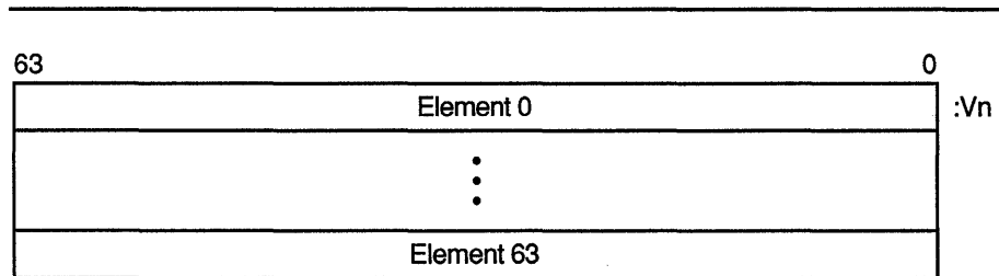
Figure 10–1 Vector Register
