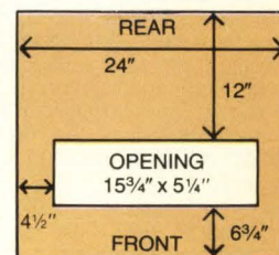
Diagram of top showing location of cutout.
