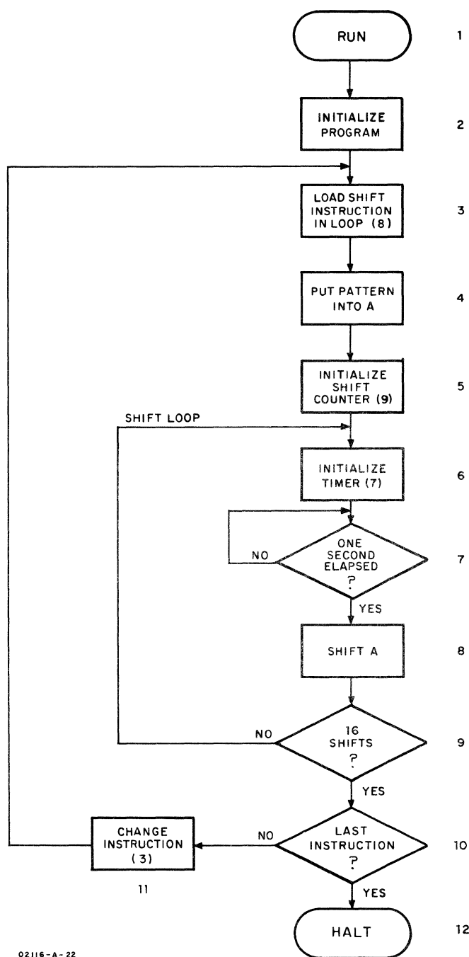
Figure 4-7. Flowchart for Shift-Rotate Demonstration
