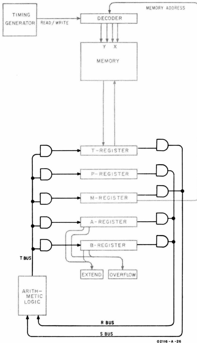
Figure 3-12. Bus System Block Diagram
