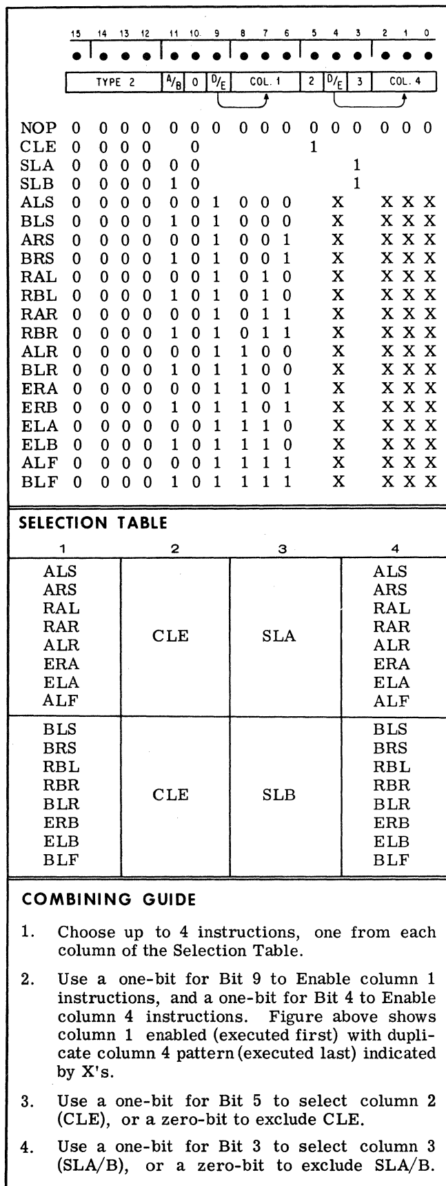
Figure 2-5. Shift-Rotate Instructions
