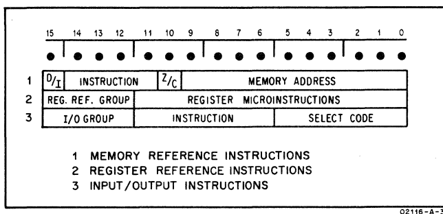
Figure 2-3. Basic Instruction Formats
