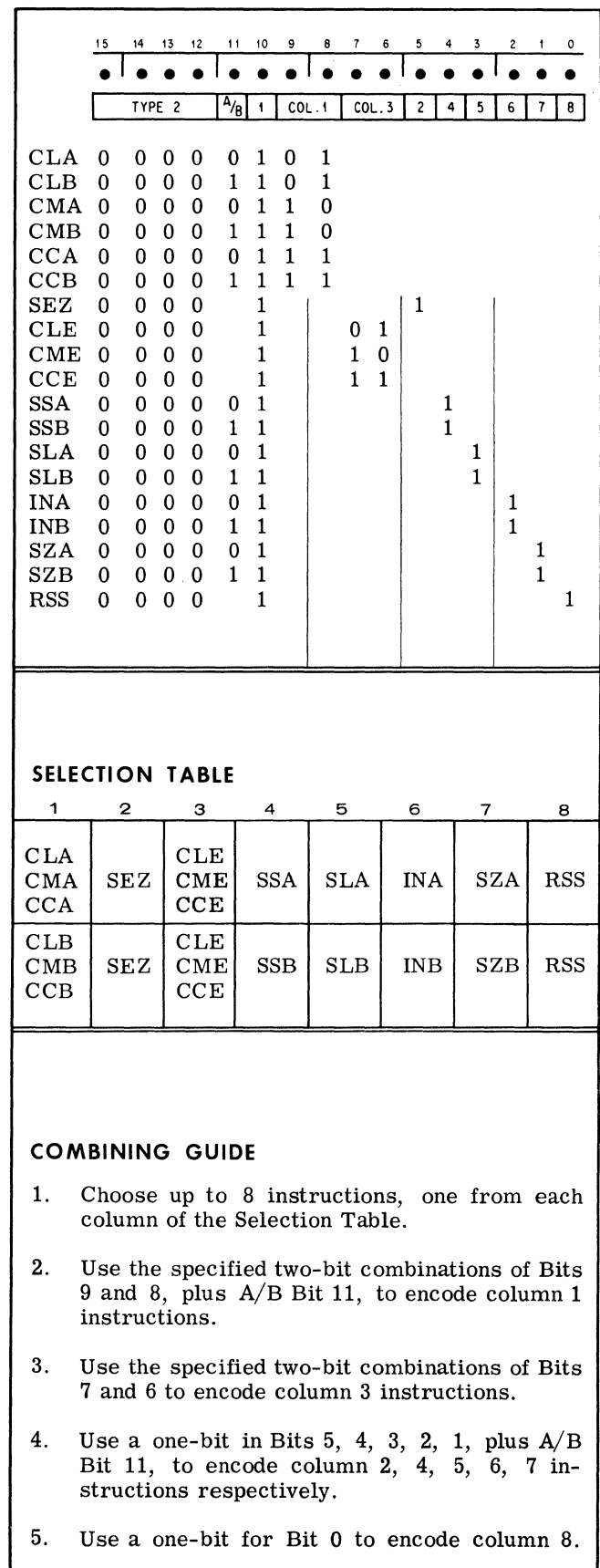
Figure 2-6. Alter-Skip Instructions
