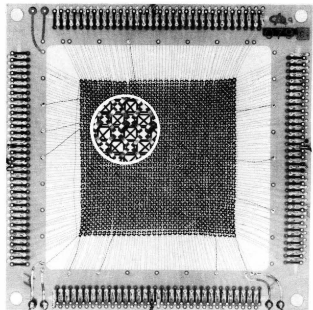
Figure 3-10. Core Plane
