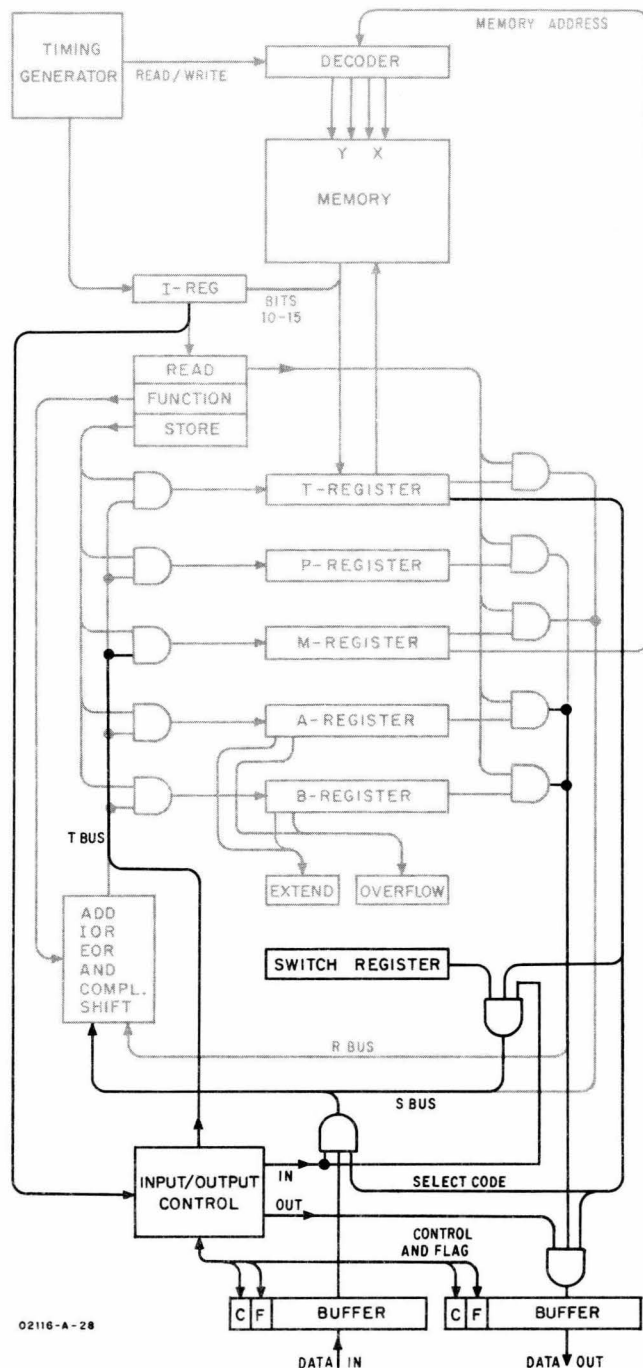
Figure 3-14. Input/Output System Block Diagram
