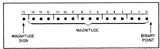
Figure 2-8. Basic Data Format
