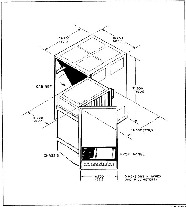
Figure 2-1. HP 2116A Dimensions (Showing Chassis Extended)
