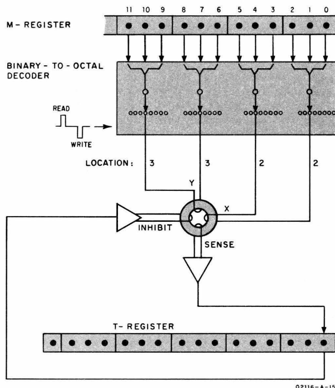
Figure 3-8. Core Addressing, Reading, and Writing
