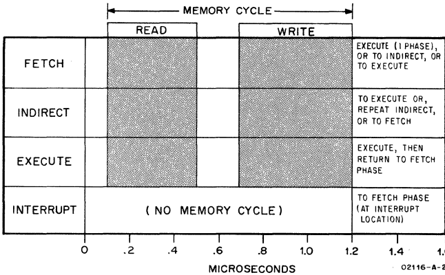
Figure 2-2. Machine Timing
