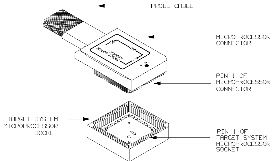
Figure 3-2. Installing into a PLCC type socket
