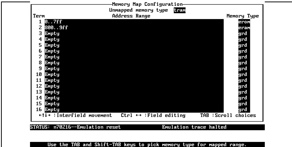
Figure 2-4. Memory Map Configuration
