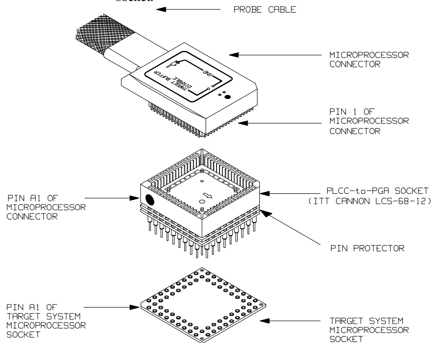
Figure 3-3. Installing into a PGA type socket
