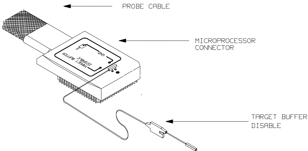
Figure 3-1. Auxiliary Output Lines
