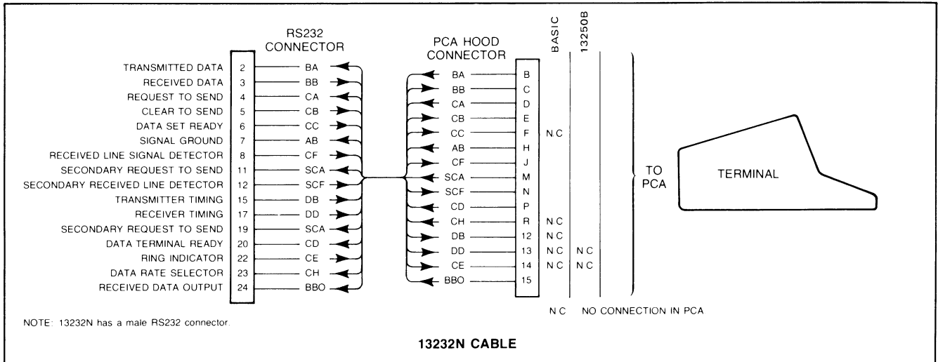
Figure 7-16. Standard Communications Cabling
