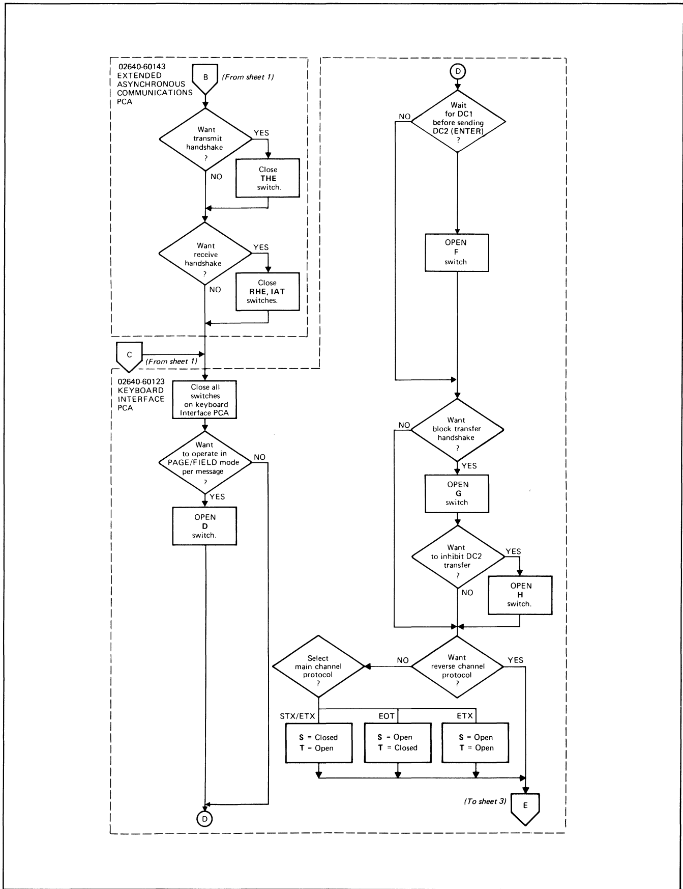
Figure 5-10. Data Communications Configuration Flowchart (Sheet 2 of 4)
