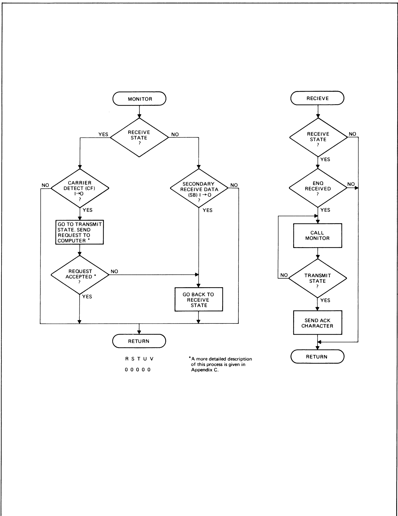
Figure 5-8. Reverse Channel Protocol
