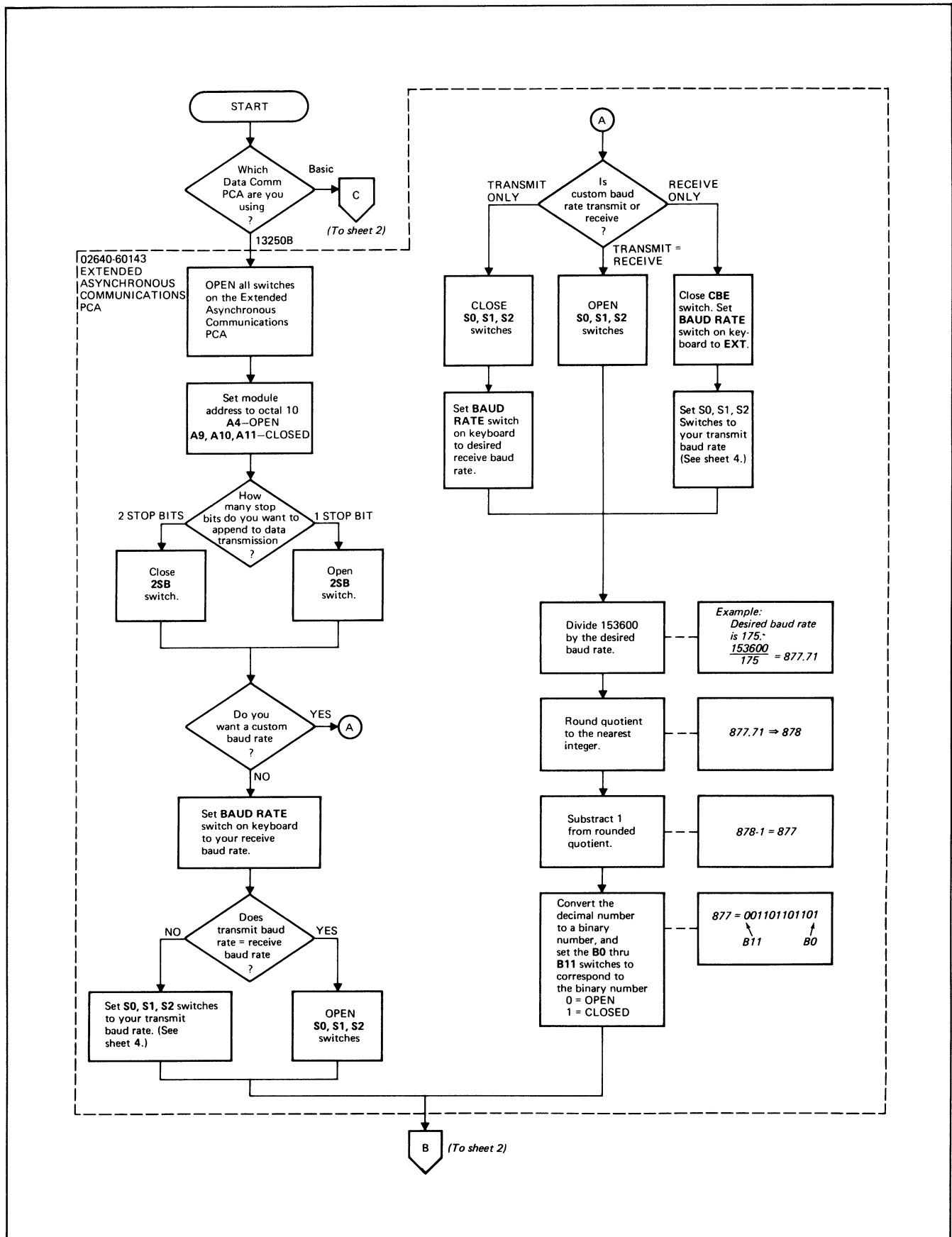
Figure 5-10. Data Communications Configuration Flowchart (Sheet 1 of 4)
