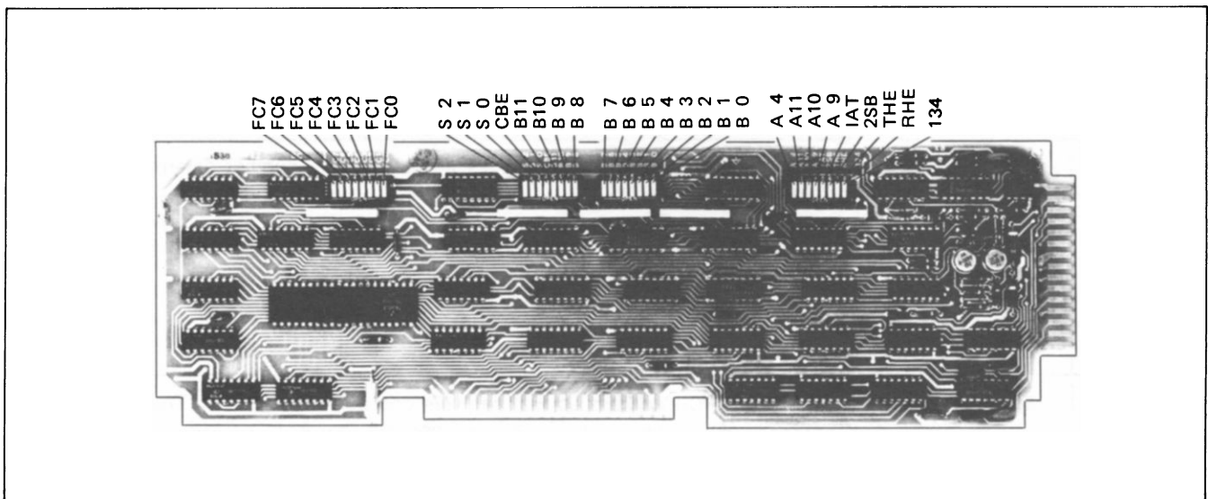
Figure 7-15. Extended Asynchronous Communications PCA Strapping Options
