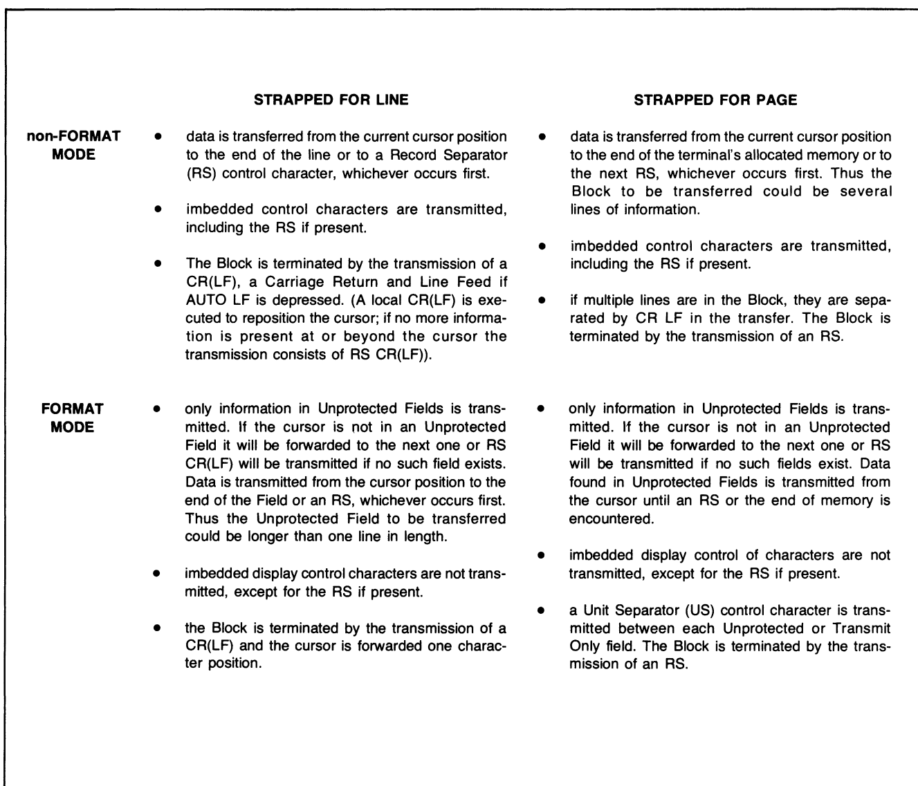
Figure 5-4. Block Mode Operation
