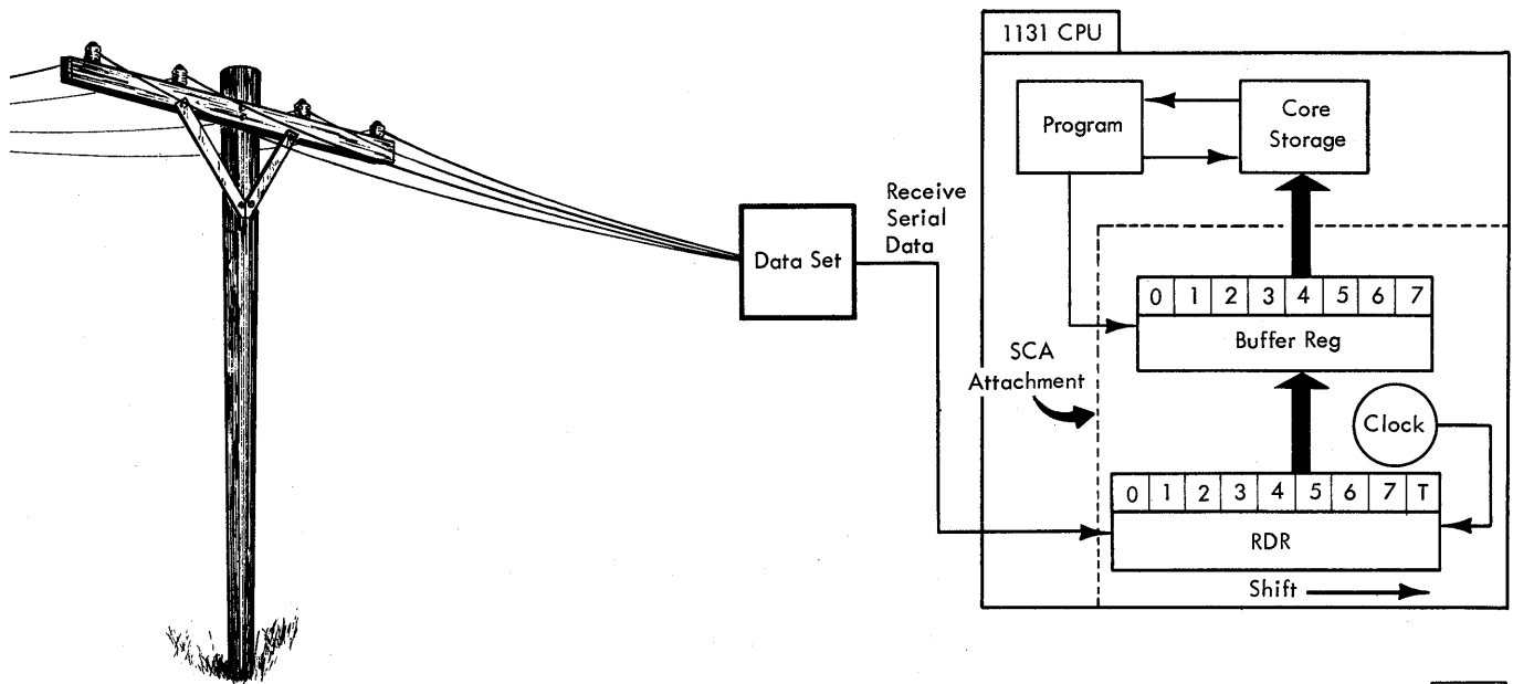
Figure 6-6. Receive Operation
