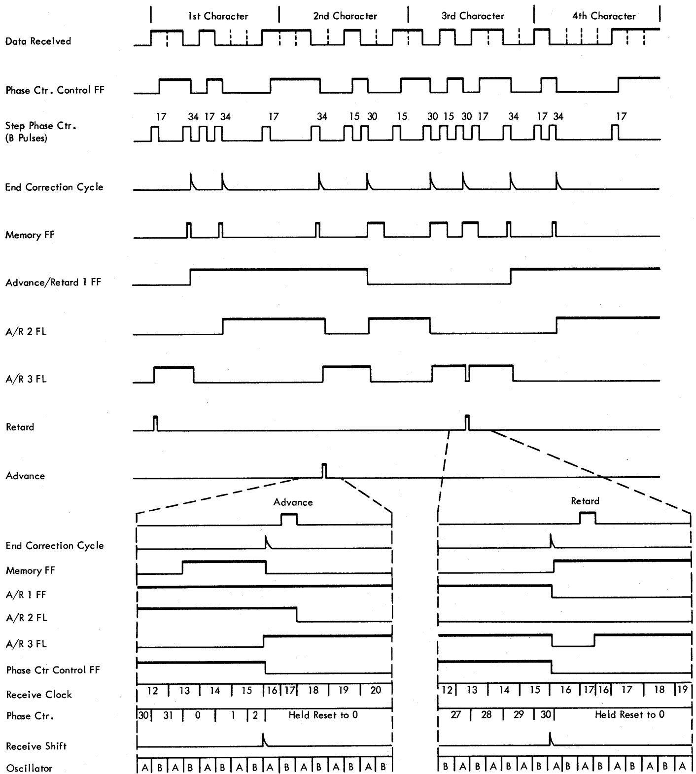
Figure 6-10. Phase Counter
