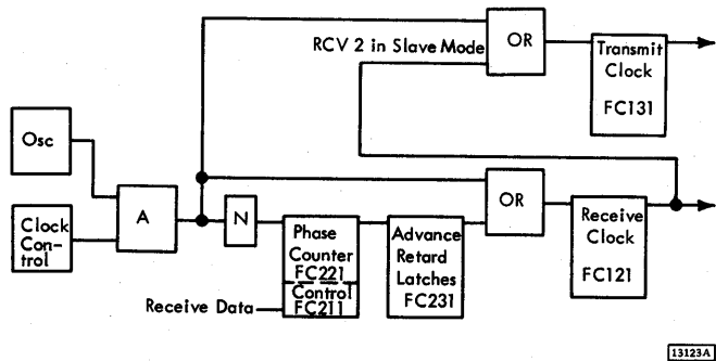
Figure 6-8. Clocks
