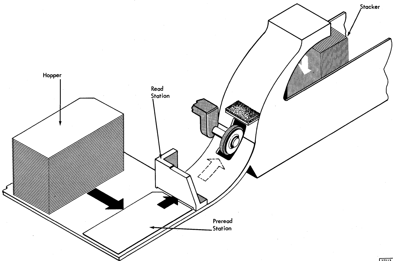
Figure 7-2. 2501 Card Path
