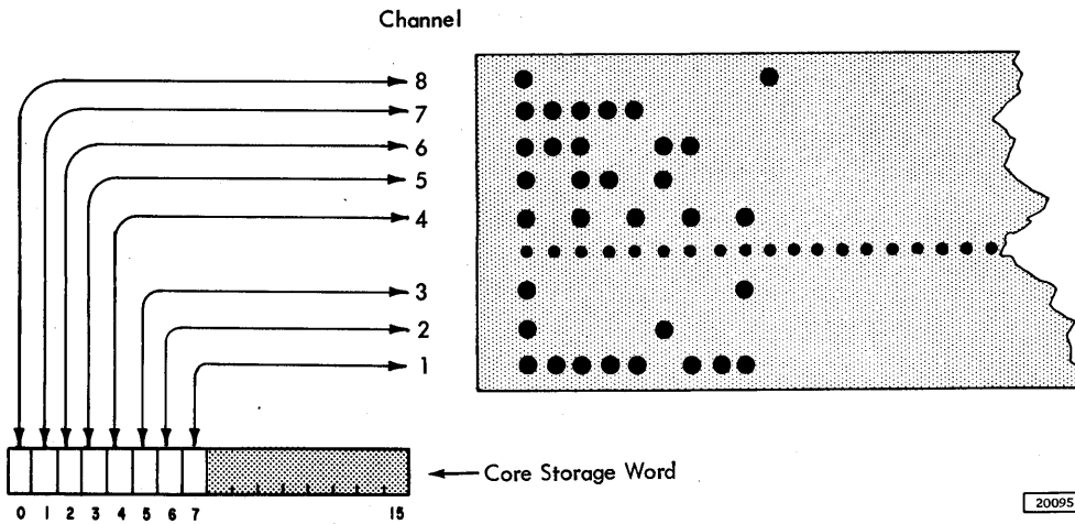
Figure 3-1. 1134/1055 Character Format
