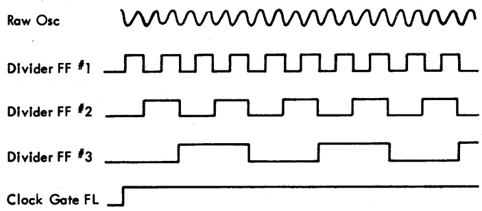
Figure 6-9. Clock Drive
