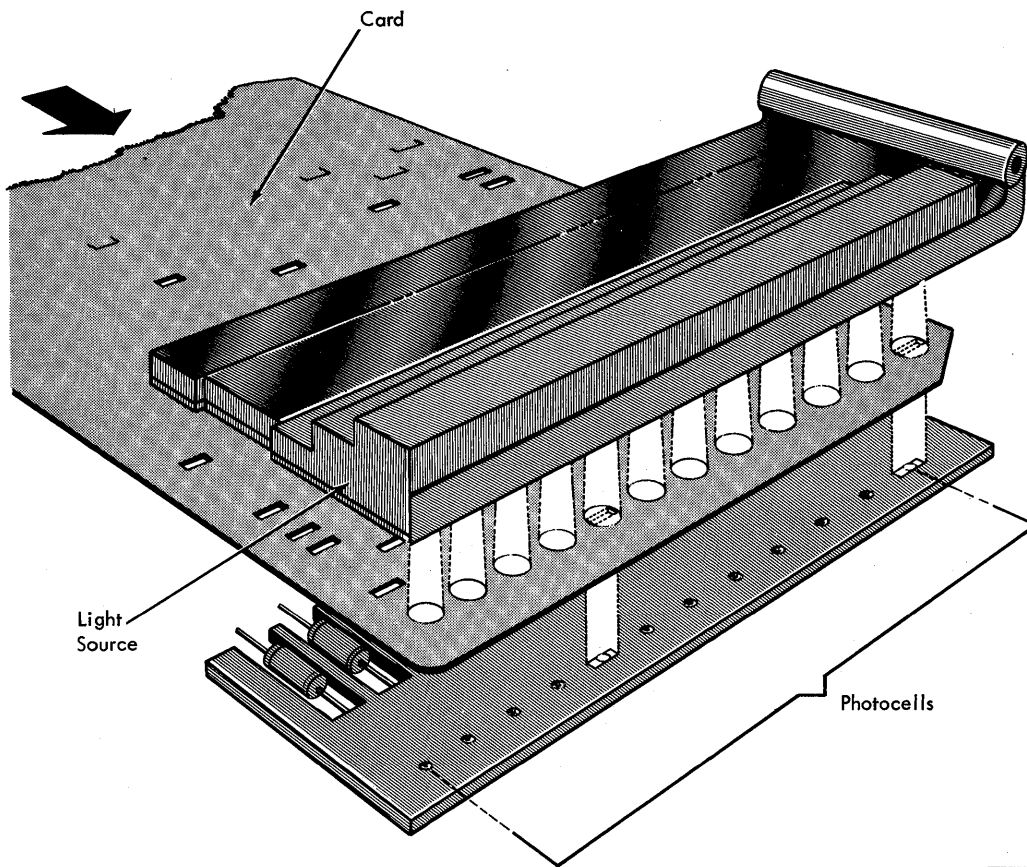
Figure 7-3. Photocell Reading
