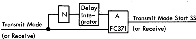
Figure 6-11. Start Singleshots
