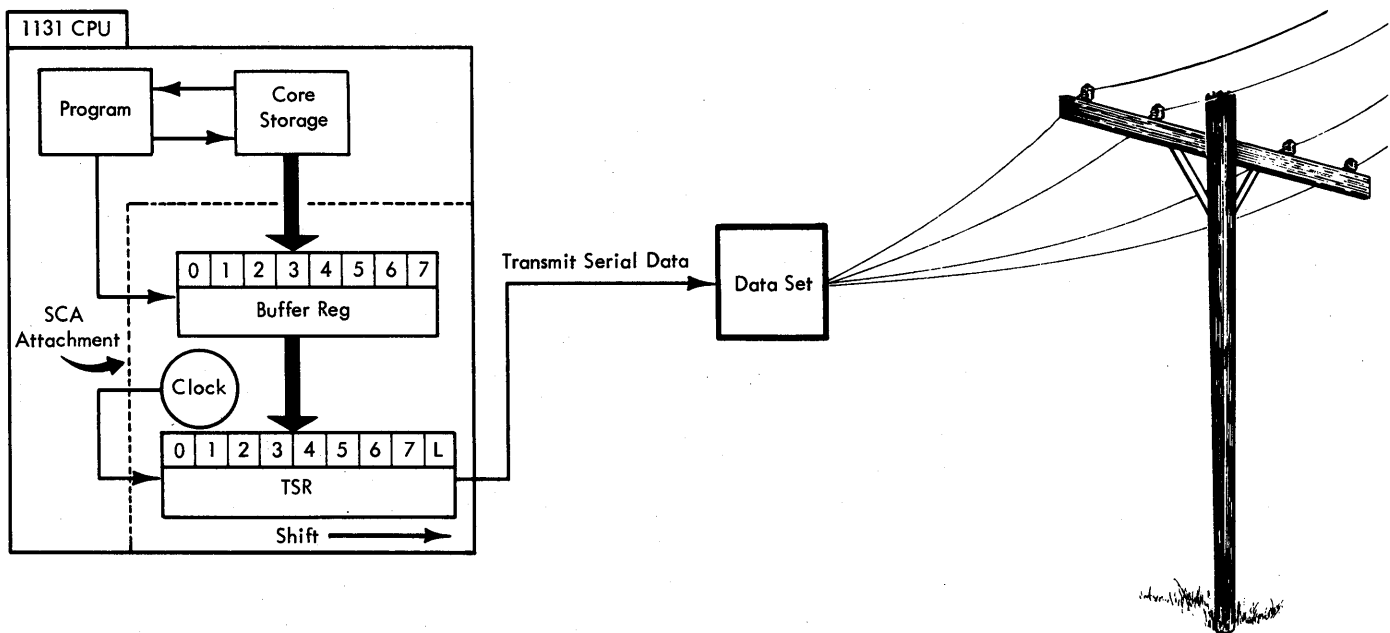
Figure 6-5. Transmit Operation
