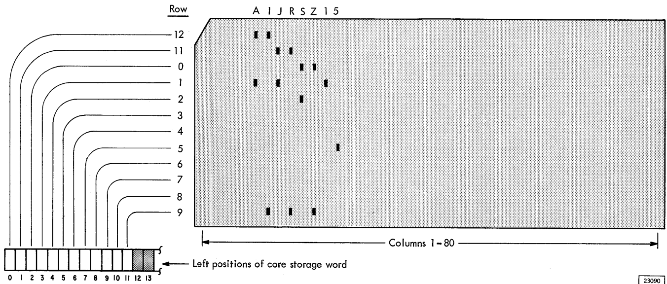
Figure 7-4. Card Code
