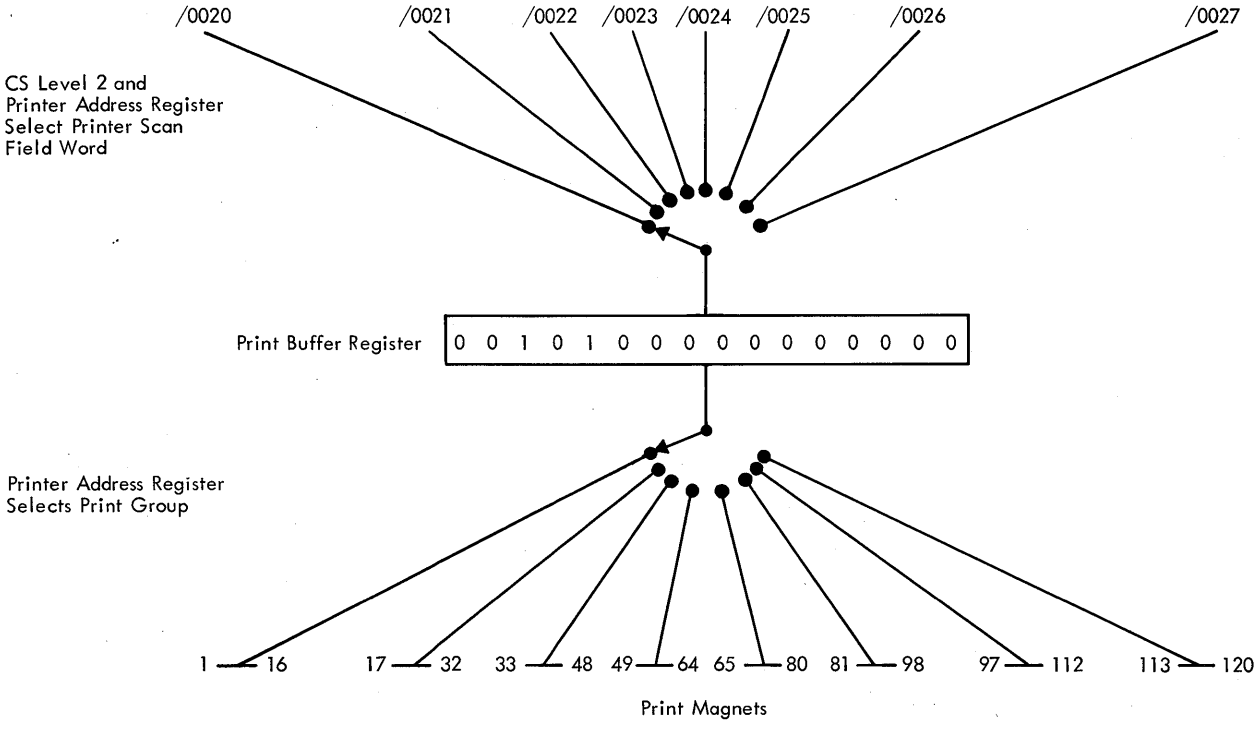
Figure 1-3. Print Operation
