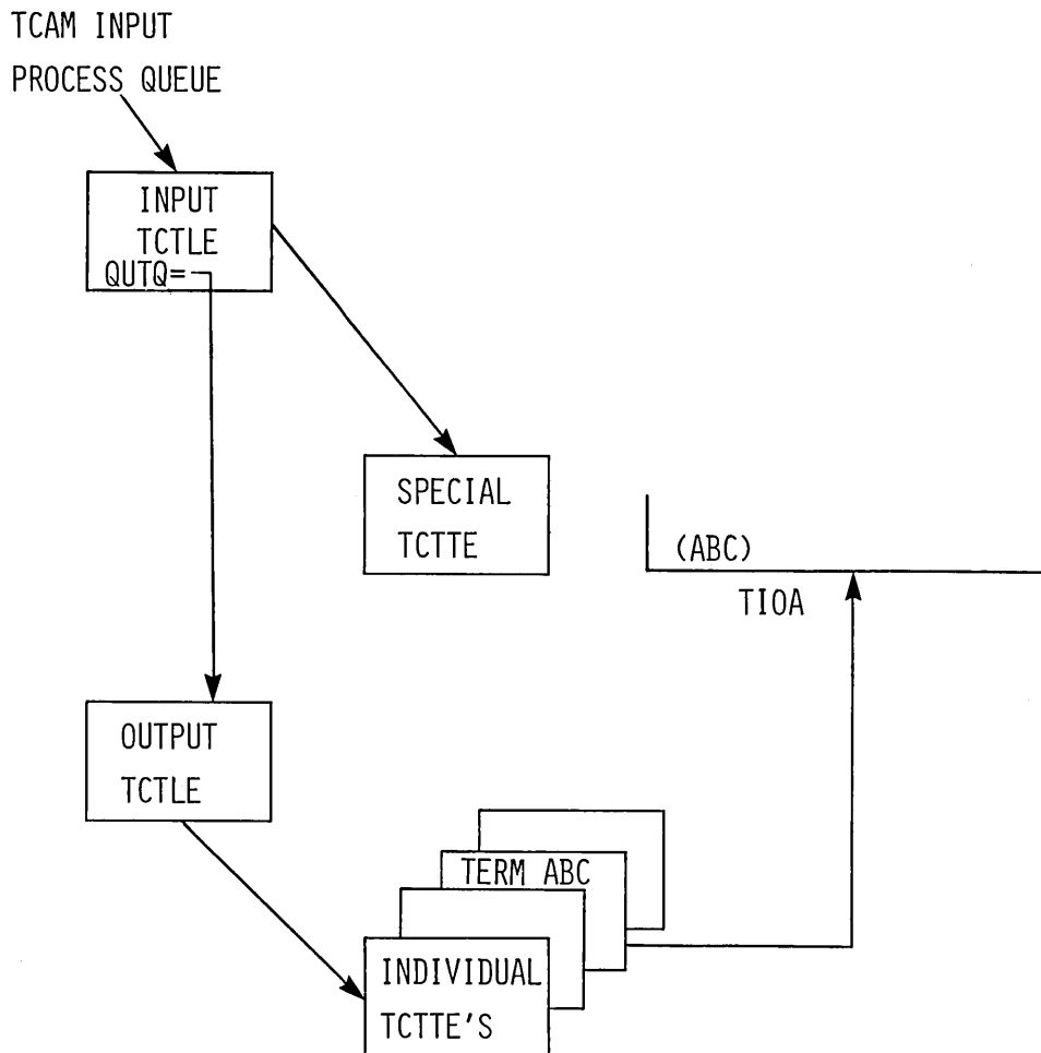
Figure 13. After TCAM read CICS attaches TIOA to corresponding TCTTE
