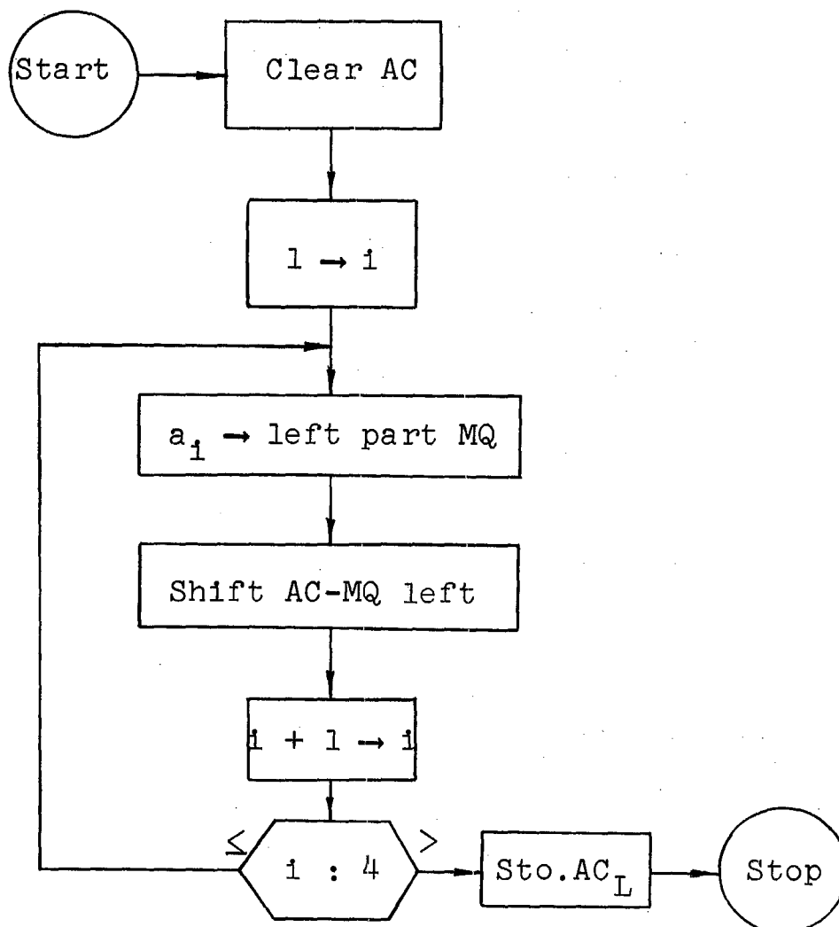
Fig. 12-1. Flowchart for packing routine.
