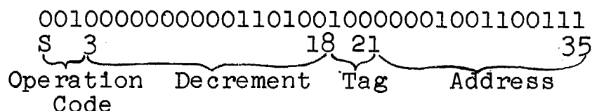
Fig. 8.2 Format of certain indexing instructions
