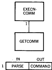
Figure 4 Control-coupled modules
