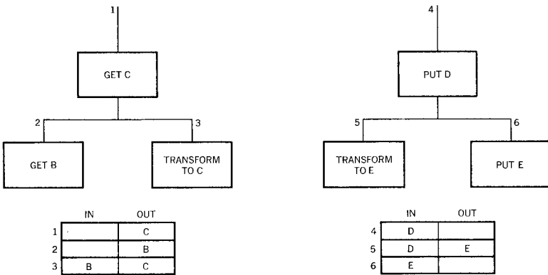
Figure 13 Lower levels
