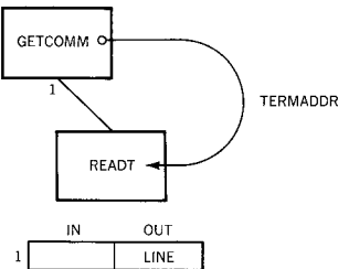
Figure 2 Module connections
