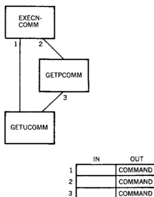
Figure 5 Simplified coupling
