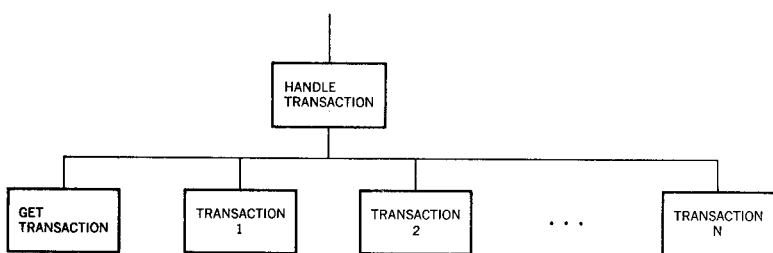
Figure 9 Transaction structure
