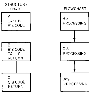
Figure 7 Structure chart compared to flowchart
