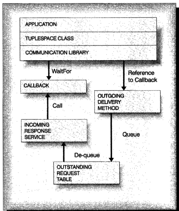
Figure 4 Client communication architecture
