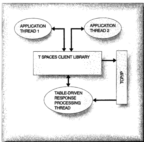
Figure 3 Client architecture
