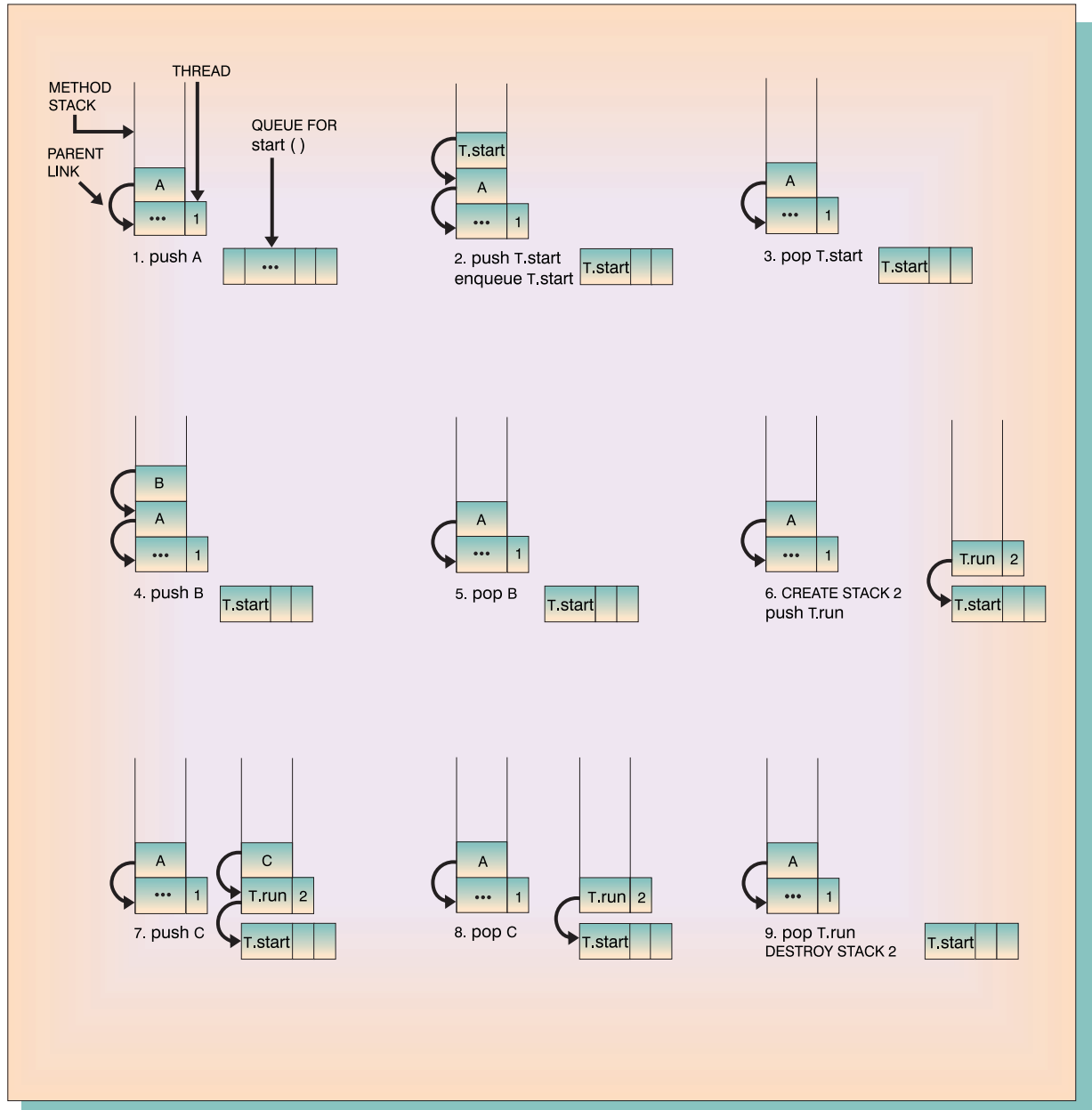
Figure 7 Application of the stack-based algorithm to handle the start and run methods used to initiate a new thread
