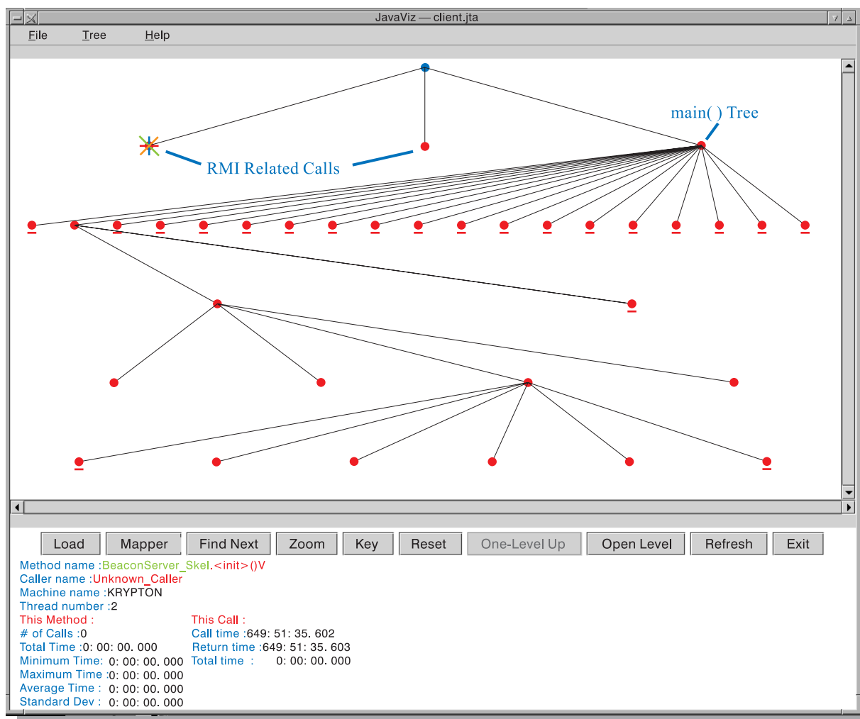
Figure 13 Portion of the call graph for Server 1
