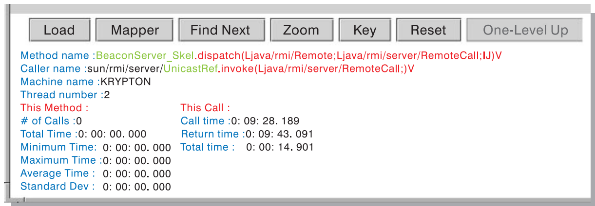
Figure 12 Data on the BeaconServer_Skel.dispatch() method call in the node information window of the visualizer
