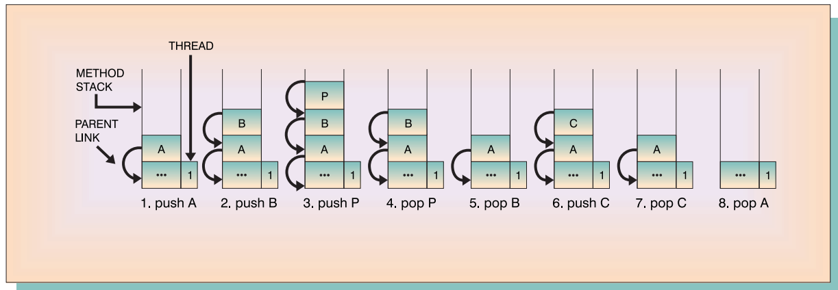
Figure 6 Application of the stack-based algorithm for tree generation to the example in Figure 5
