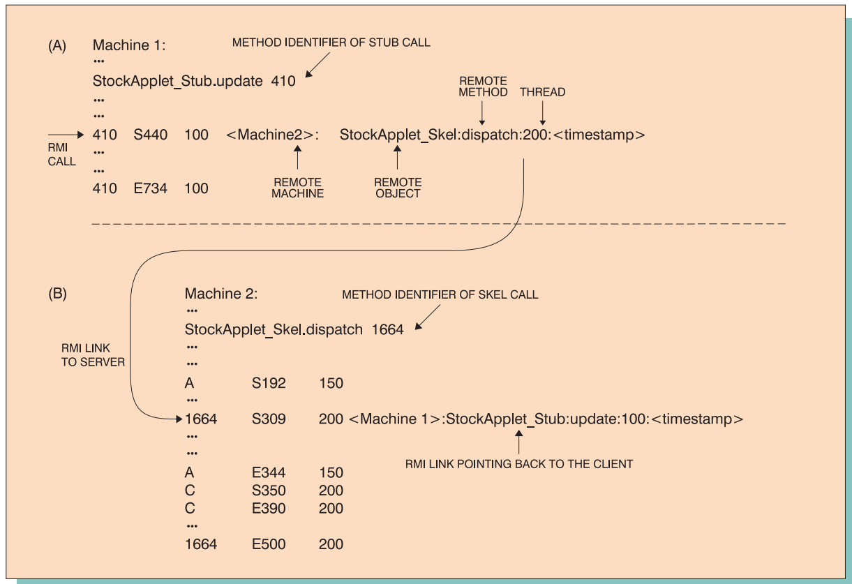
Figure 8 (A) The .mrg file entries for a client running on Machine 1; (B) the .mrg file entries for a server running on Machine 2
