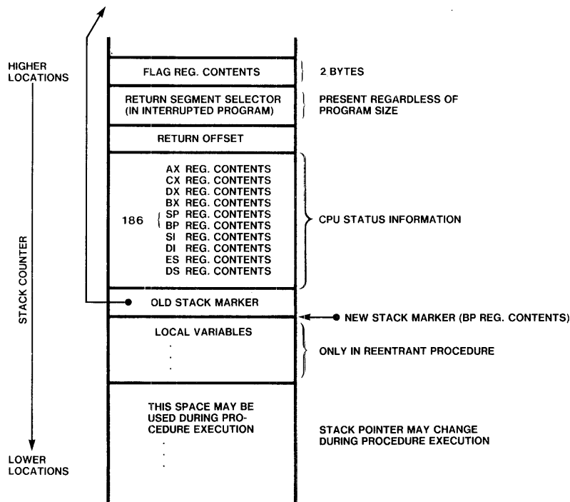
Figure G-2. Stack Layout During Execution of an Interrupt Procedure Body
