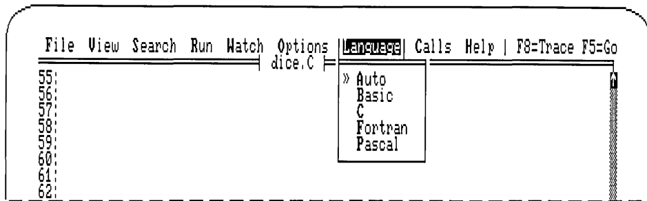
Figure 2.8 The Language Menu
