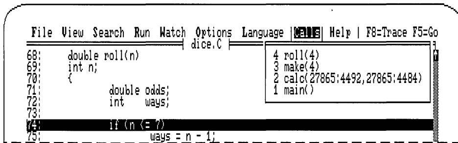
Figure 2.9 The Calls Menu
