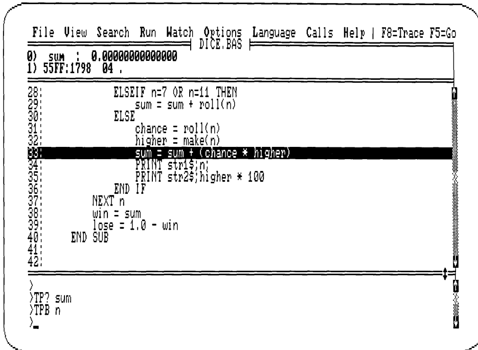
Figure 8.3 Tracepoints in the Watch Window
