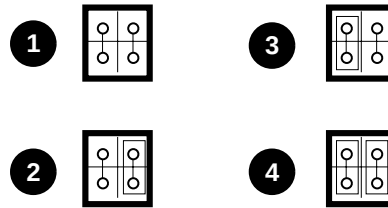
Figure 7-2 Jumper Settings for TRM PWR/TRM ENB Connector
