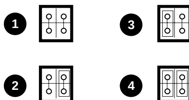
Figure 3-4 Jumper Settings for TRM PWR/TRM ENB Connector
