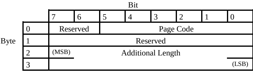
Figure 8-26 Read/Write Compression Ratio Page Header
