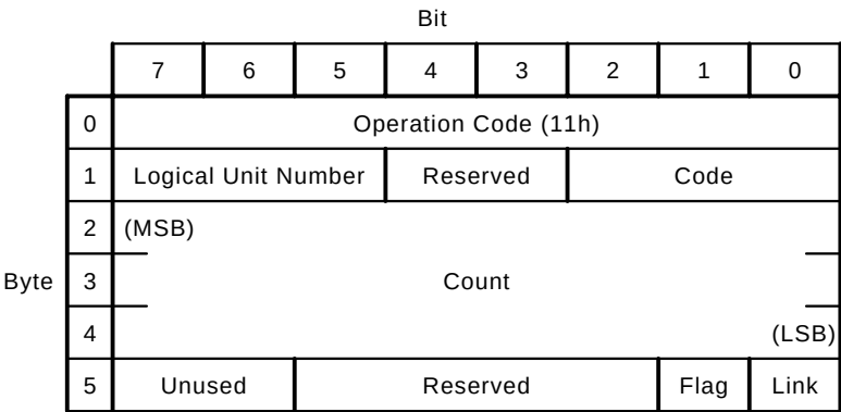
Figure 8-75 SPACE CDB
