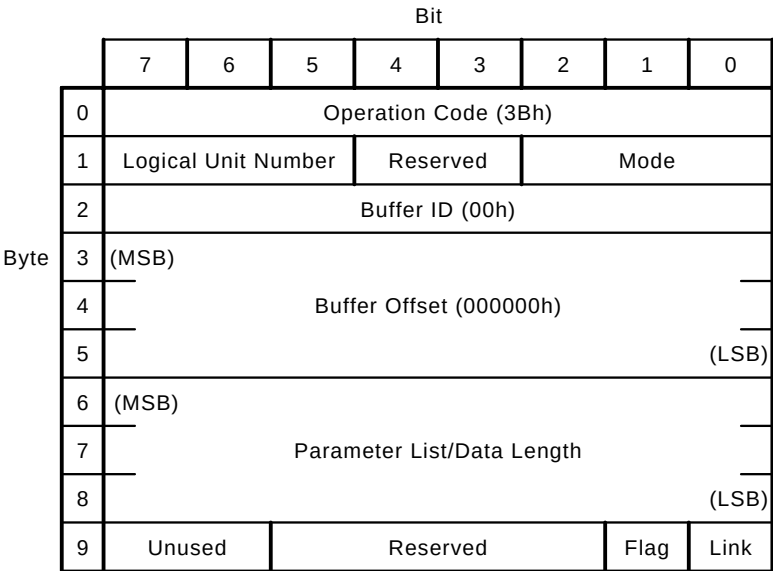
Figure 8-80 WRITE BUFFER CDB
