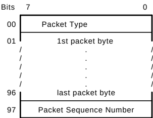
Figure D-1 EEROM Log Area Layout
