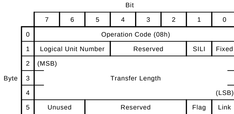
Figure 8-57 READ CDB
