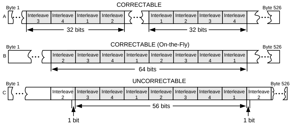
Figure 5-8 Correctable and Uncorrectable Double-Burst Errors
