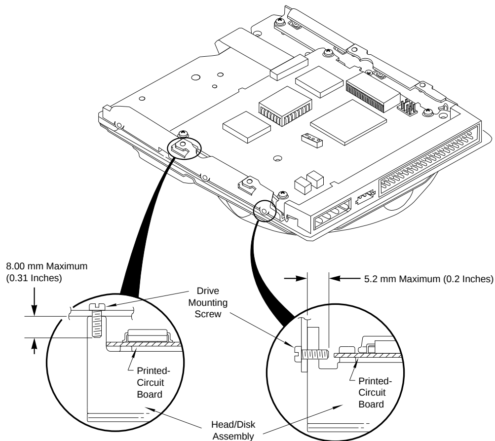
Figure 3-7 Mounting Screw Clearance for Quantum Fireball TM (One-Disk) Drive
