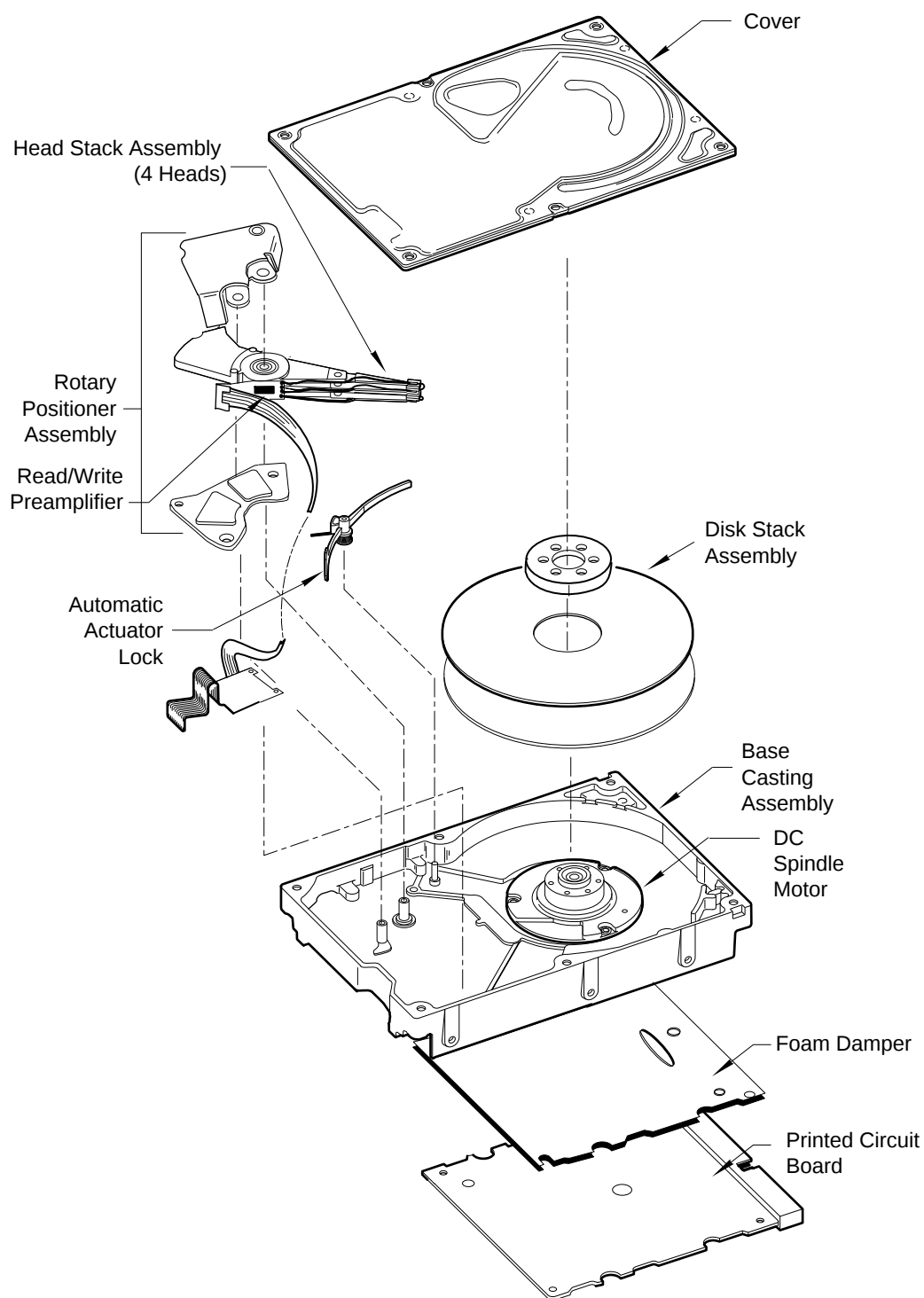
Figure 5-1 Quantum Fireball TM (Two-Disk) Drive Exploded View
