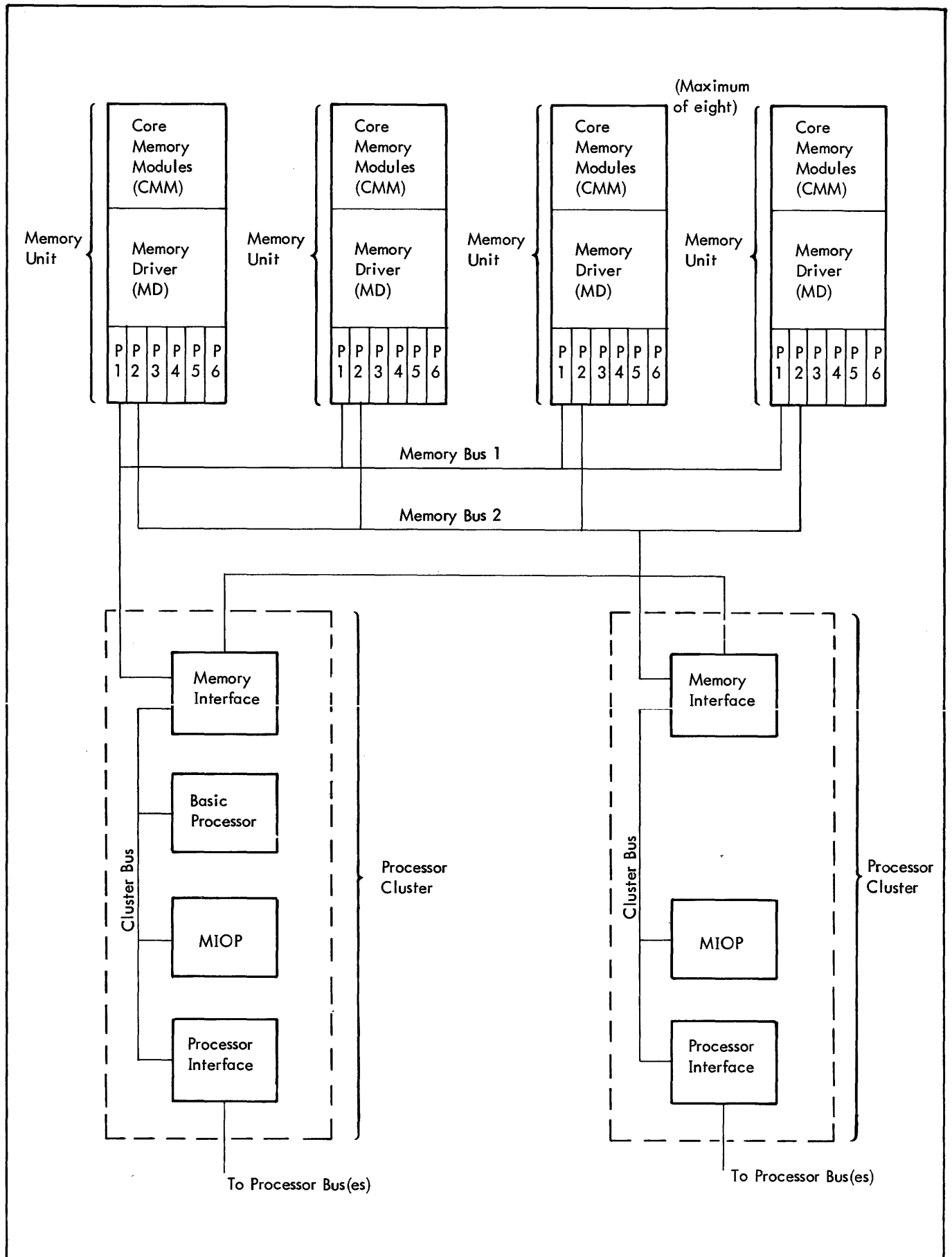
Figure 4. Main Memory
