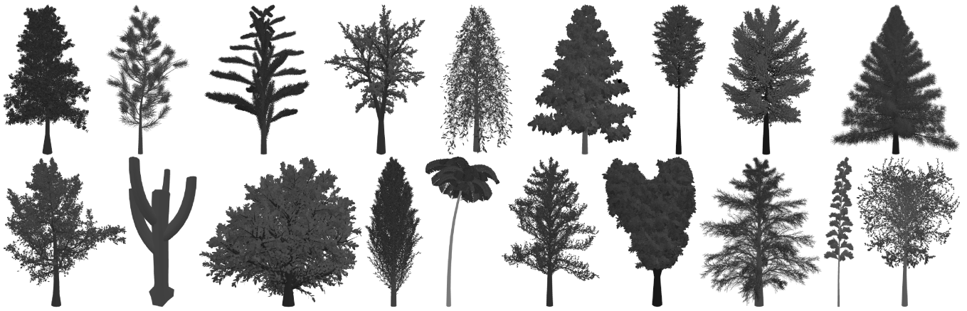
Figure 8: Nineteen trees that were used as initial landmarks for the parametric tree space.
