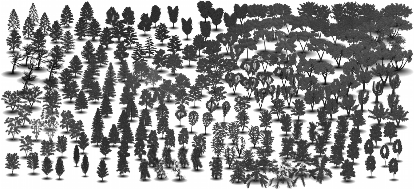
Figure 1: A section of a parametric space of trees.
