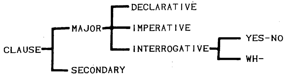
Figure 2.12. Simple system network for the clause.
