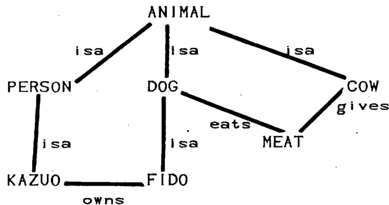
Figure 3.5. A semantic net.
