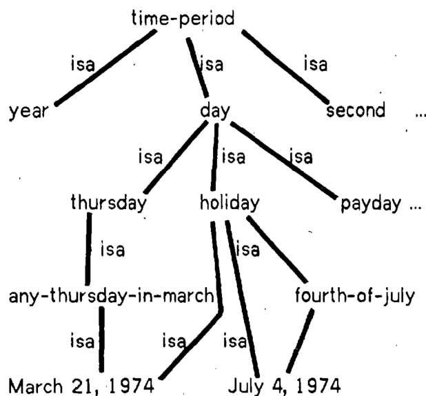
Figure 4.4. A generalization hierarchy for time periods.
