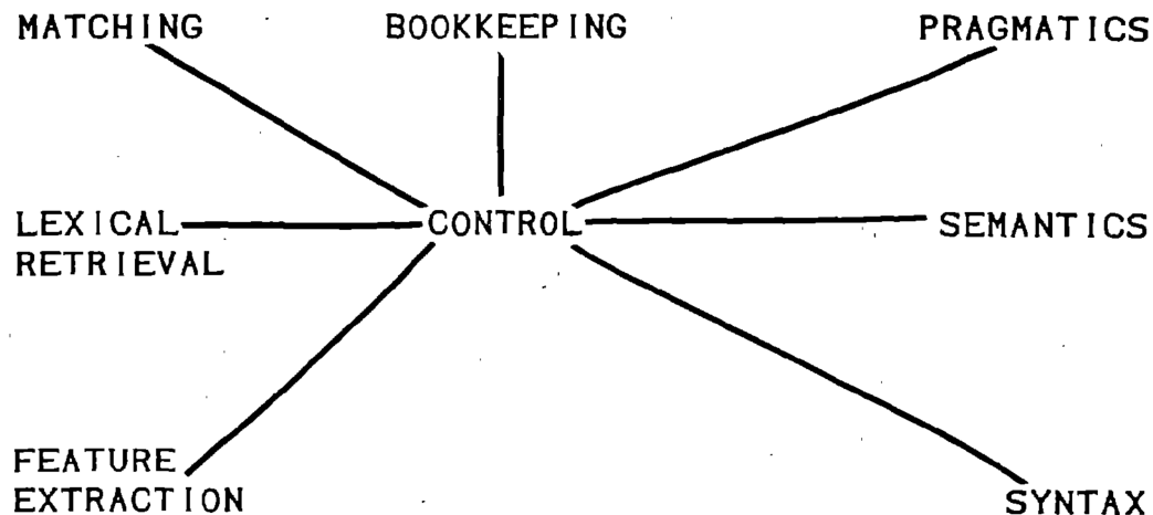
Figure 1.6. Heterarchical system organization.
