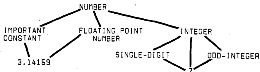
Figure 4.5. Part of a generalization hierarchy for numbers
