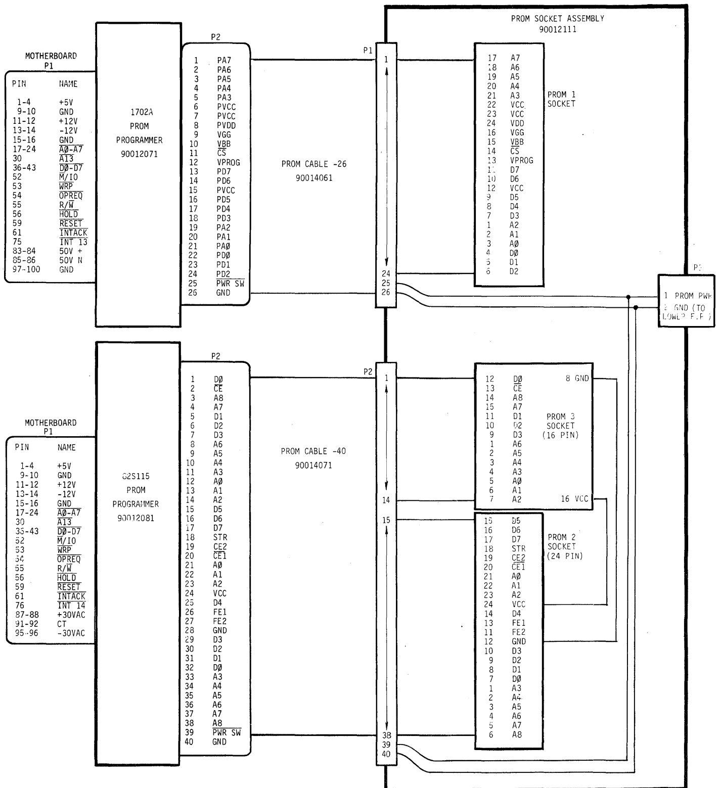
FIGURE 8-11 PROM PROGRAMMER INTERCONNECT
