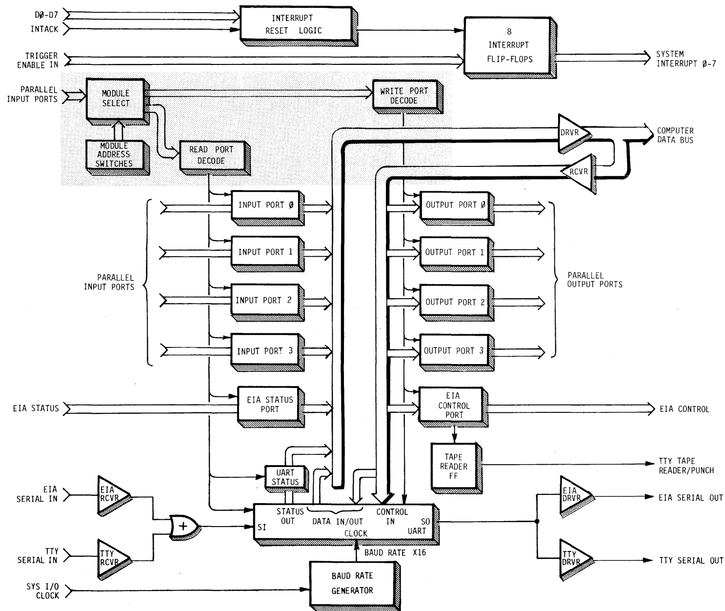
FIGURE 7-4 MODULE AND PORT ADDRESS CONTROL
