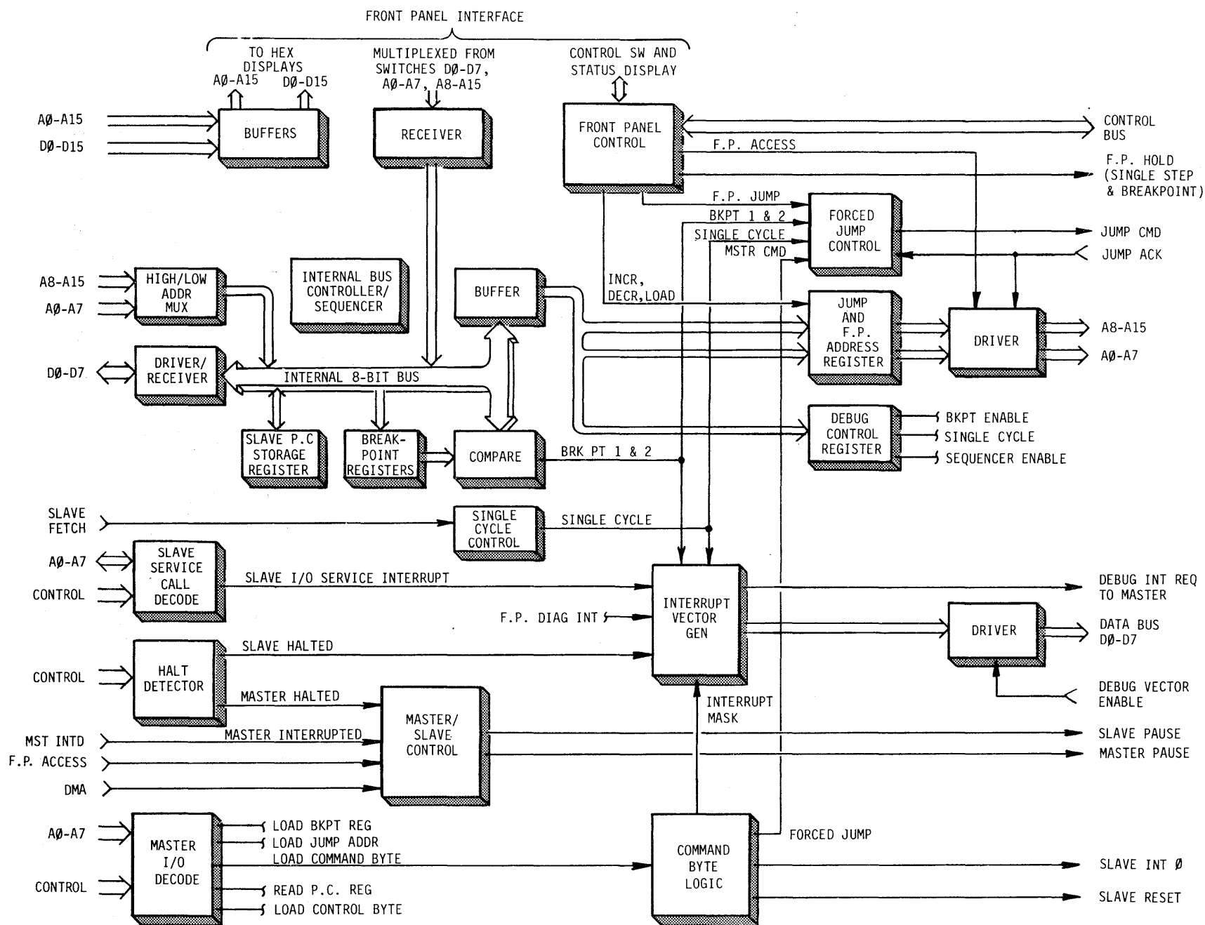
FIGURE 4-1 DEBUG AND FRONT PANEL I/O BLOCK DIAGRAM
