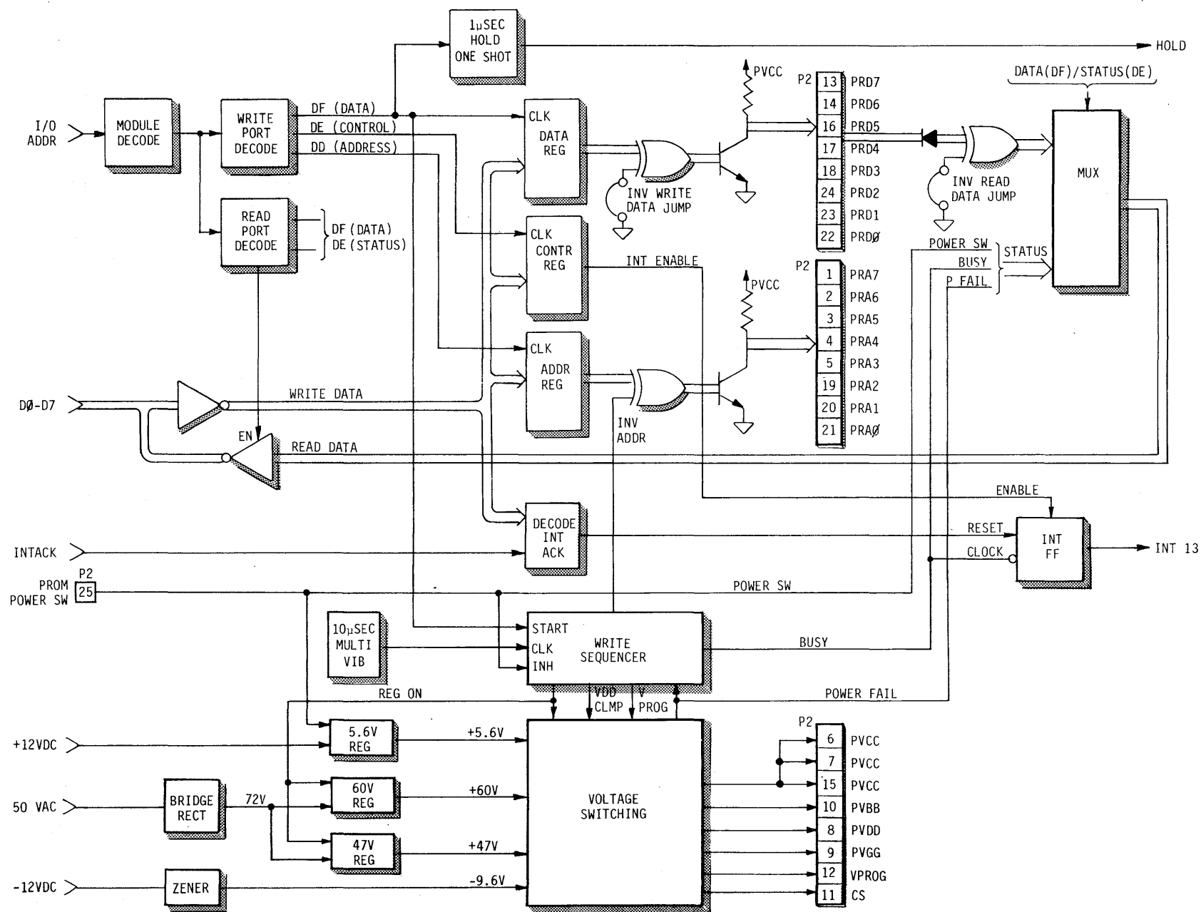
FIGURE 8-3 1702A PROM PROGRAMMER BLOCK DIAGRAM
