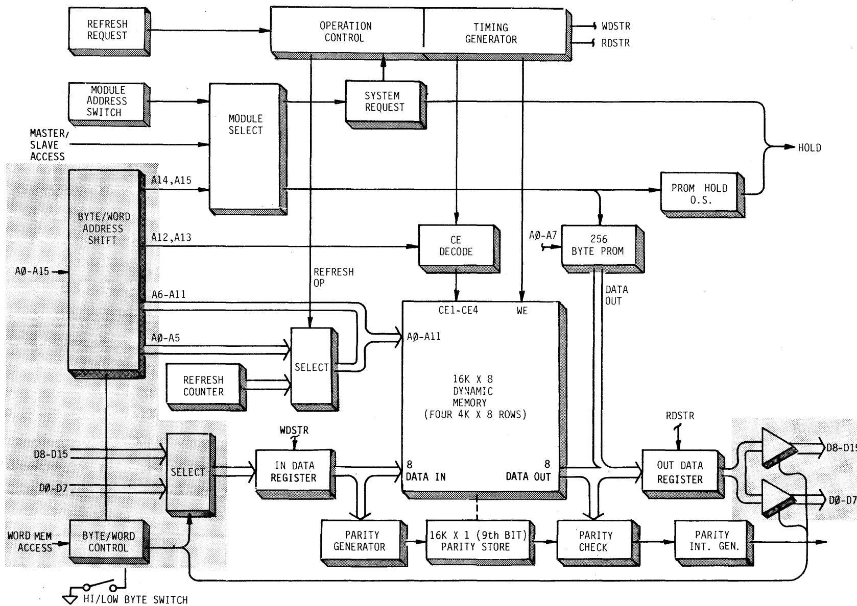
FIGURE 6-5 BYTE WORD CONTROL
