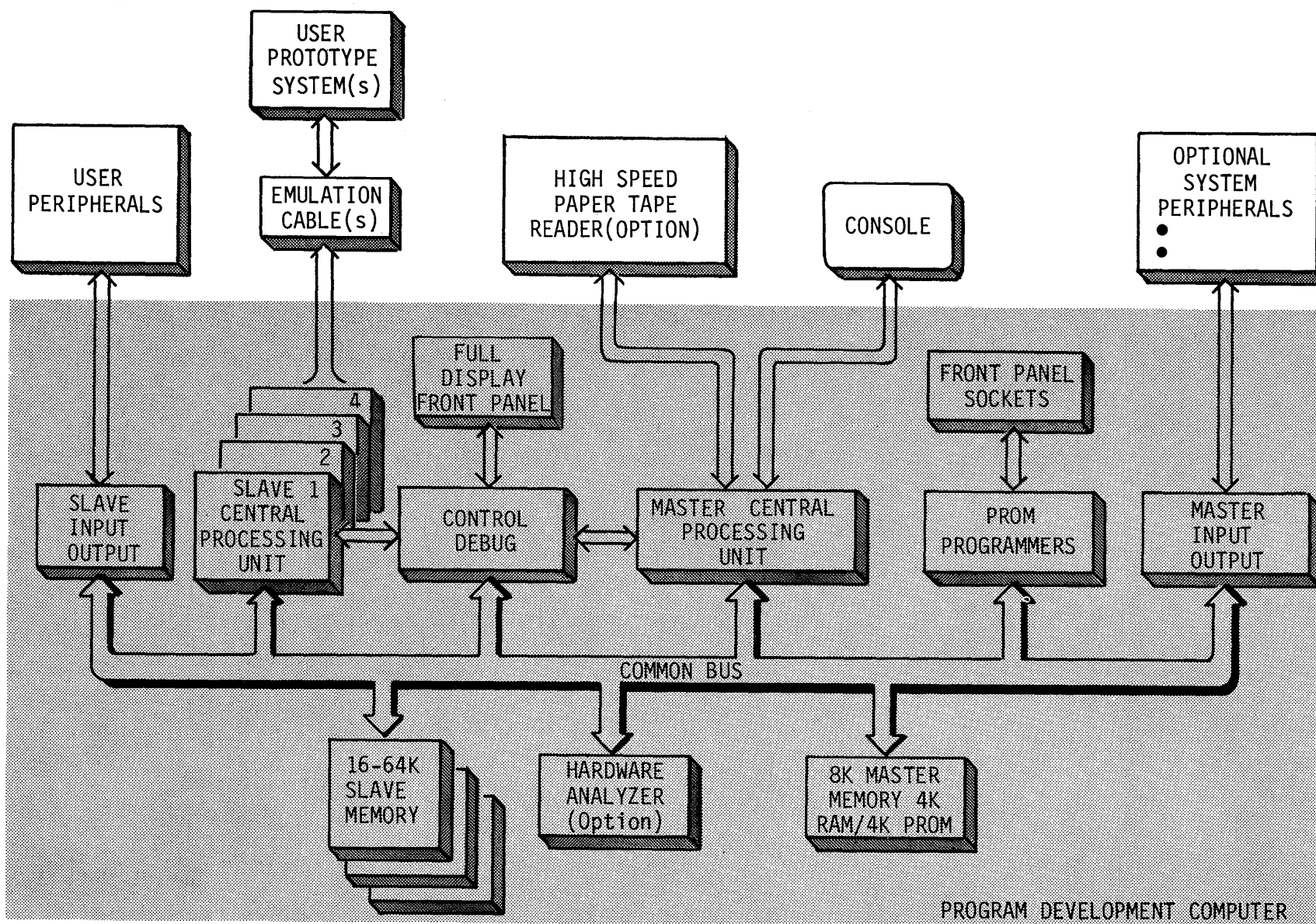
FIGURE 1-2 THE UNIVERSAL EMULATOR SYSTEM
