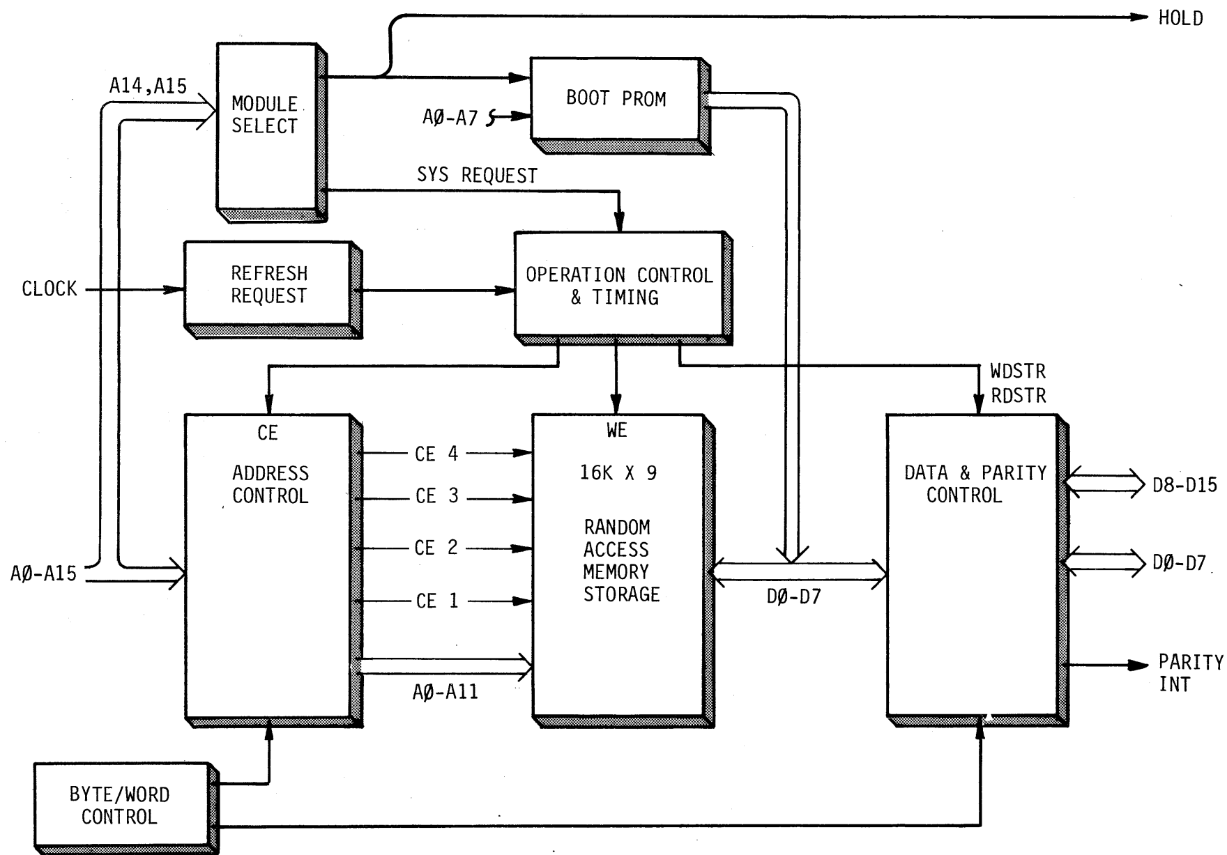
FIGURE 6-1 16K DYNAMIC RAM SIMPLIFIED BLOCK DIAGRAM
