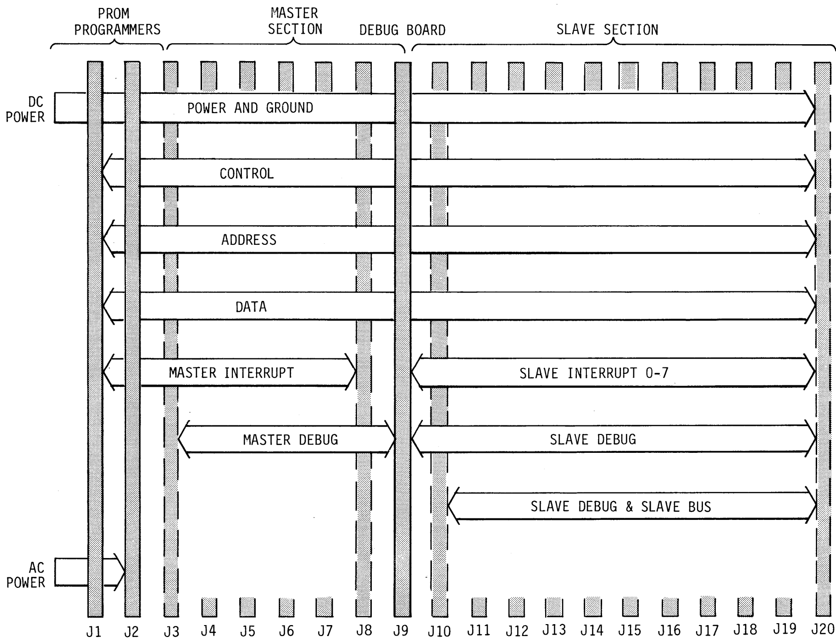
FIGURE 9-1 BUS STRUCTURE
