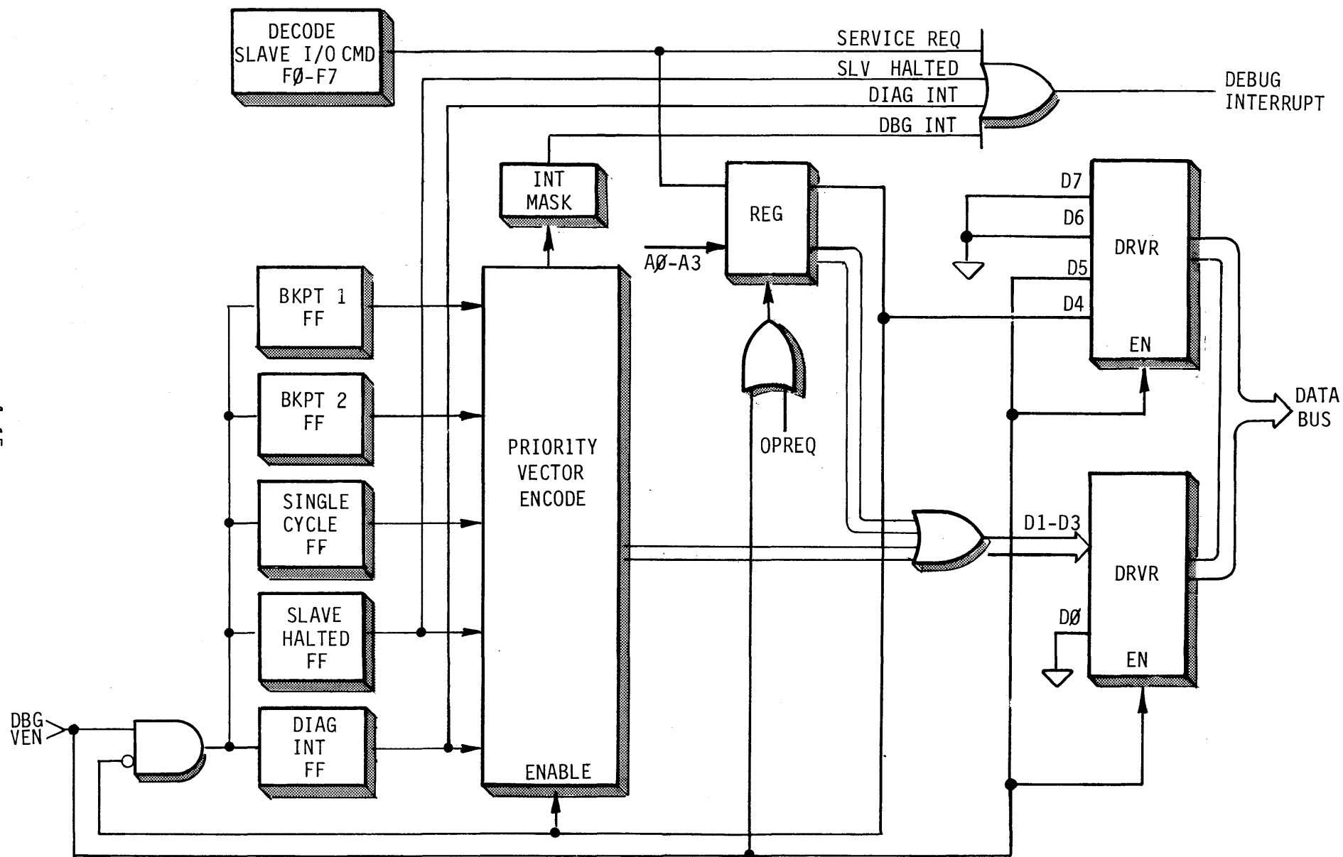
FIGURE 4-9 DEBUG INTERRUPT LOGIC
