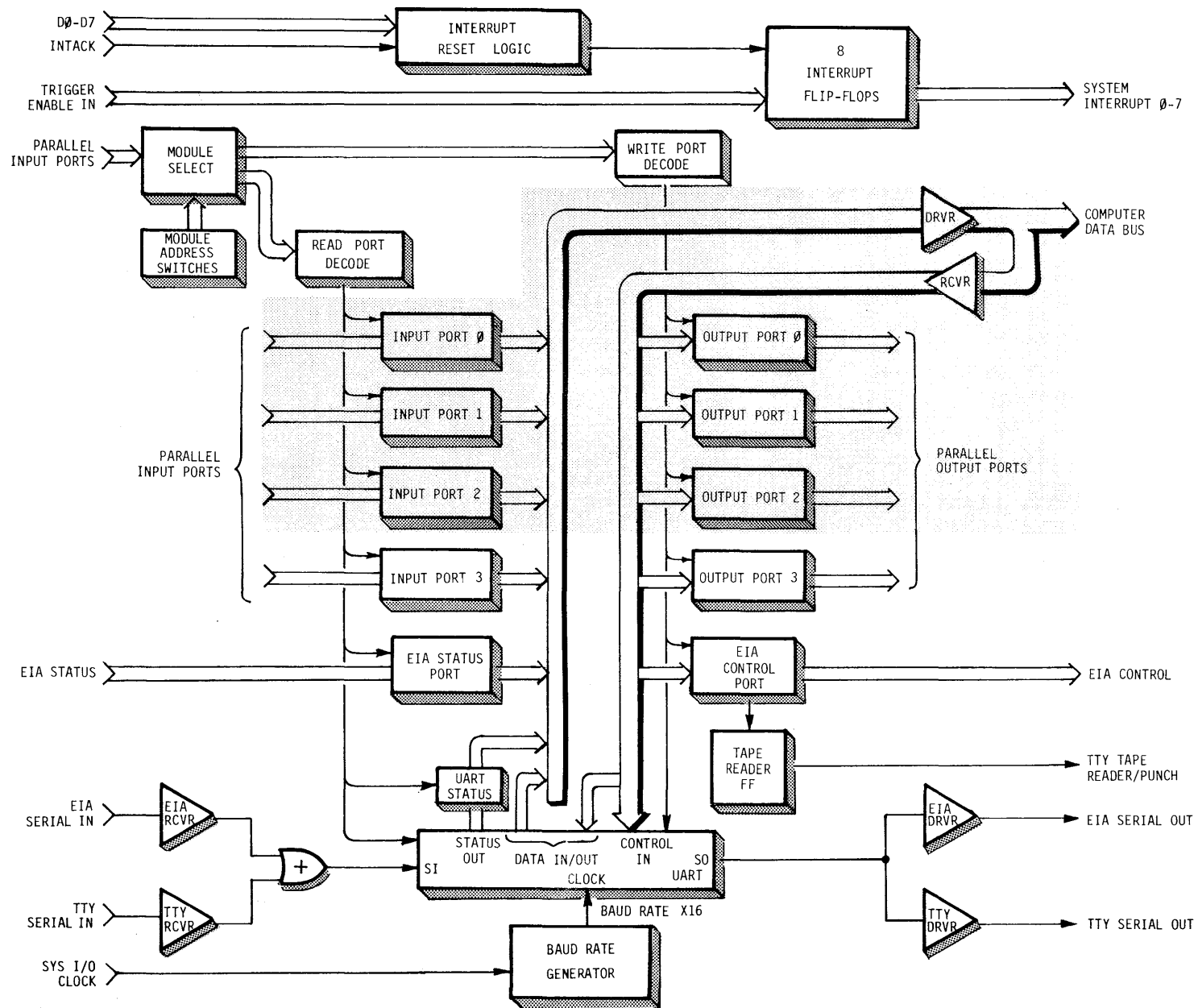
FIGURE 7-5 PARALLEL INPUT-OUTPUT PORTS
