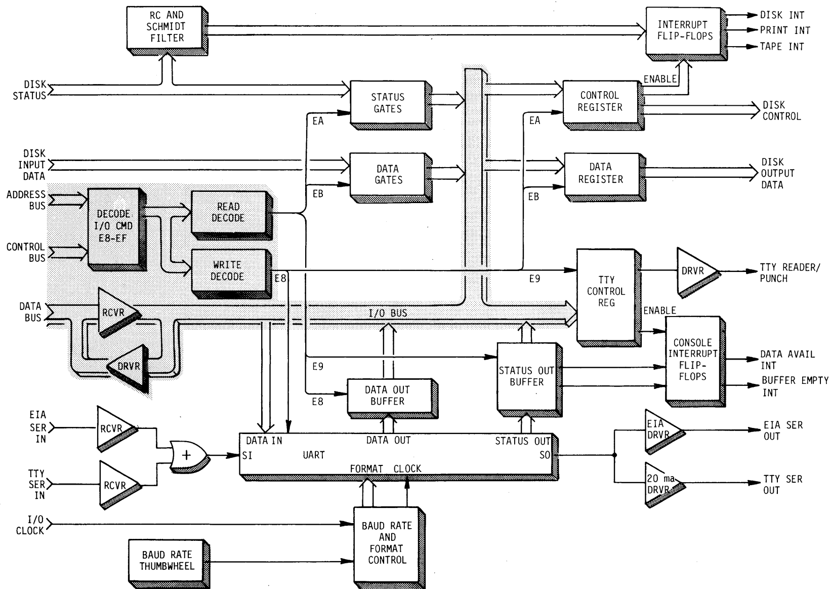
FIGURE 3-9 MASTER CPU I/O DECODING BLOCK DIAGRAM
