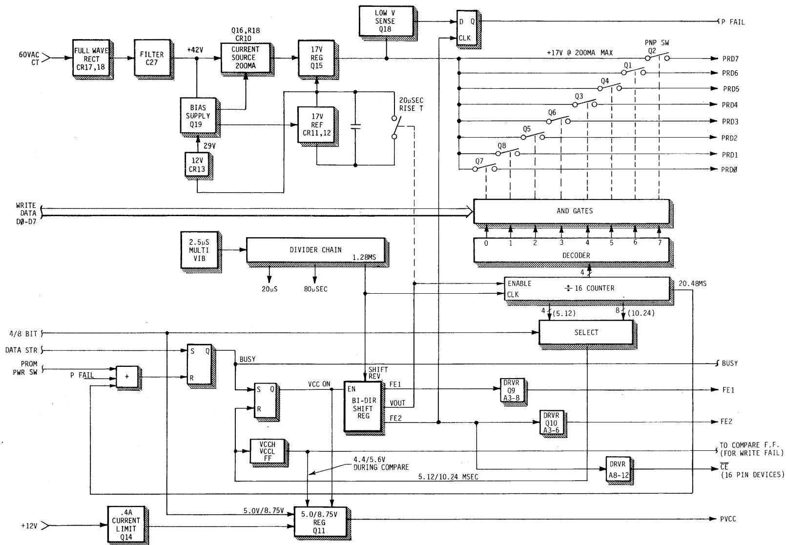
FIGURE 8-8 82S115 PROM PROGRAMMER WRITE WAVEFORM GENERATOR
