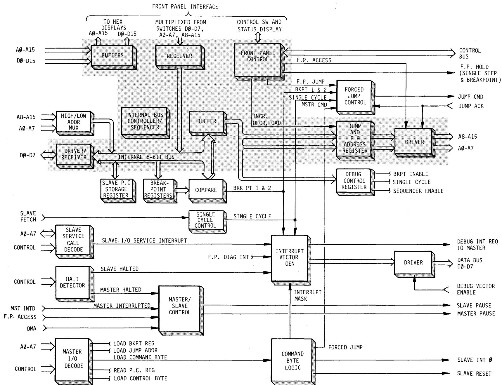
FIGURE 4-5 FRONT PANEL INTERFACE
