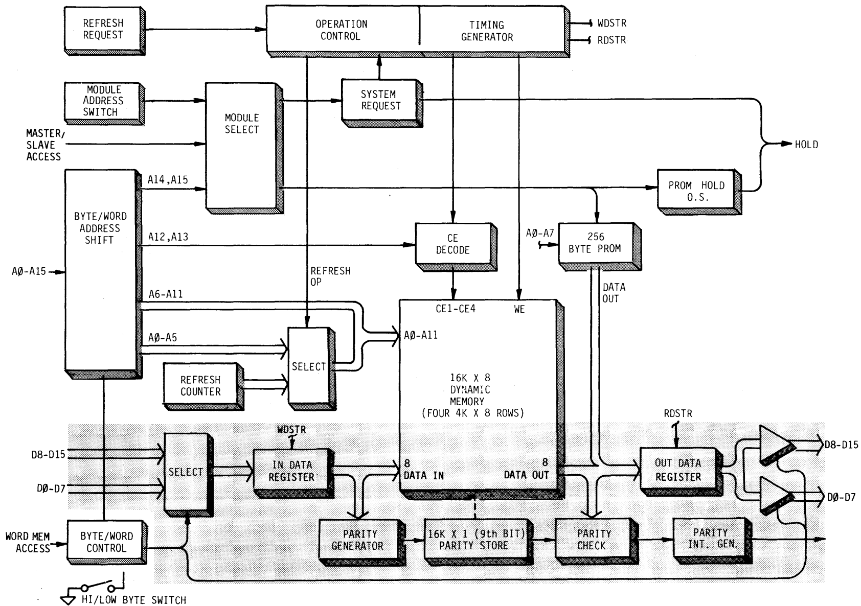
FIGURE 6-8 DATA AND PARITY CONTROLFIGURE
