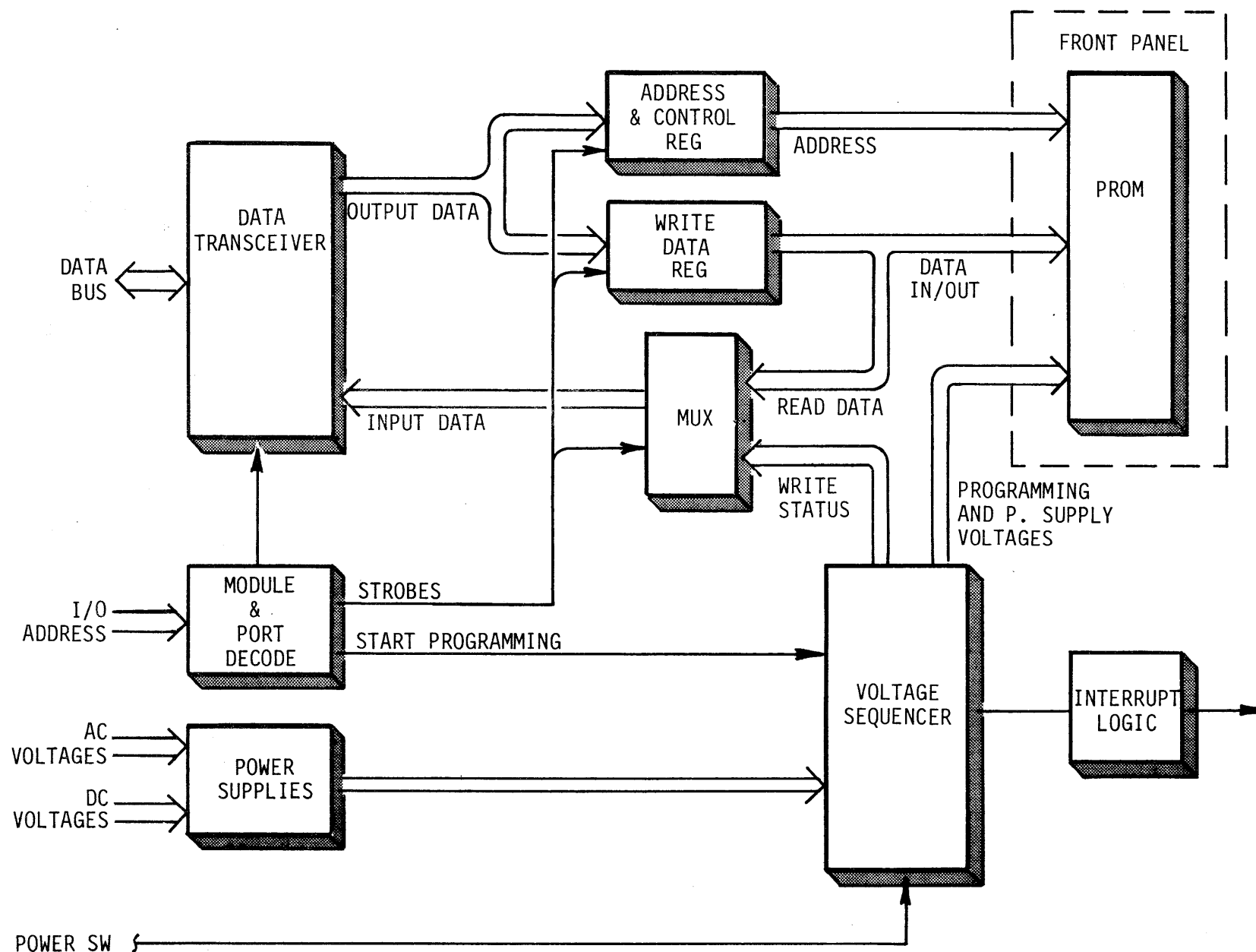
FIGURE 8-1 SIMPLIFIED PROM PROGRAMMER BLOCK DIAGRAM
