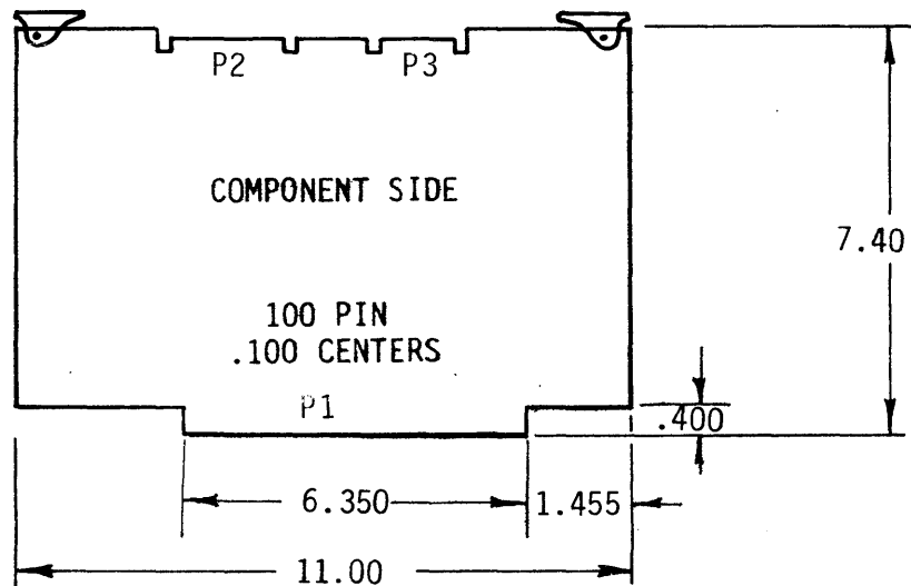
FIGURE 3-13 MASTER CPU ENVIRONMENTAL, POWER AND PHYSICAL REQUIREMENTS
