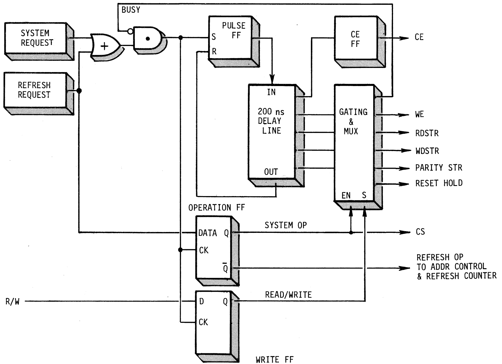
FIGURE 6-12 OPERATION CONTROL AND TIMING BLOCK DIAGRAM
