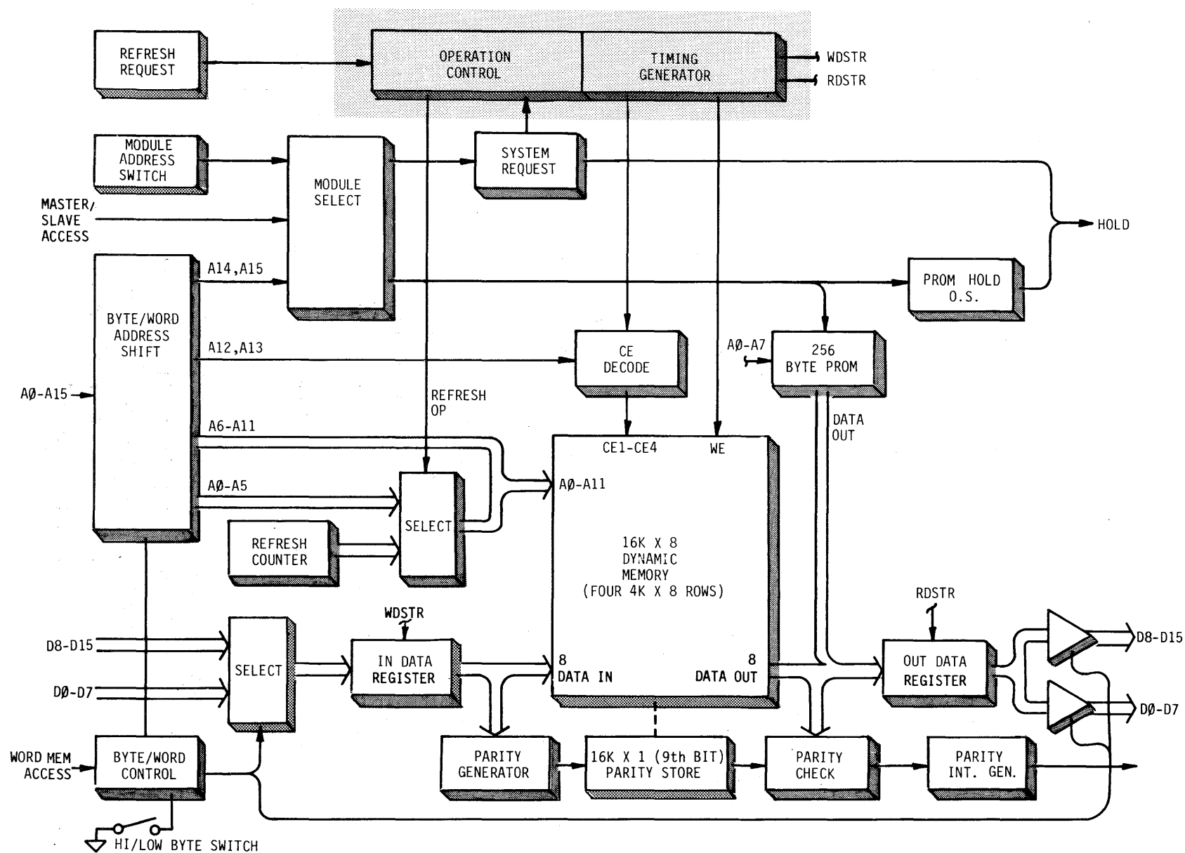
FIGURE 6-11 OPERATION CONTROL AND TIMING
