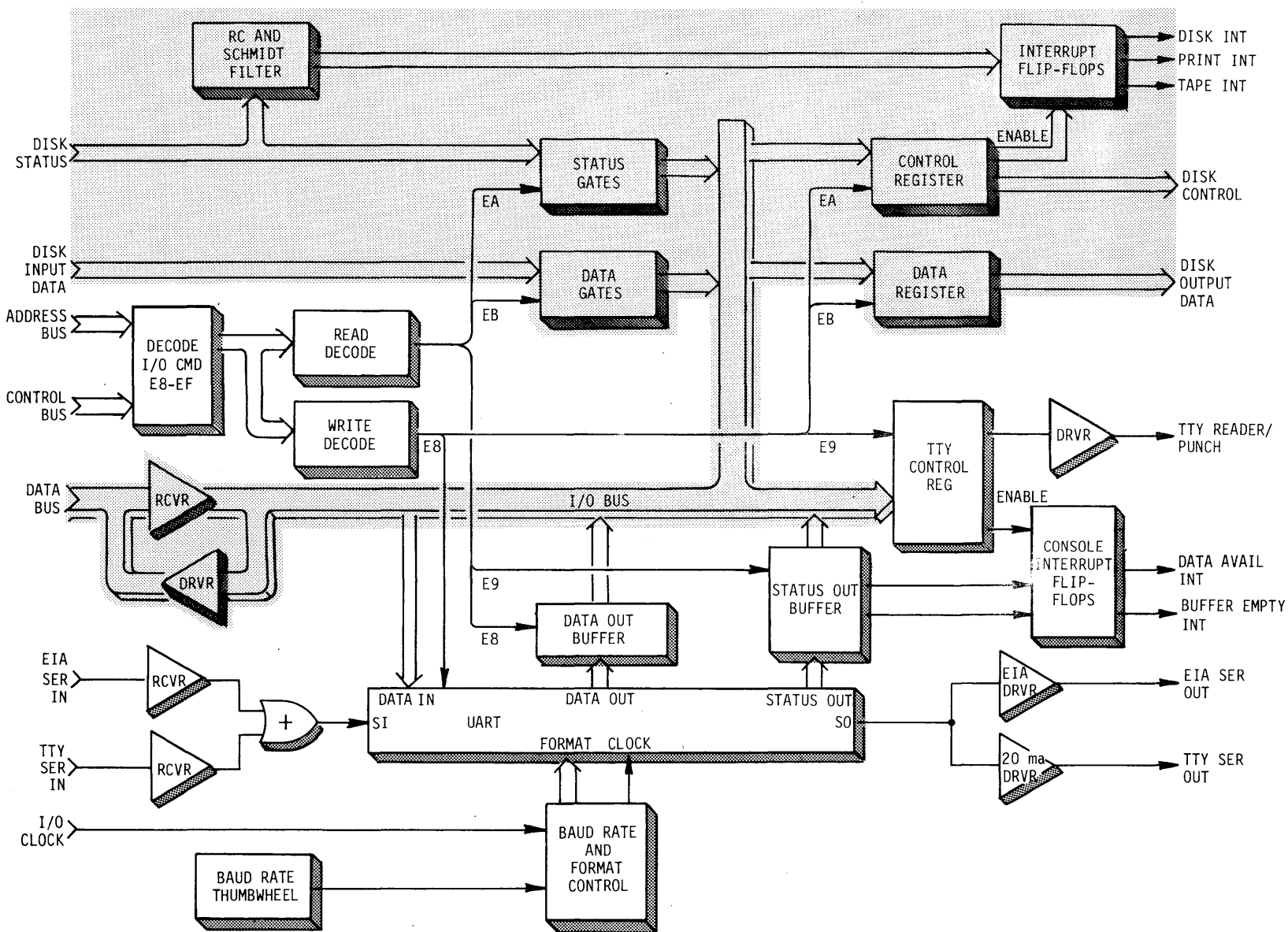
FIGURE 3-7 MASTER CPU DISK I/O BLOCK DIAGRAM
