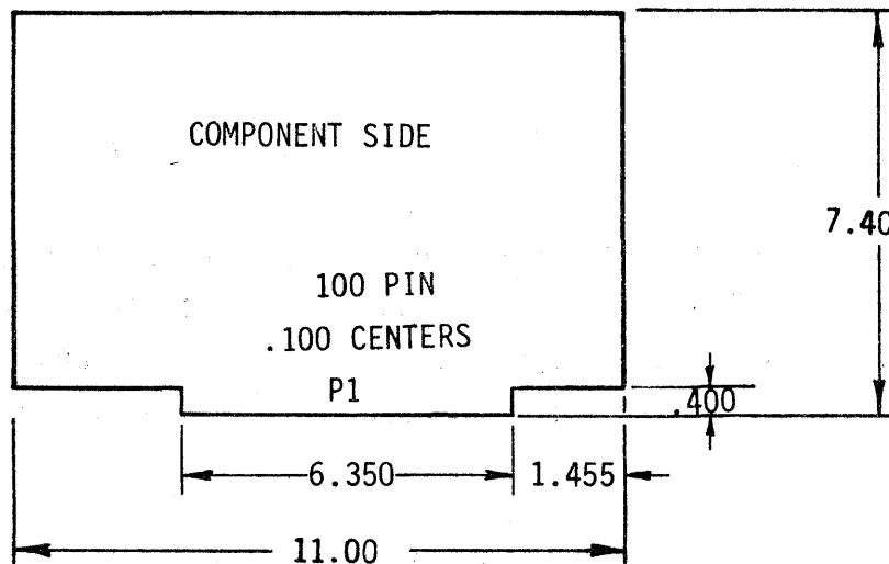
FIGURE 6-14 16K DYNAMIC RAM ENVIRONMENTAL, POWER AND PHYSICAL REQUIREMENTS
