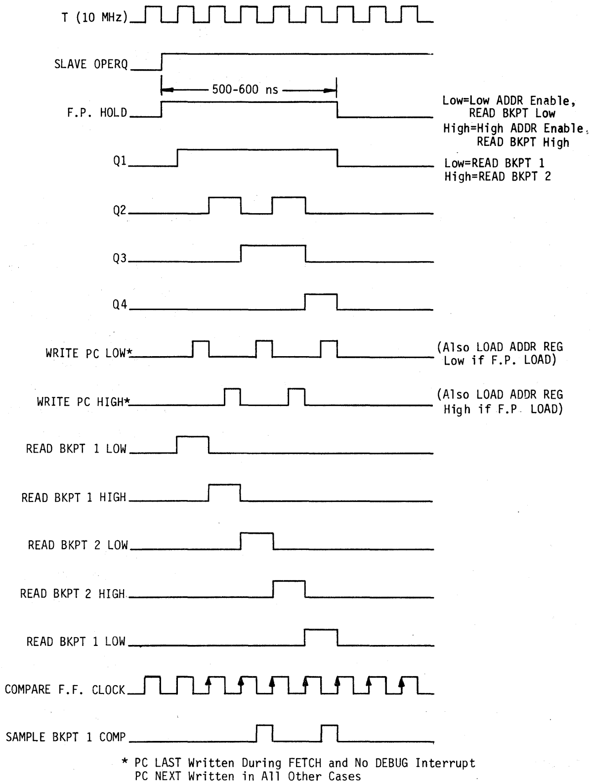
FIGURE 4-11 SEQUENCER TIMING
