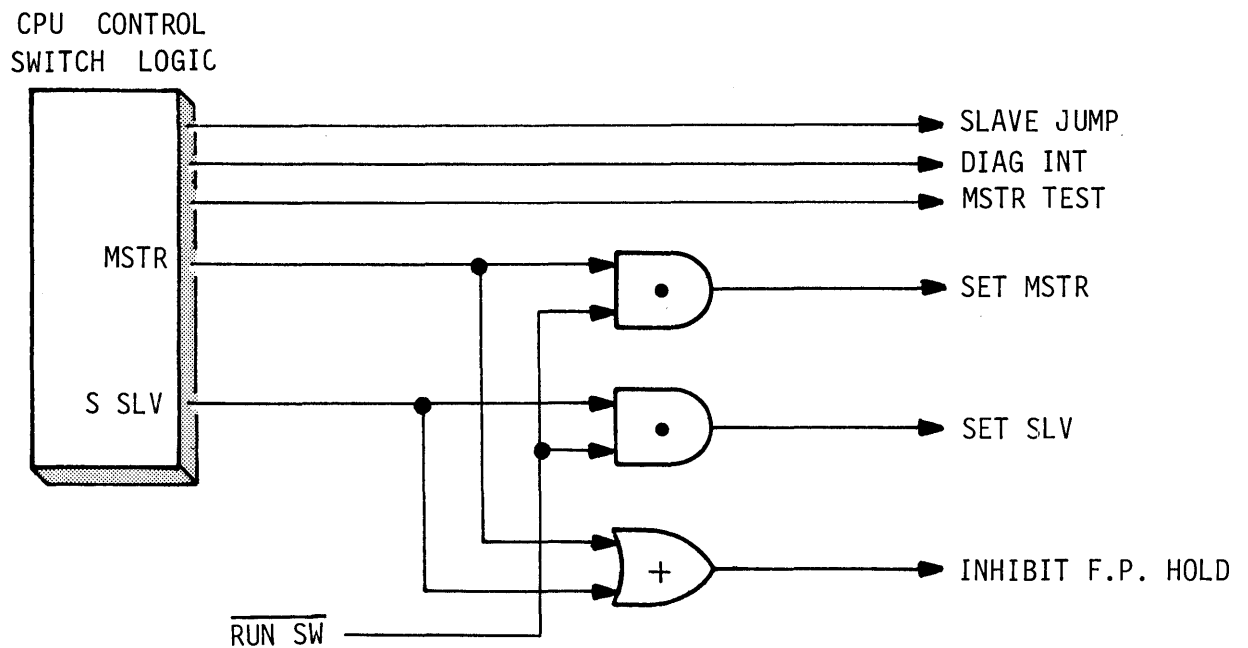
FIGURE 10-5 CPU CONTROL
