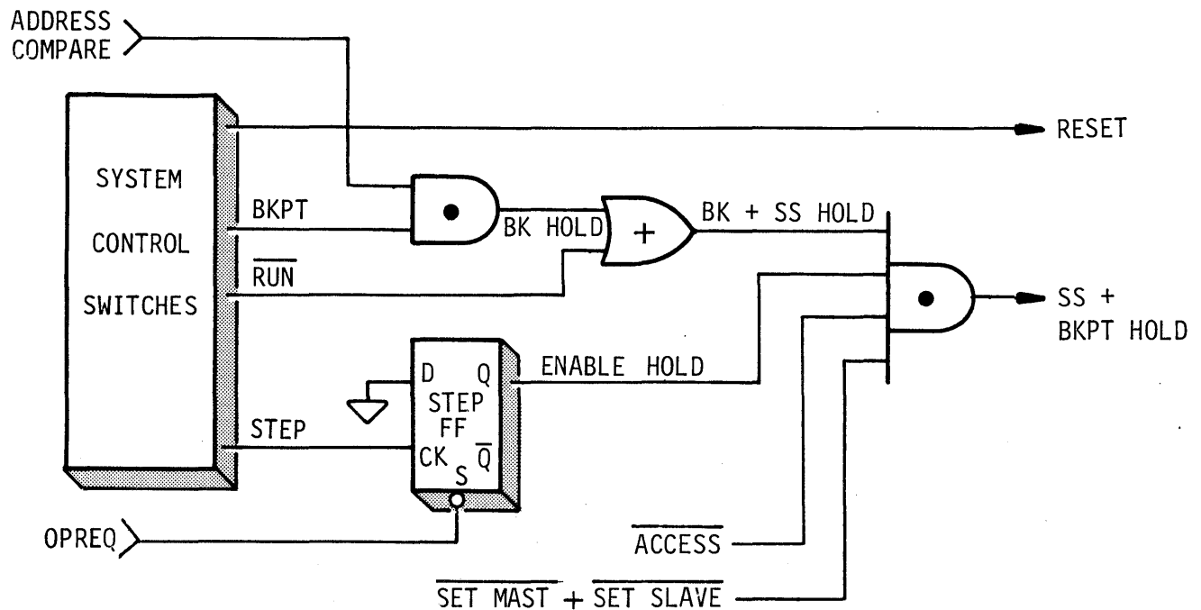
FIGURE 10-6 SYSTEM CONTROL LOGIC
