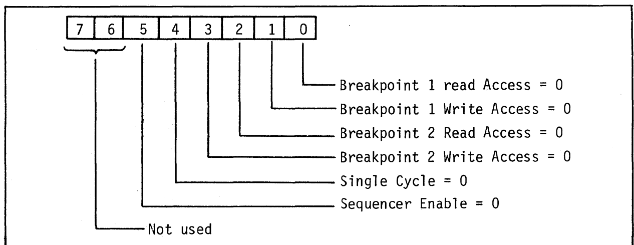
FIGURE 4-8c DEBUG CONTROL BYTE FORMAT
