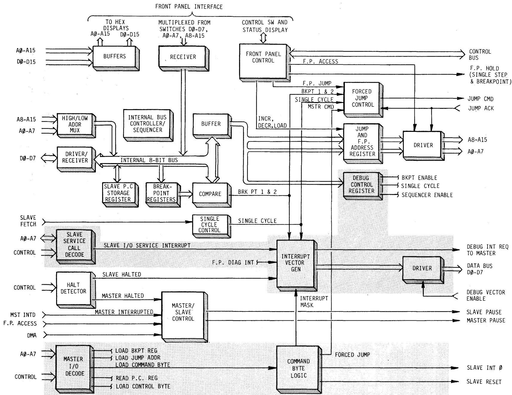
FIGURE 4-4 I/O COMMANDS AND INTERRUPTS
