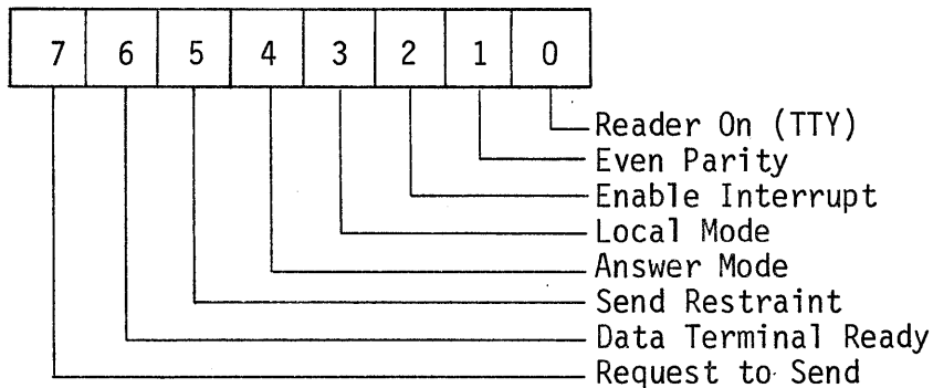
FIGURE 7-3 SERIAL PORT BYTE FORMATS
