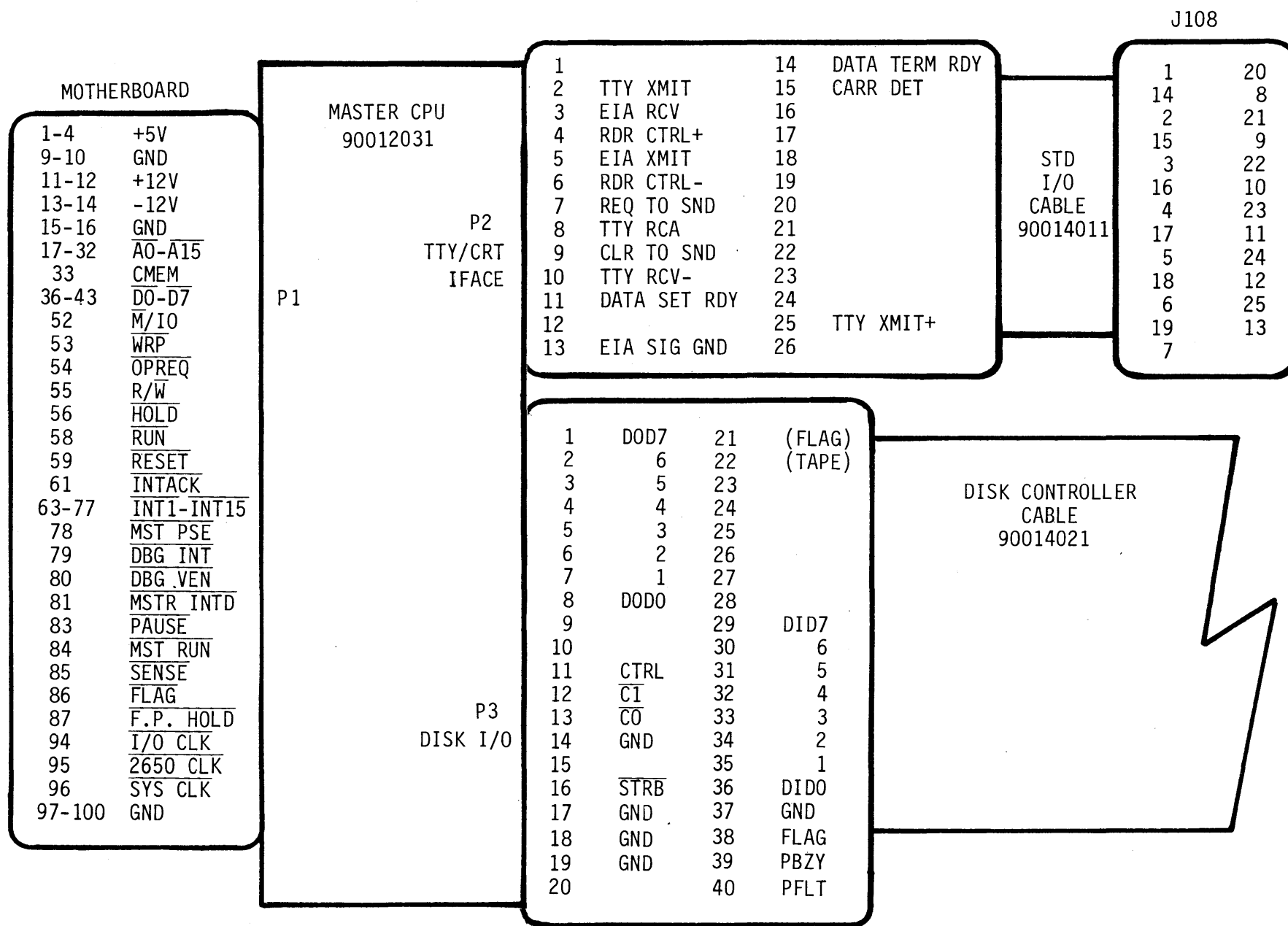
FIGURE 3-15 MASTER CPU INTERCONNECT
