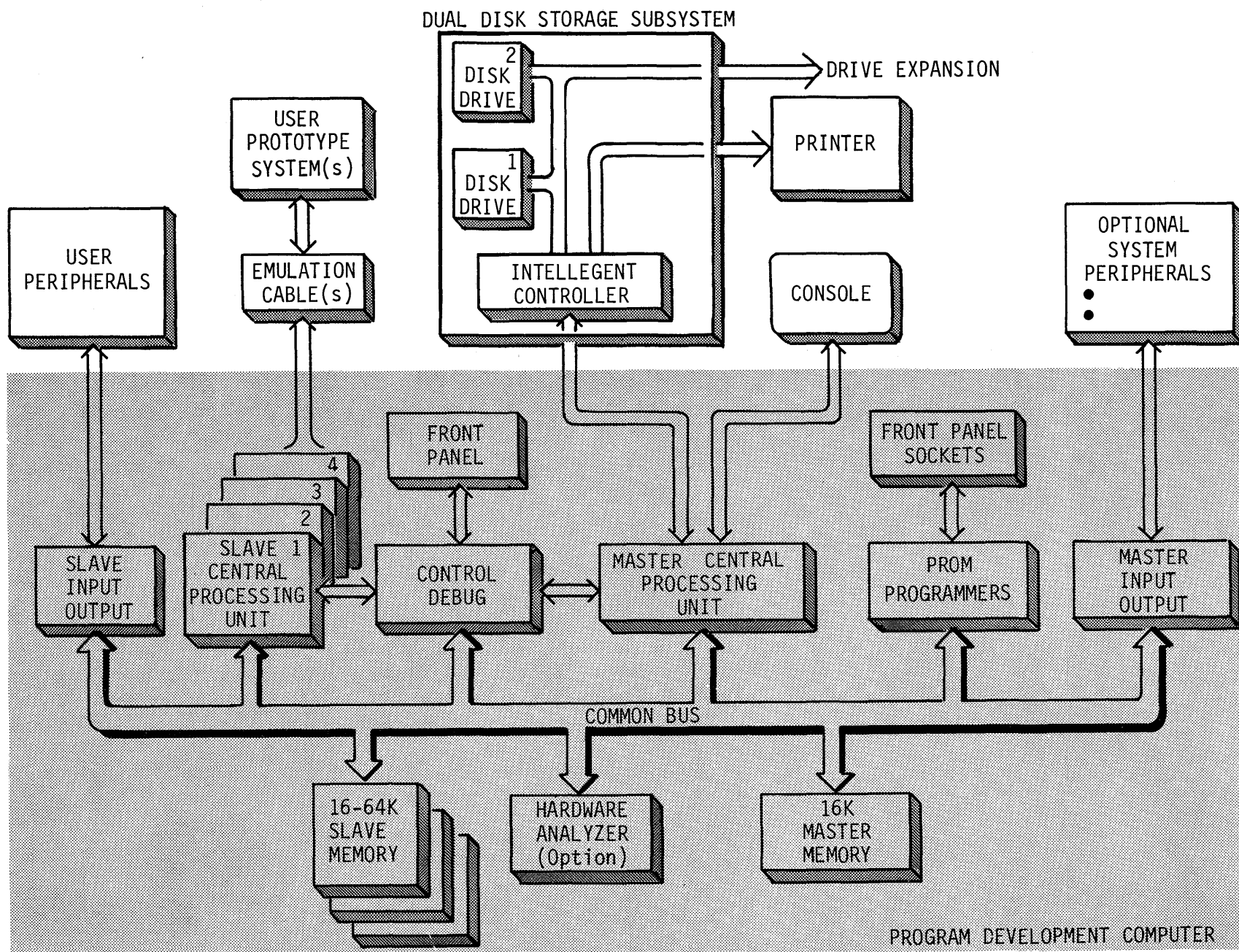
FIGURE 1-1 THE UNIVERSAL ONE SYSTEM
