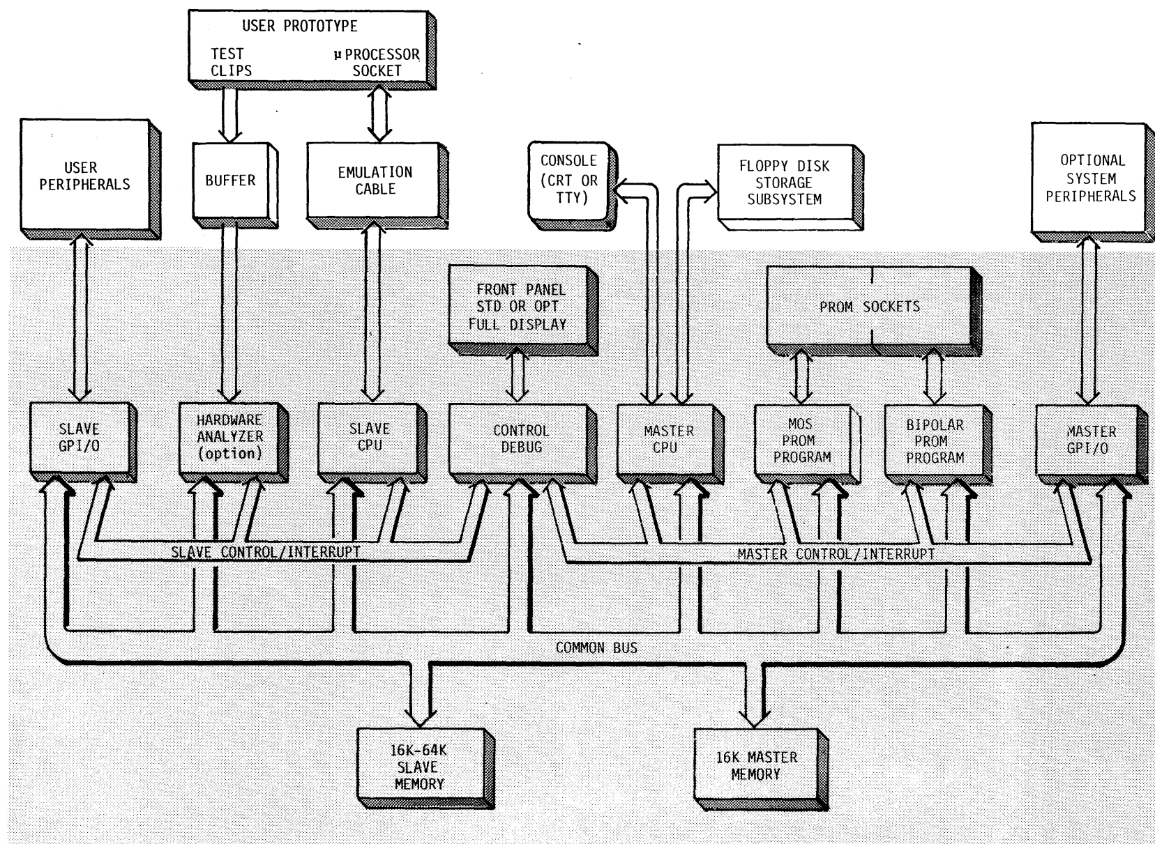
FIGURE 2-1 UNIVERSAL ONE SYSTEM BLOCK DIAGRAM
