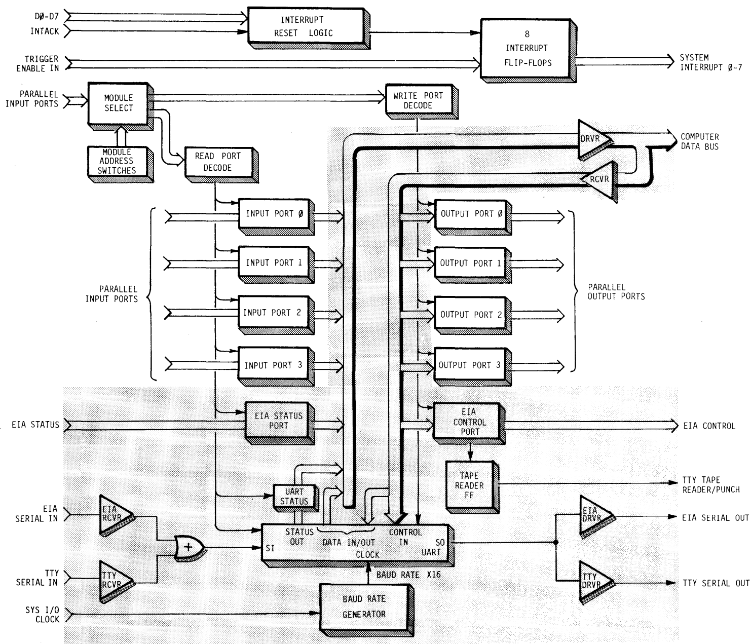
FIGURE 7-2 SERIAL I/O PORTS
