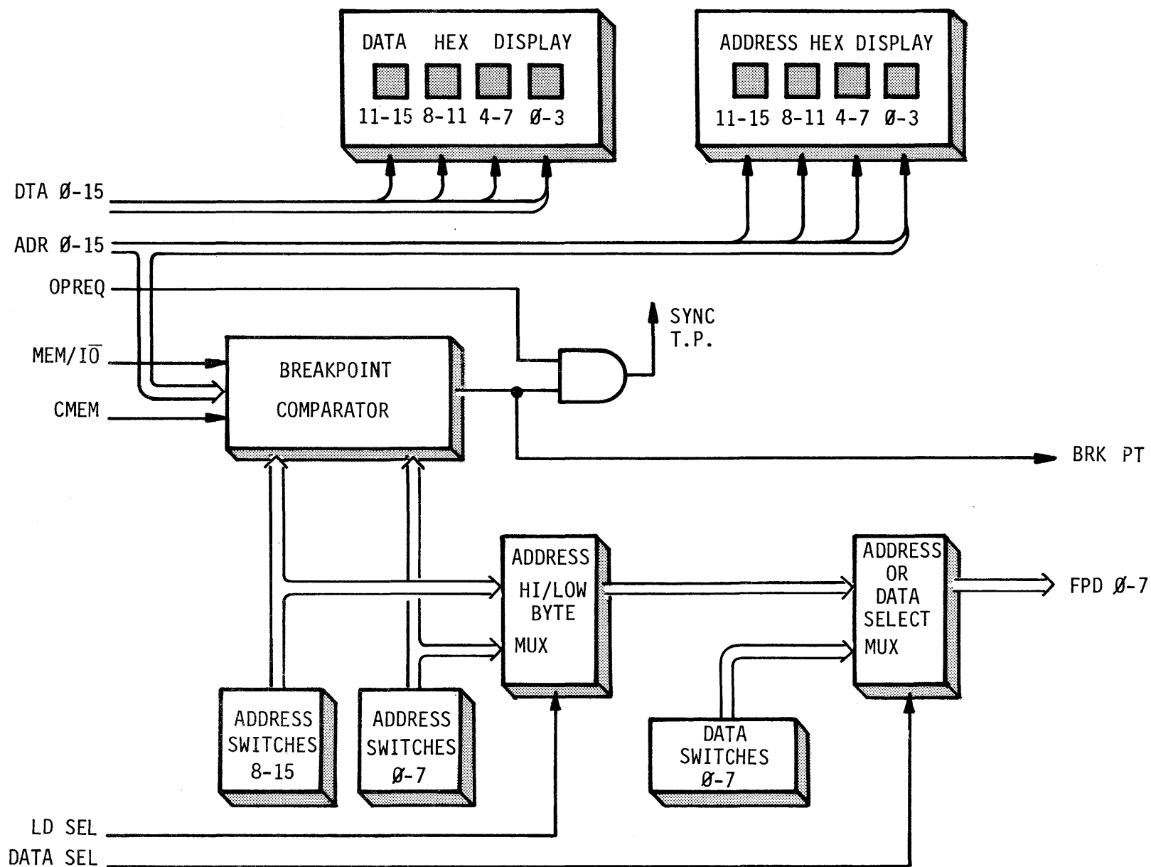
FIGURE 10-3 DATA AND ADDRESS LOGIC DETAILED BLOCK DIAGRAM
