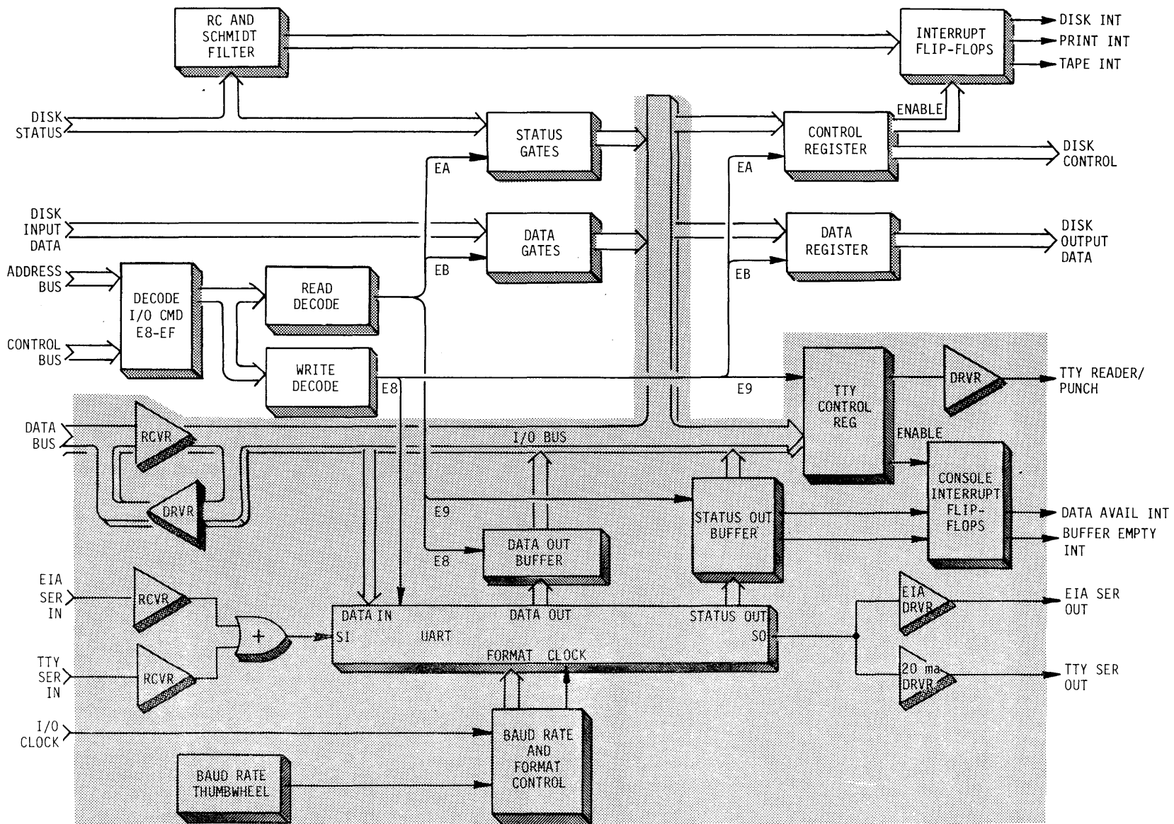
FIGURE 3-5 MASTER CPU CONSOLE I/O
