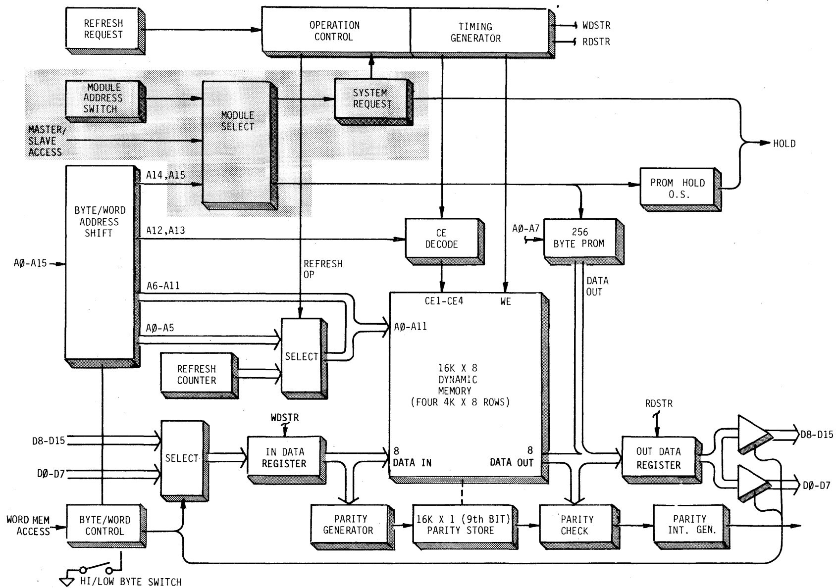
FIGURE 6-4 MODULE SELECT AND SYSTEM REQUEST LOGIC
