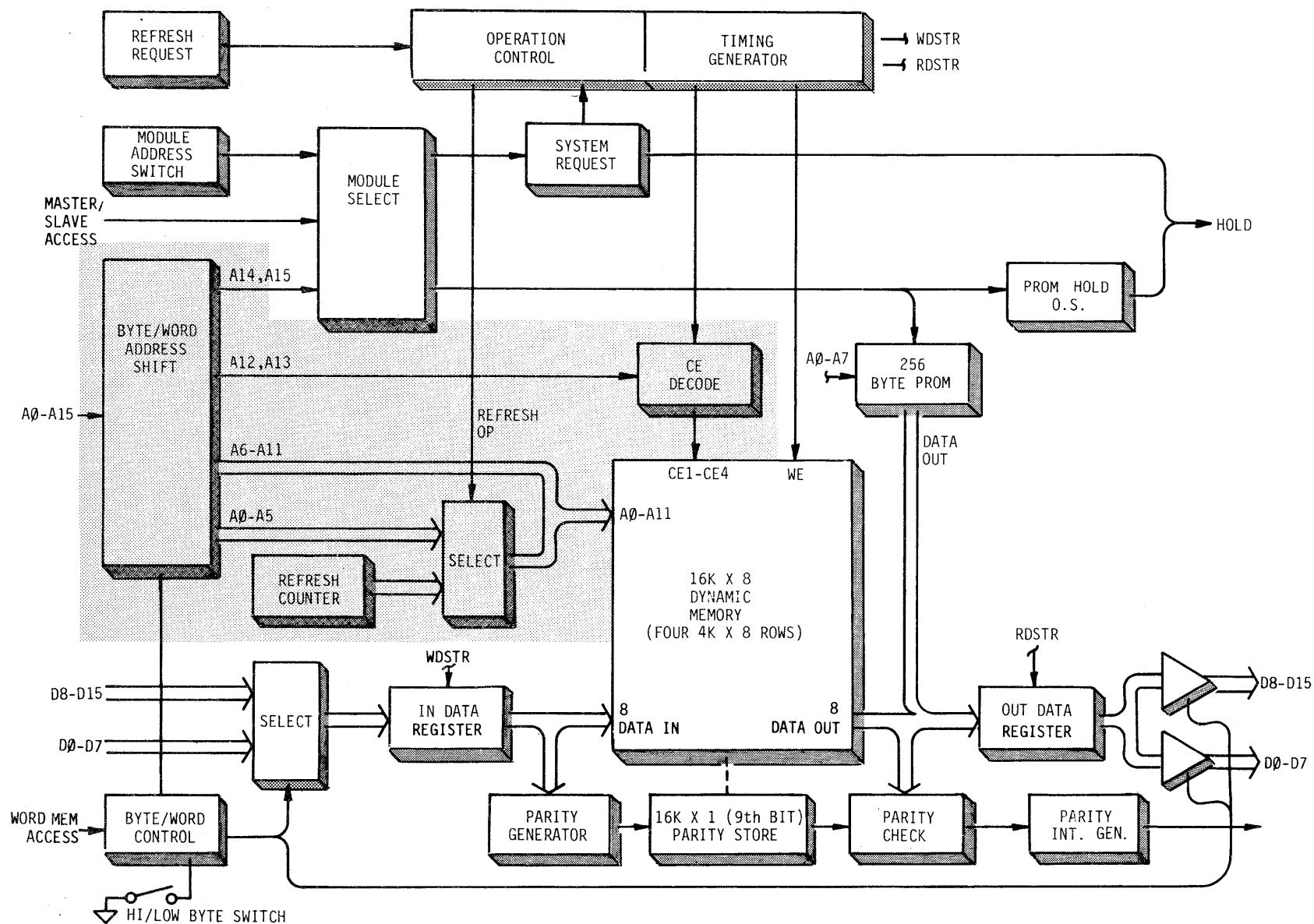
FIGURE 6-7 ADDRESS CONTROL
