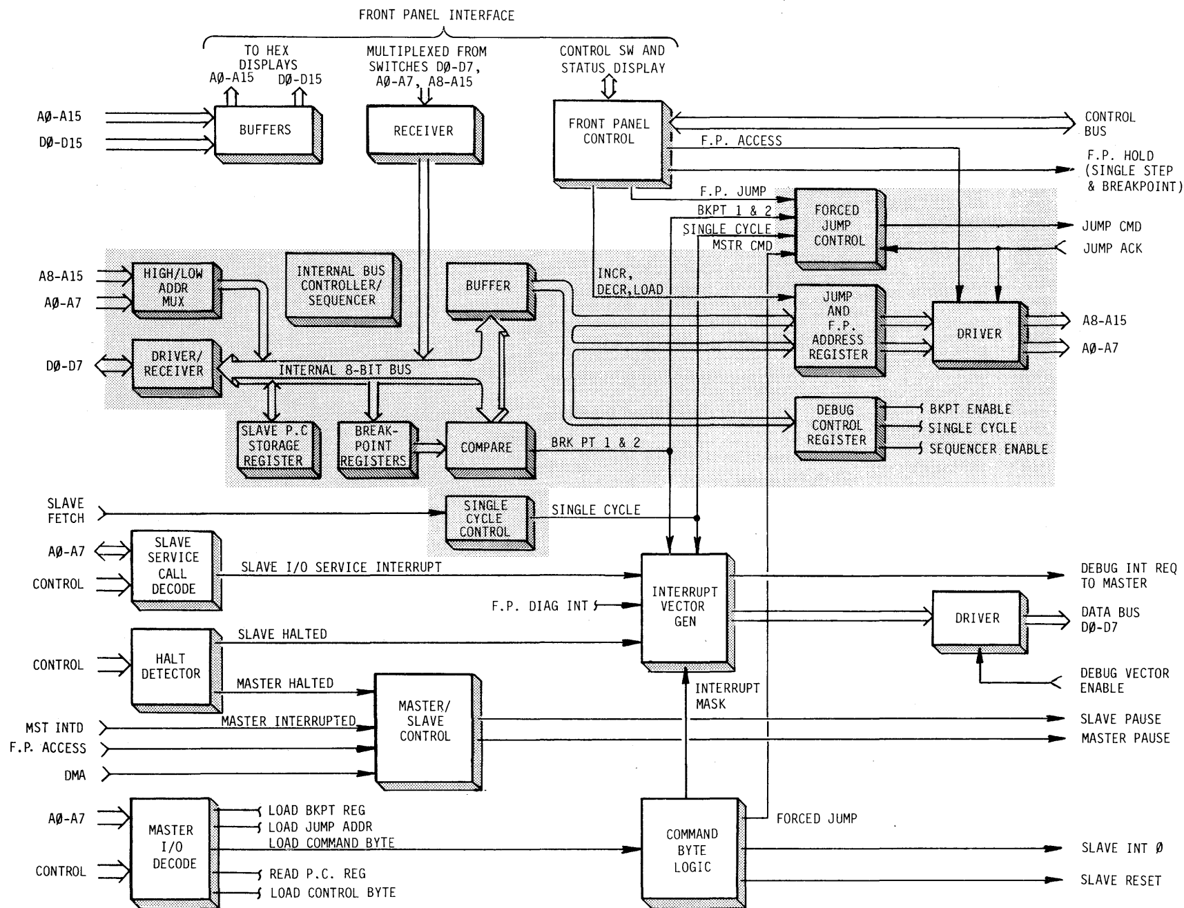
FIGURE 4-3 DEBUG LOGIC
