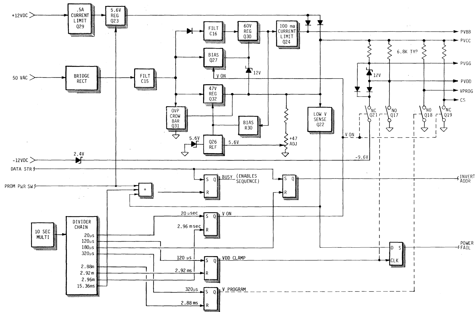
FIGURE 8-5 1702A PROM PROGRAMMER WRITE WAVEFORM GENERATOR DETAILED BLOCK DIAGRAM
