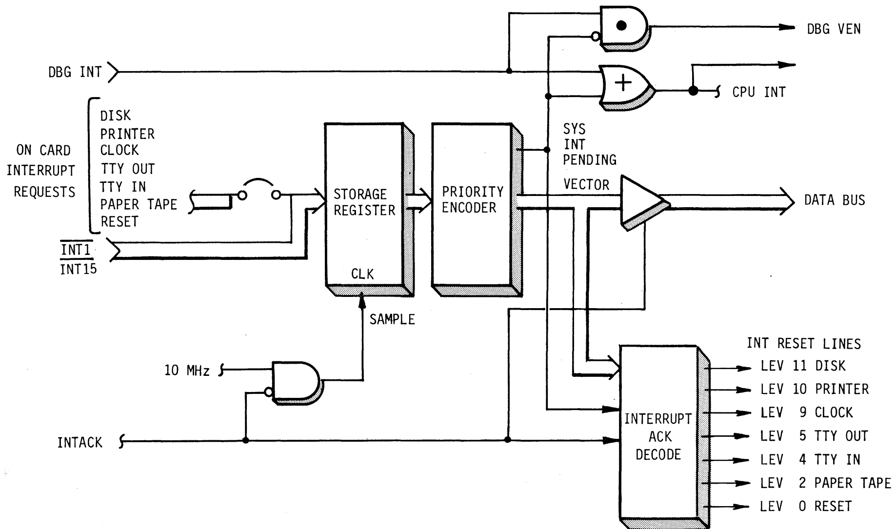
FIGURE 3-10 MASTER CPU INTERRUPT LOGIC
