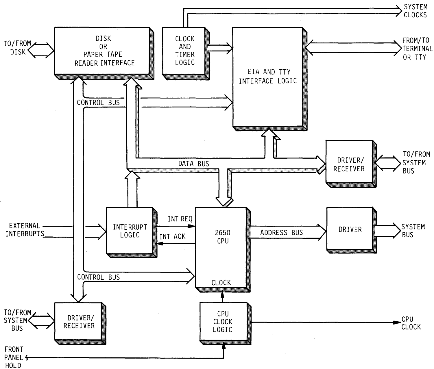
FIGURE 3-1 MASTER CPU BLOCK DIAGRAM
