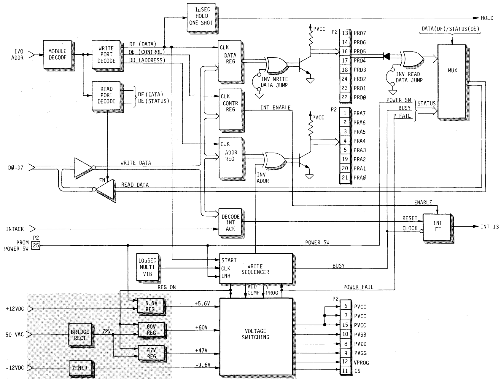
FIGURE 8-4 1702A PROM PROGRAMMER BLOCK DIAGRAM
