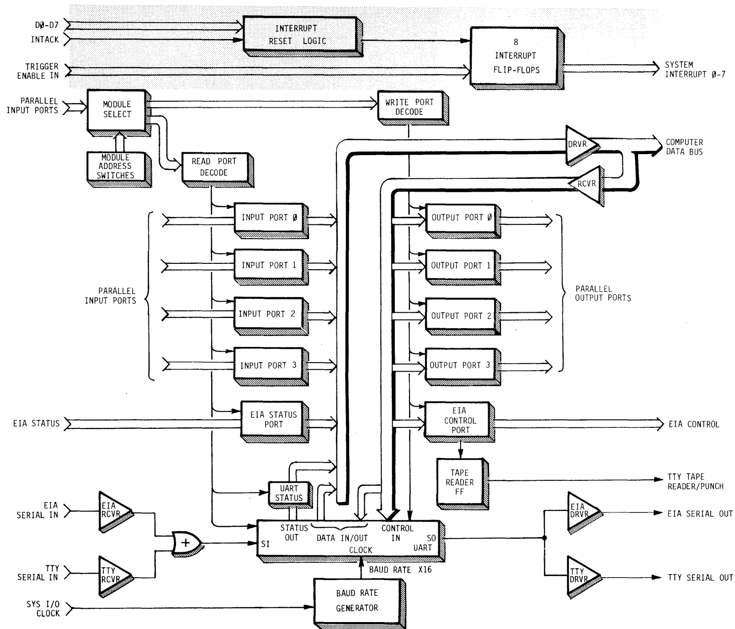
FIGURE 7-6 INTERRUPT LOGIC
