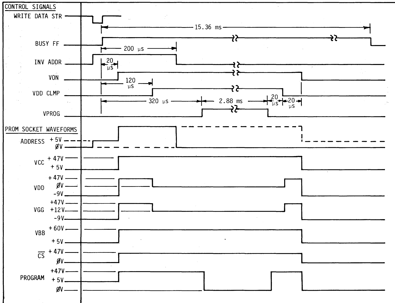
FIGURE 8-6 1702A SEQUENCER TIMING
