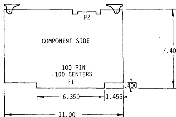
FIGURE 8-14 82S115 PROM PROGRAMMER ENVIRONMENTAL, POWER AND PHYSICAL REQUIREMENTS
