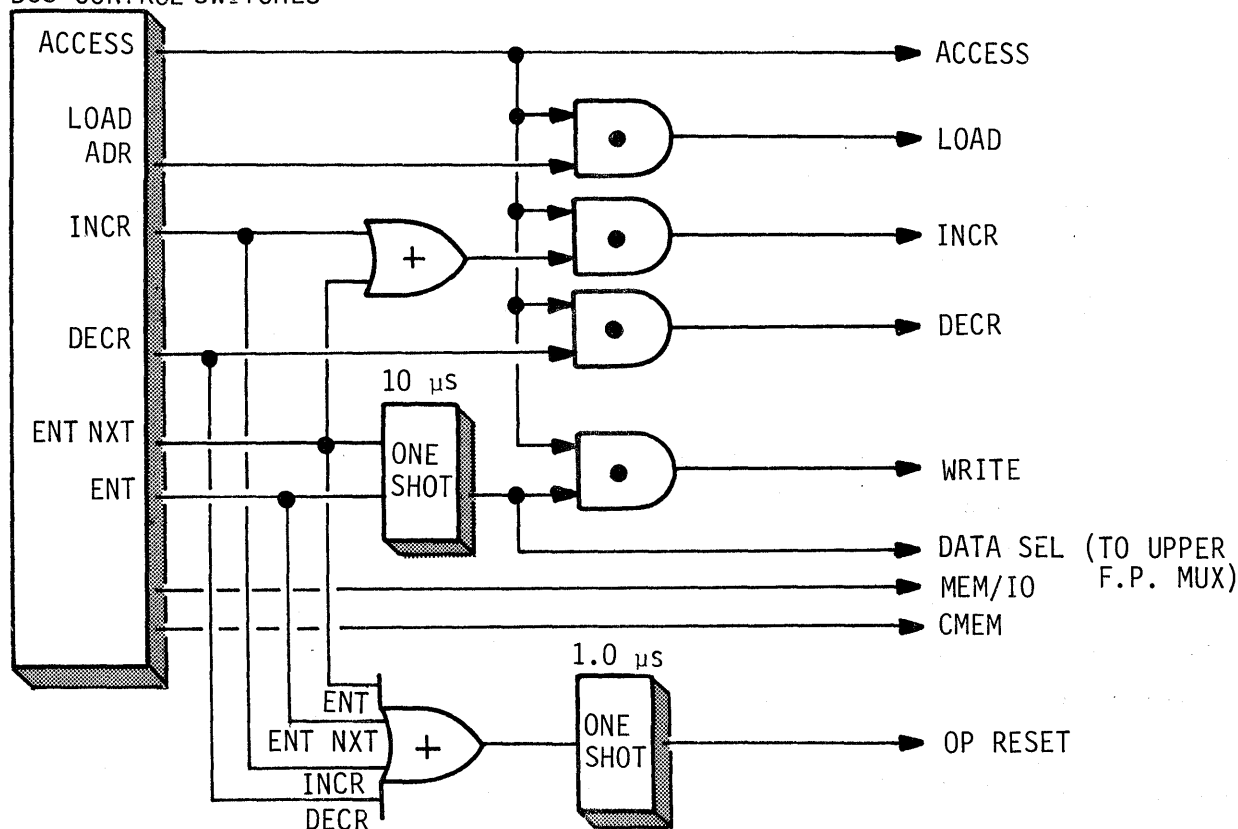
FIGURE 10-4 BUS ACCESS LOGIC
