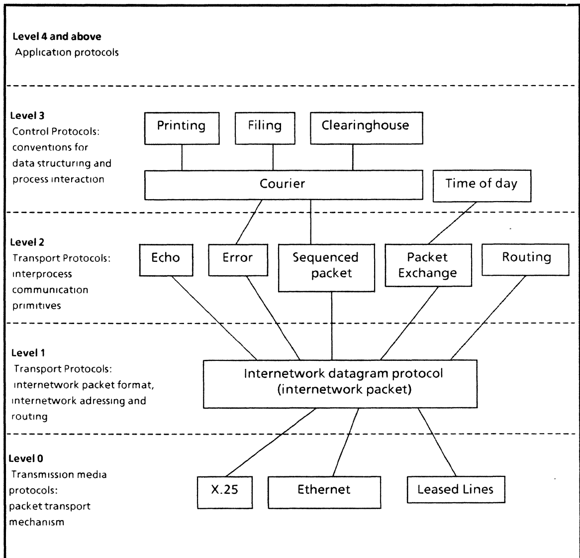
Figure 2.4 XNS Protocols
