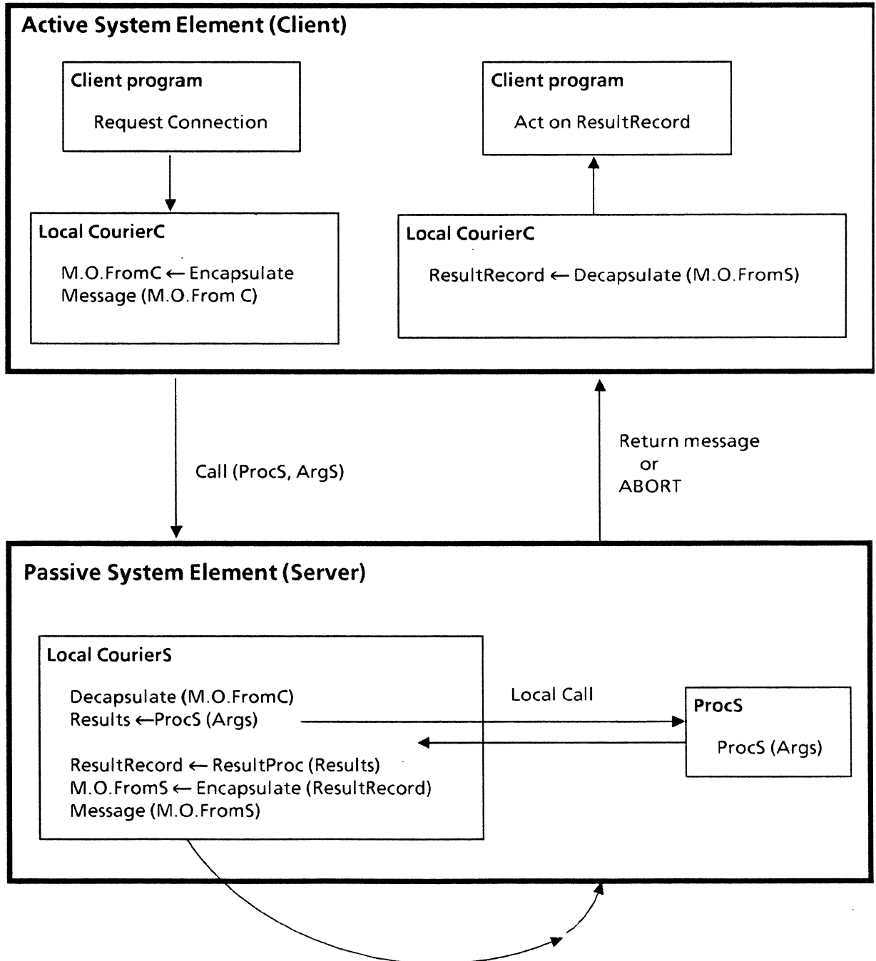
Figure 2.2 Courier Model
