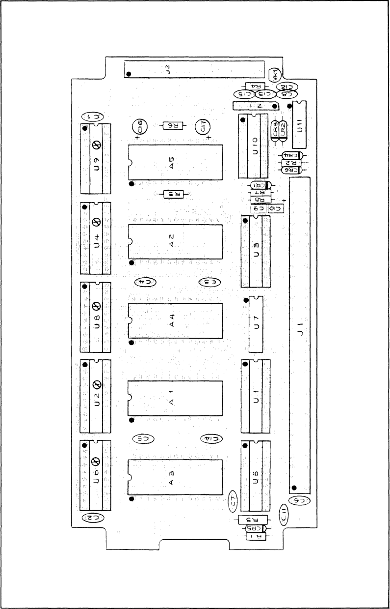
Figure 5-1. Interface PCB, Non-Component Side
