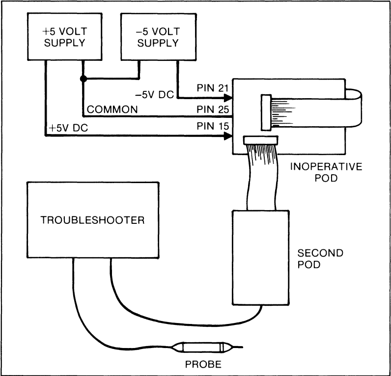
Figure 5-3. Troubleshooting an Inoperative Pod
