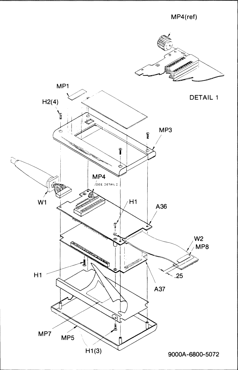
Figure 6-1 Final Assembly - 9000A - 6800 Pod
