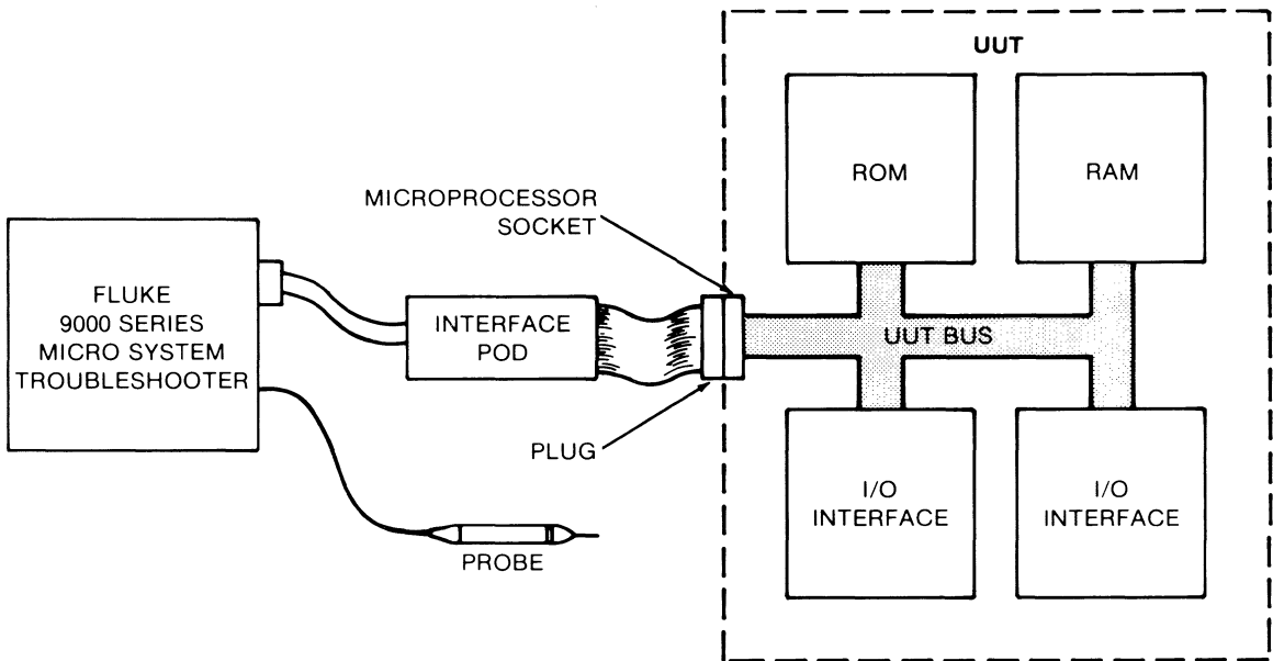
Figure 1-1. Relationship of Interface Pod
