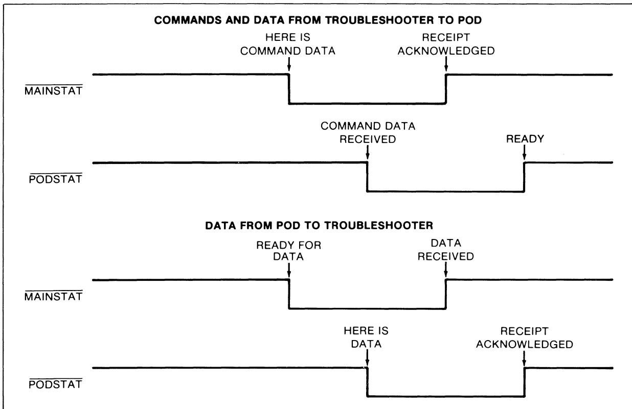
Figure 4-3. Handshaking Signals
