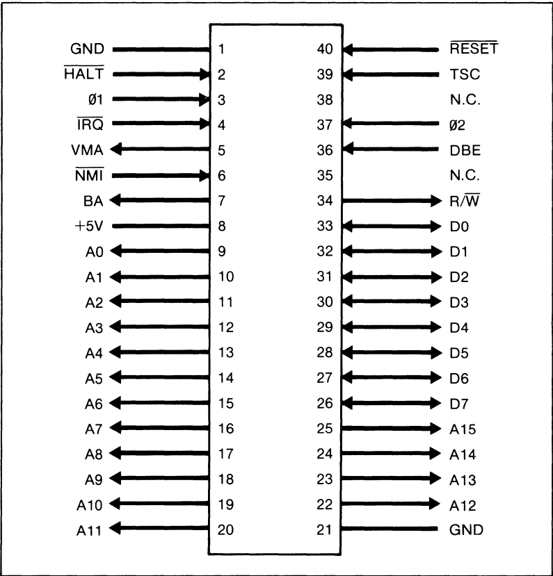
Figure 3-1. 6800 Pin Assignments
