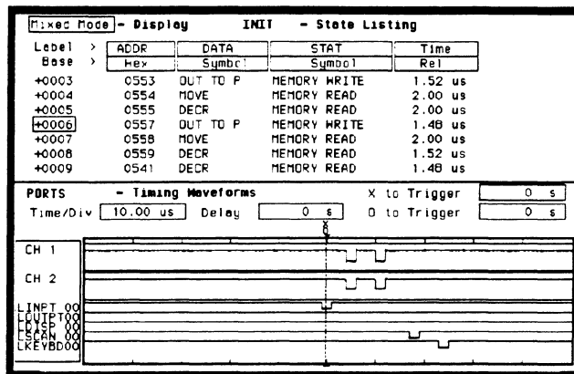
Figure 26-9. State/Timing/Scope Mixed Mode Display
