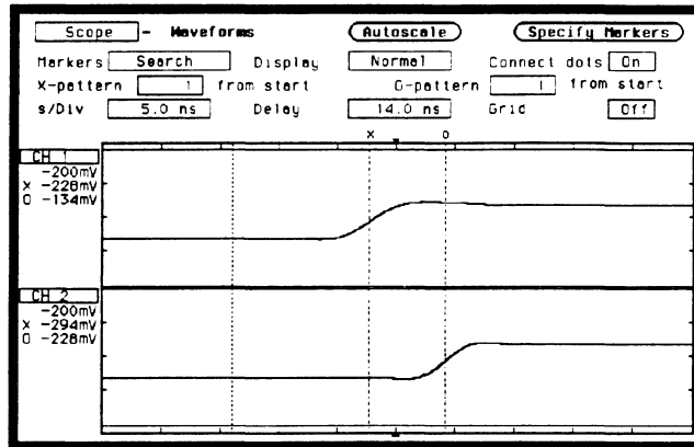
Figure 25-26. Waveform Display
