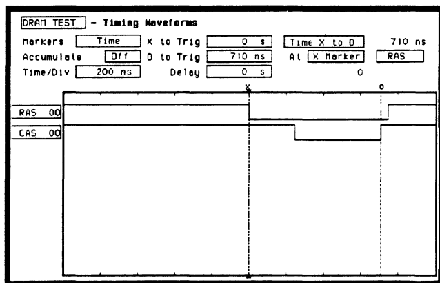
Figure 20-11. Marker Placement
