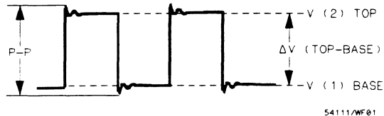
Figure 25-14. Top And Base Levels
