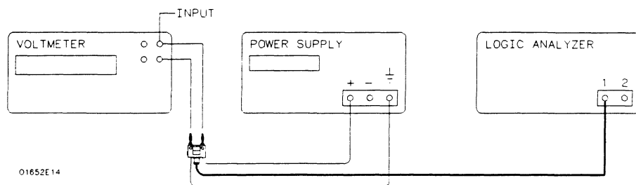
Figure D-7. Attenuator Calibration Equipment Setup
