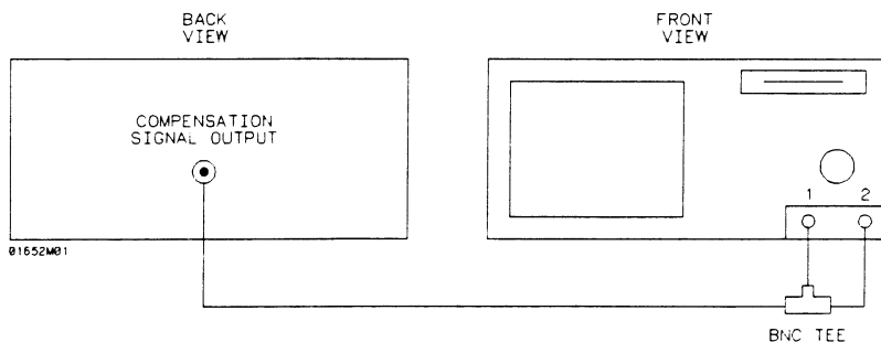
Figure 23-7. Compensation Signal Hookup
