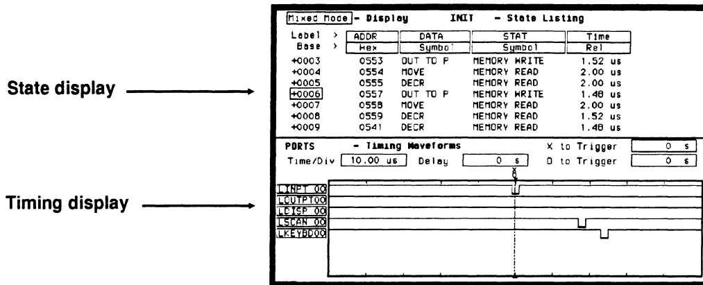
Figure 26-2. Timing/State Mixed Mode Display
