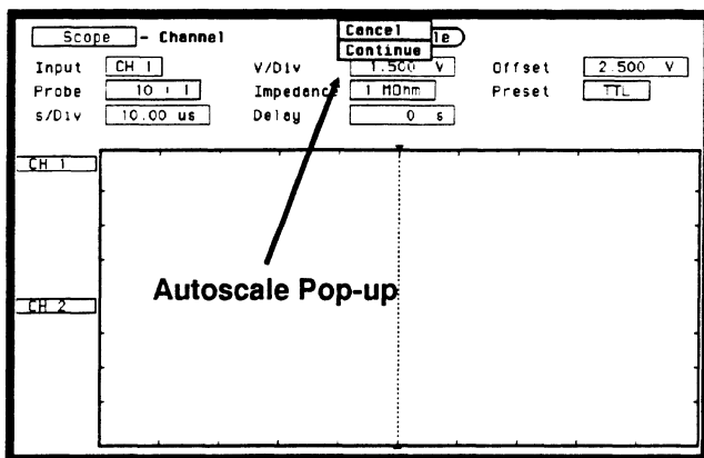
Figure 23-18. Autoscale Pop-up
