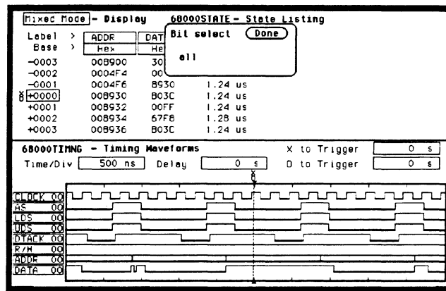
Figure 21-12. Overlapping Timing Waveforms
