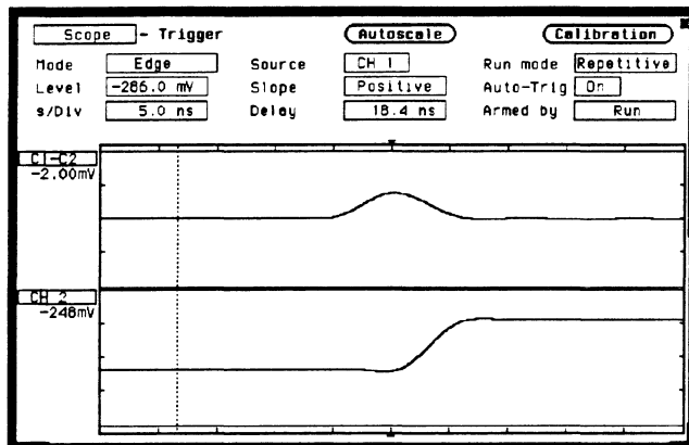
Figure 23-13. C1-C2 Waveform Display
