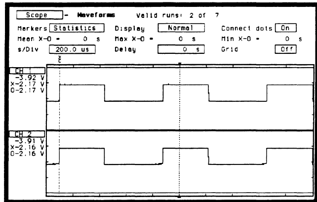
Figure 25-19. Statistics Fields
