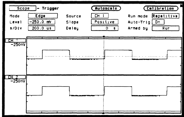
Figure 25-4. Autoscaled Waveform
