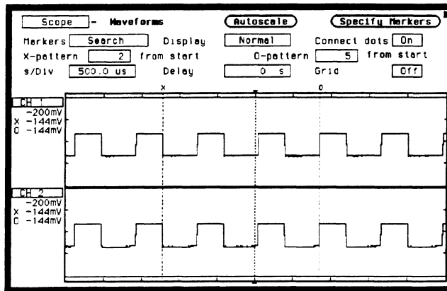
Figure 25-23. Search Marker Measurement Waveform
