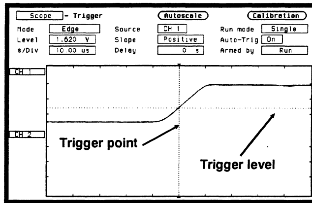
Figure 24-2. Trigger Point
