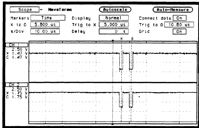
Figure 27-13. Scope Waveforms Display
