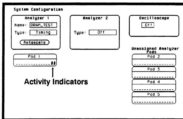
Figure 20-3. Activity Indicators
