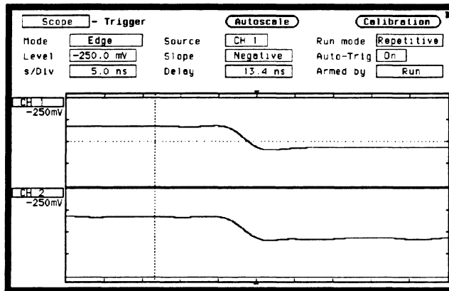
Figure 25-6. Negative Edge Of Waveform
