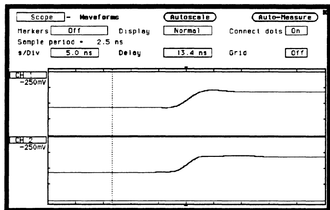
Figure 25-5. Expanded Waveform
