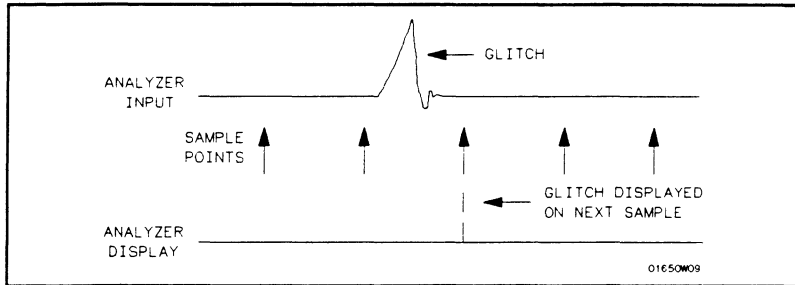
Figure 18-5. Glitch in Timing Waveform
