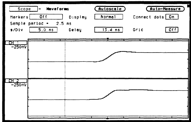
Figure 25-8. Rising Edge on Waveform
