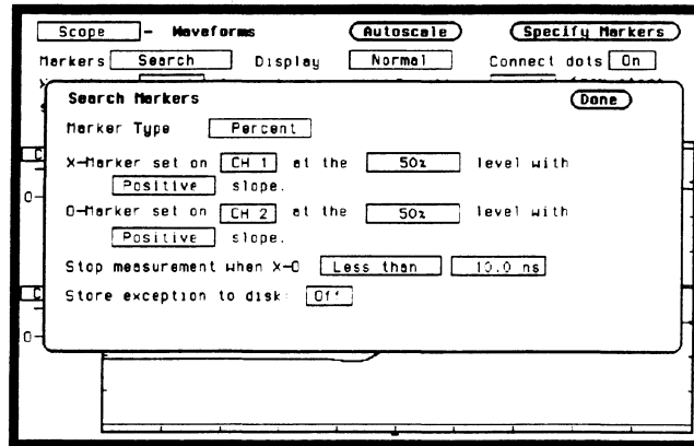
Figure 25-25. Stop Measurement Less than Setup
