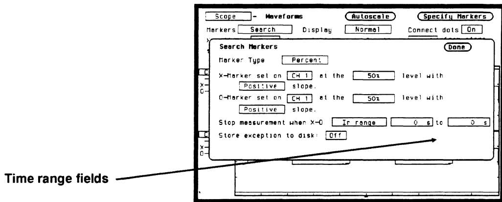
Figure 25-18. Range Fields
