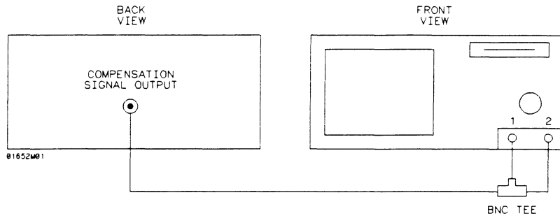
Figure 25-3. Equipment Setup
